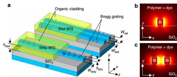
Figure 1.21 Silicon organic hybrid laser concept. (a) Light is guided by SOI strip or slot waveguides consisting of thin silicon nanowires (width w_{strip} \approx 150\text{--}500\text{nm} , height h_{WG} \approx 200\text{--}350\text{nm} ). Optical gain is provided by a fluorescent organic cladding material (thickness h_{clad} \approx 500 \pm 50\text{nm} ). (b) Dominant electric field component ( E_x ) of the fundamental quasi-TE mode for a narrow strip. (c) Dominant electric field component ( E_x ) of the fundamental quasi-TE mode for a slot waveguide [81].
