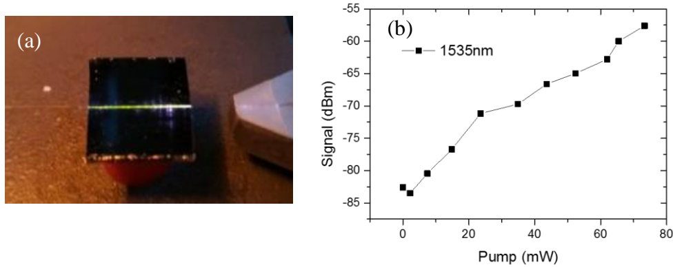
Figure 3.23 Gain measurements of polymer waveguide (a), light injection and (b) signal evolution as function of the pump power.
