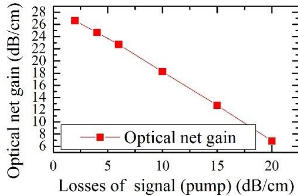
Figure 3.29 Simulated optical gain in 1-centimeter-long hybrid slot waveguides with slot width 220nm according to the spectroscopy parameters in Table.3.8.
