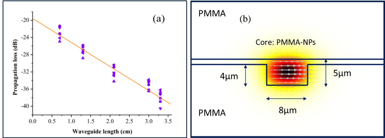
Figure 3.20 (a) Linear propagation losses as a function of waveguide length. The derivative loss level obtained from linear fitting is 5.3 \pm 0.3 \text{ dB/cm} at wavelength \sim 1535 \text{ nm} . (b) Waveguide geometry of the Er NPs PMMA waveguides and the electric field E_x confinement of TE mode at wavelength \sim 1535 \text{ nm} .
