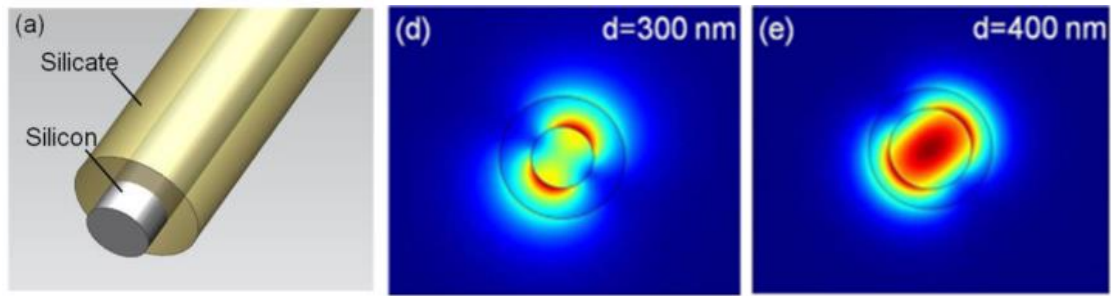
Figure 1.19 (a) Schematic of the core-shell nano- structure. (d) (e), optical electrical-field distribution images for HE11 mode with core diameters of 300 nm, 400 nm [114].
