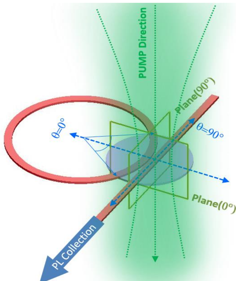
Figure 4.15 Schematic graph of polarization of the pump beam with \theta angle regarding to the resonator coupler. The two 0^\circ -plane and 90^\circ - plane represent the nanotube axis plane or projection plane, respectively. Green beam is to shown the pump incidence and its possible polarizations, depicted with blue arrows. The violet disk represents the CNT layer. The PL was collected from the bus waveguide by using lensed fibers.
