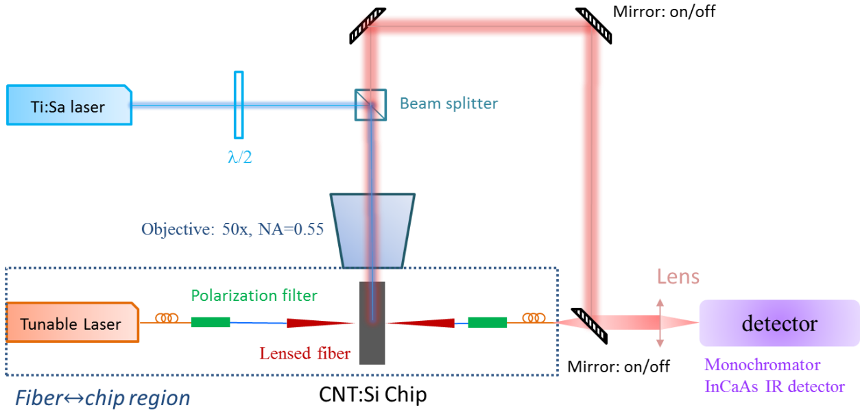
Figure 4.11 Schematic graph of the optical setup that was used to characterize the CNT PL coupling with silicon ring resonators. Fiber to Chip region were adopted to collect PL from the waveguides for section 4.3. The free space PL collection method was used to study the CNT interaction with nanobeam cavities in section 4.4.
