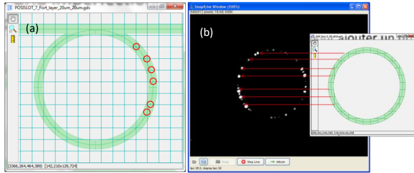
Figure 2.11 (a) Subfields of the slot ring resonator gds , where the red circles or equivalent places are the risky regions giving rise to stitching errors; (b) captured scattering losses of slot waveguides from near infrared camera (from the top, at \lambda=1.55\mu\text{m} , when injecting light in-plane from an input SOI strip).
