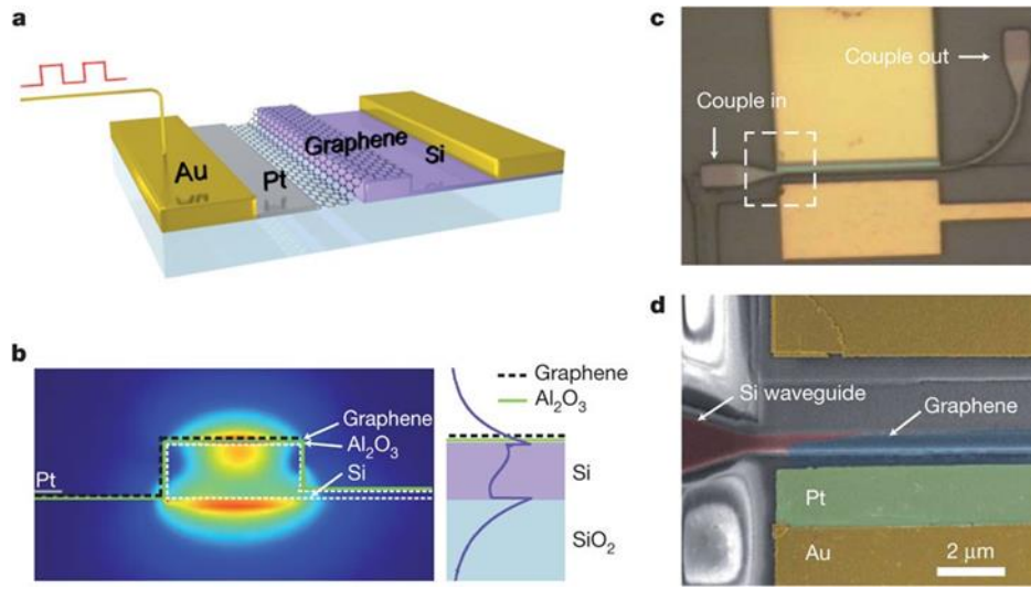
Figure 1.17 (a) Three-dimensional schematic illustration of a device based on a graphene sheet placed on top of a silicon bus waveguide, separated from it by a 7-nm-thick \text{Al}_2\text{O}_3 layer (not shown). (b) Left, cross-section of the device, with an overlay of the optical mode plot, calculated by finite element simulation. (c,d) Top view of the whole device [51].
