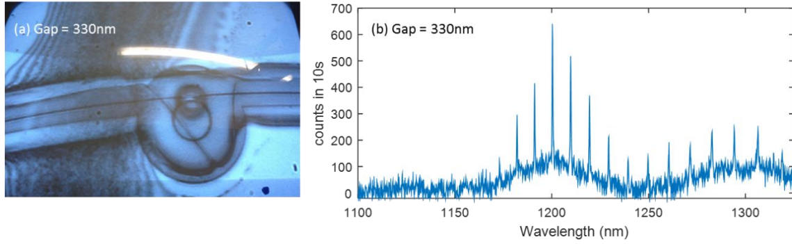
Figure 4.21 (a) Optical view of the ring resonator with PFO-CNT ribbon deviating far from the ring resonator center. (b) Collected photon counts from ring resonator in (a).
