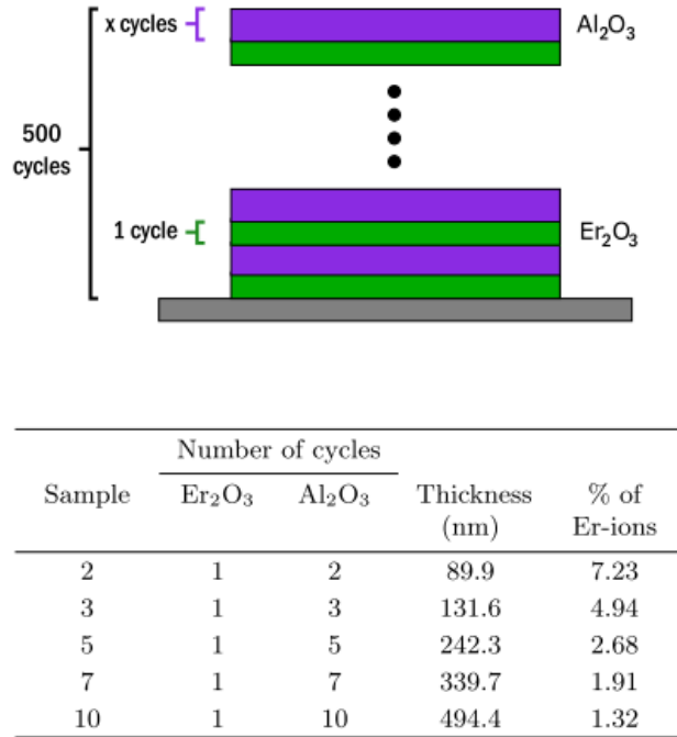
Figure 3.24 The tested samples are composed of 500 periods (cycles), as shown on the left. Five different samples were fabricated with different numbers of Al_2O_3 cycles between each two Er_2O_3 layers. The ratios of the number of the Er_2O_3 and Al_2O_3 cycles are shown on the left. The total thickness and Er ion ratios are also summarized. [210]
