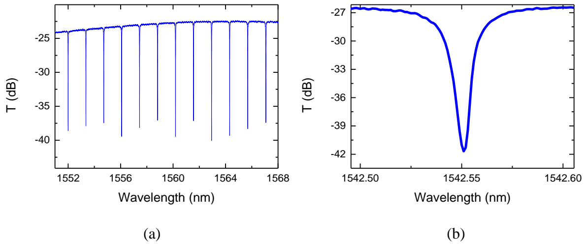
Figure 2.26 Linear Transmission spectrum of 70 \mu m diameter silicon ring resonator with width of 600nm; (b) Q -factor and extinction ratio (ER) of the resonance peak @ 1.542 \mu m extracted are Q =81,000 and 15dB for TE polarization.
