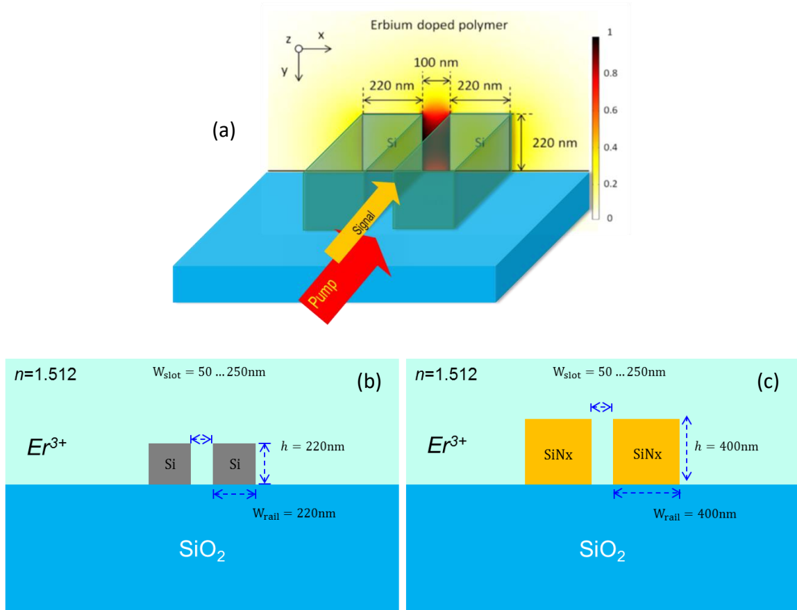
Figure 3.6: (a) Normalized electric field energy of the cross section of silicon slot waveguides filled by \text{Er}^{3+} -doped materials for 1530 nm wavelength signal amplification. The slot waveguide cross-sections are considered with different slot sizes both for the silicon (b) and silicon nitride (c) waveguide cases.
