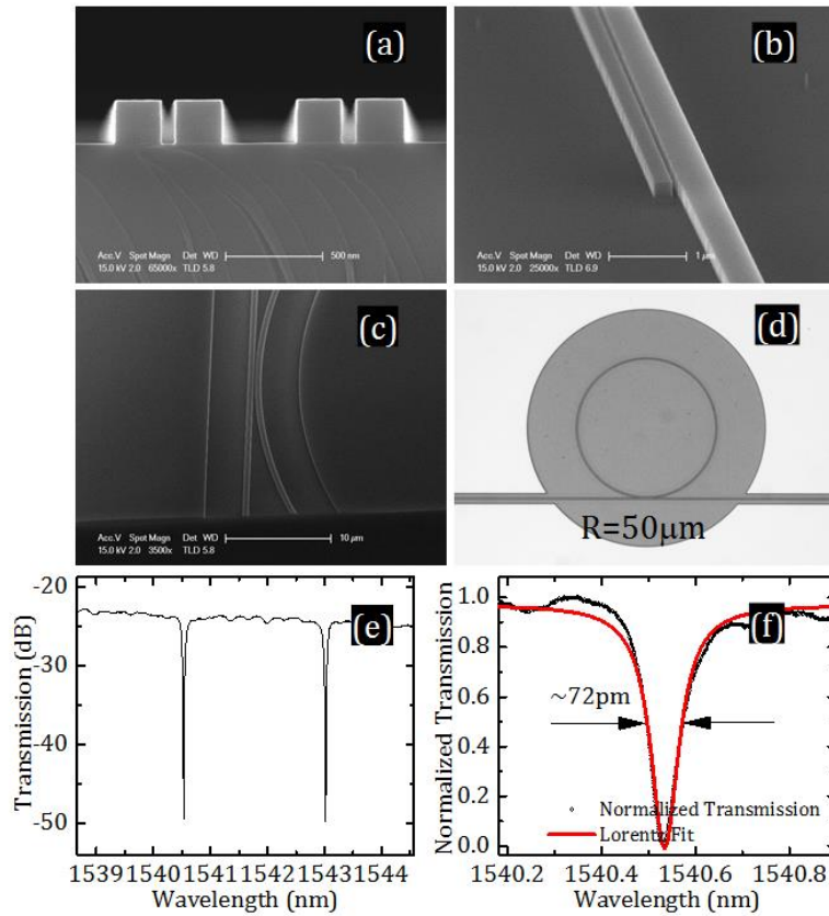
Figure 2.27 Cross-section of ring coupler with a coupling gap here of 310 \pm 10 \text{ nm} ; (b). Mode converter used to couple light from strip waveguide to slot waveguide; (c). View of the straight bus-ring coupler region; (d). Optical overview of a fabricated slotted all pass ring resonator (APR); (e-f). Normalized transmission spectrum of slotted APR with coupler gap of 500nm with a Lorentzian fitting curve.
