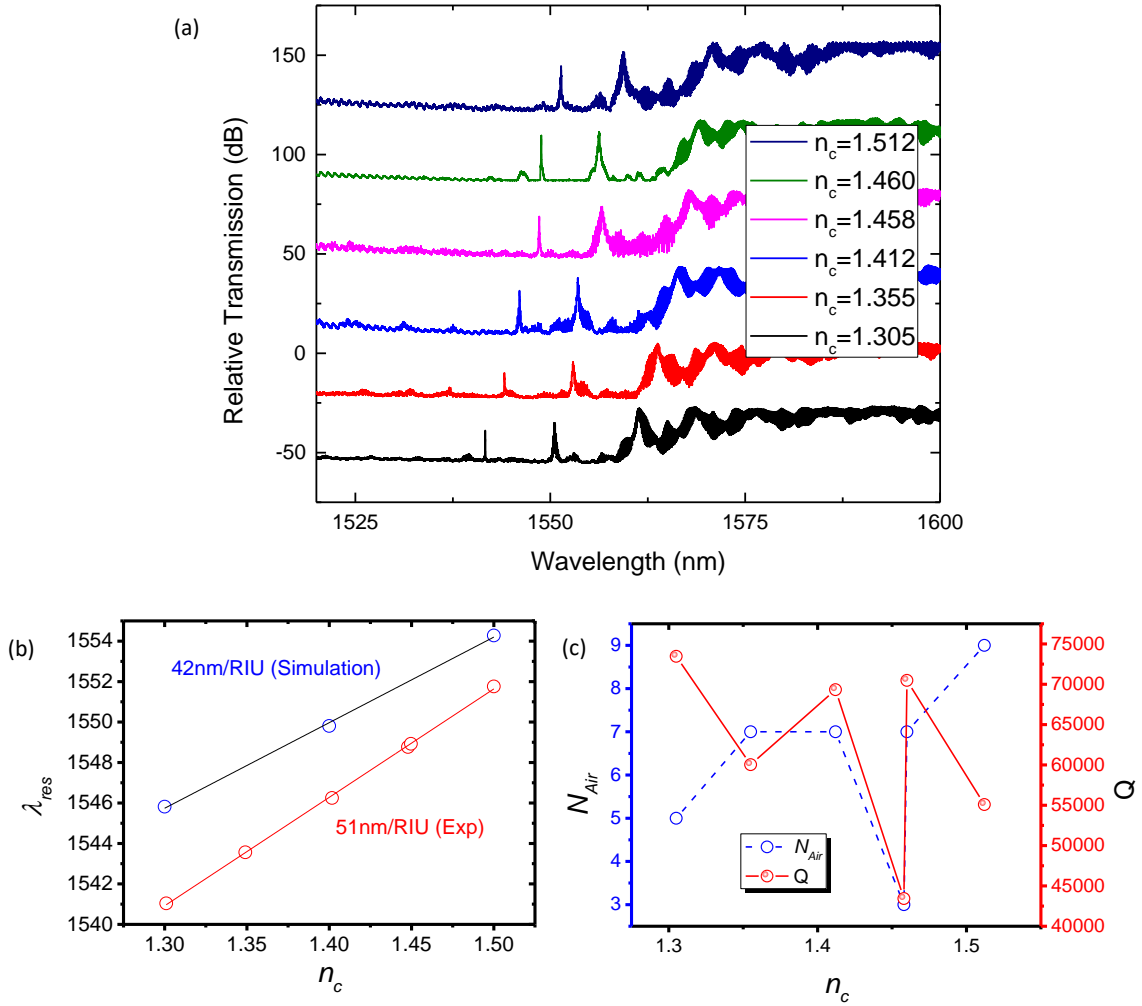
Figure 2.39 (a), Resonance wavelength shift as a function of the cladding RI. (b), simulated and experimental sensitivity of the first cavity I-mode. (c) Measured max Q -factor of the I-mode resonance as a function of the cladding RI.
