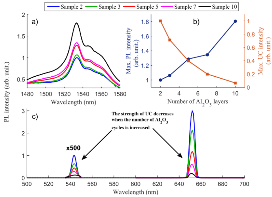
Figure 3.25 (a) PL-spectra of the Samples at the wavelength range 1480-1580 nm;(b) Maximum PL signal as a function of the number of \text{Al}_2\text{O}_3 layers between each \text{Er}_2\text{O}_3 layer in the Samples and (c) Up-conversion spectra of the fabricated samples in the 500 - 700 nm wavelength range with \lambda_{exc}=980\text{nm} . [210].
