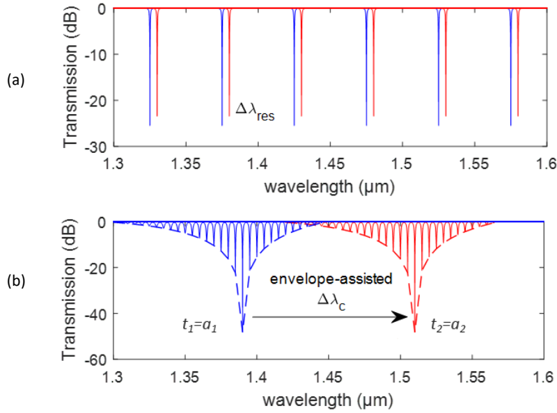
Figure 2.32 Schematic explanation of the sensing mechanism normally used by tracking one specific resonance \lambda_{\text{res}} (a) and the one that we propose by tracking the critical coupling resonance through the spectrum envelope monitoring (b).
