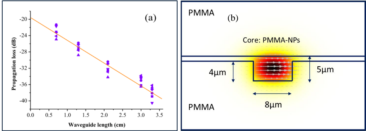
Figure 3.20 (a) Linear propagation losses as a function of waveguide length. The derivate loss level obtained from linear fitting is 5.3 \pm 0.3 \text{ dB/cm} at wavelength \sim 1535 \text{ nm} . (b) Waveguide geometry of the Er NPs PMMA waveguides and the electric field E_x confinement of TE mode at wavelength \sim 1535 \text{ nm} .
