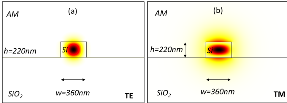
Figure 2.2 Cross-sectional view of power confinement of typical SOI strip waveguides at \lambda=1.55\mu\text{m} : (a) TE polarization; (b) TM polarization.
