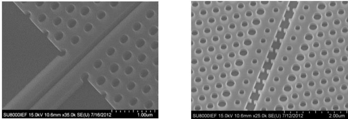
Figure 1.12 Slow light 2D photonic crystal waveguide platform. (left), Slotted photonic crystal waveguides, (right) corrugated and dispersion engineered slot photonic crystal waveguides. [91]
