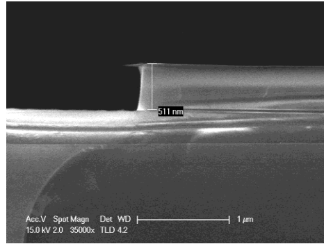
Figure 2.16 500nm thick ZEP520 has been spin coated on silicon nitride wafer
