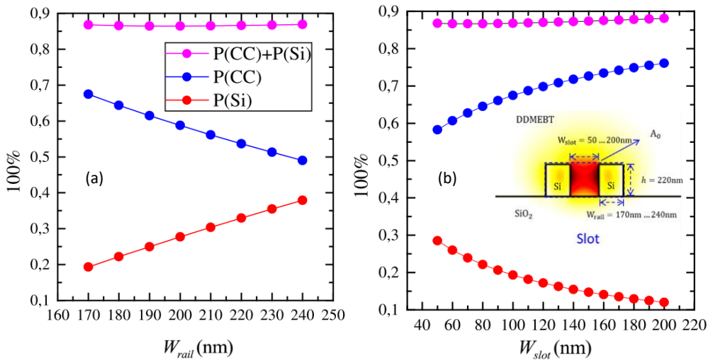
Figure 2.6 Optical power confinement in silicon rails (Si), top cladding (CC) and above BOX (CC+Si); (a) when considering slot width =100nm; (b) when considering rail widths of 170nm width ( \lambda=1.55\mu\text{m} ). The top cladding is envisioned as nonlinear polymer DDMEBT with refractive index 1.8.
