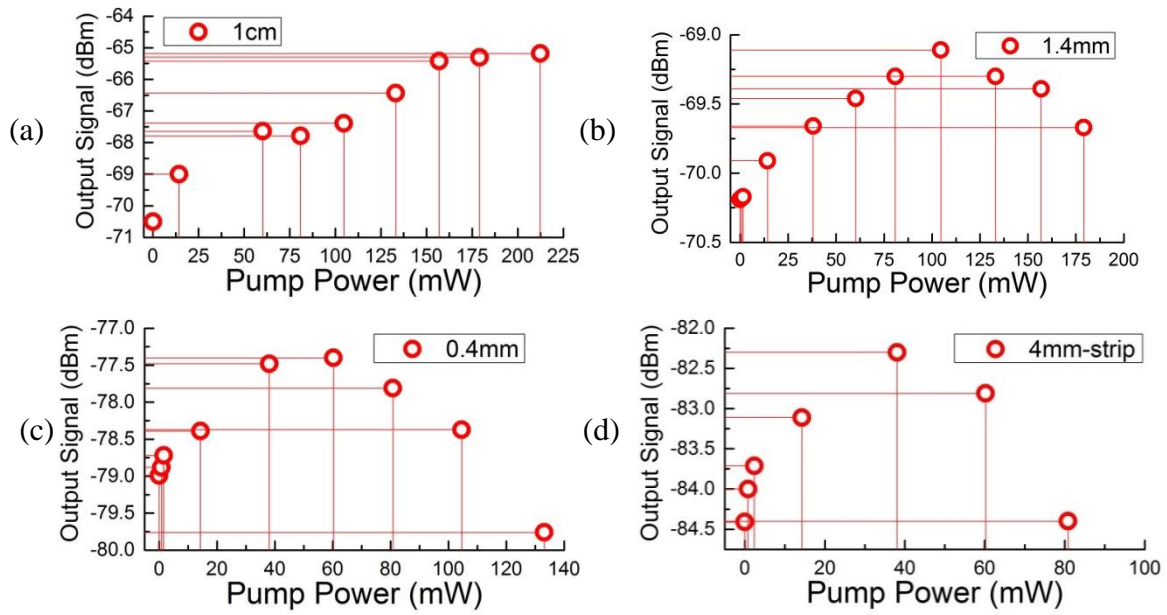
Figure 3.31 Relative gain of three different slot waveguides with 220nm slot width, one strip waveguide with 550nm width; A maximum relative gain 5.32dB, 1.08dB, 1.59dB, 2.3dB are measured, respectively.
