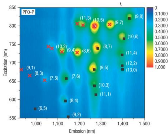
Figure 4.3 Photoluminescence excitation spectroscopy (PLE) map of SWNTs in toluene solution, in which polymer polyfluorene (PFO) were used to selectively solubilize some specific carbon nanotube species. Red cross means n-m=3q-1 and black square corresponds to n-3=3q+1 . [221]
