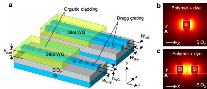
Figure 1.21 Silicon organic hybrid laser concept. (a) Light is guided by SOI strip or slot waveguides consisting of thin silicon nanowires (width w_{\text{strip}} \approx 150\text{--}500\text{nm} , height h_{\text{WG}} \approx 200\text{--}350\text{nm} ). Optical gain is provided by a fluorescent organic cladding material (thickness h_{\text{clad}} \approx 500 \pm 50\text{nm} ). (b) Dominant electric field component ( E_x ) of the fundamental quasi-TE mode for a narrow strip. (c) Dominant electric field component ( E_x ) of the fundamental quasi-TE mode for a slot waveguide [81].
