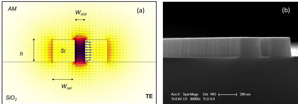
Figure 1.10 (a) Electrical field E of the fundamental TE mode of a typical silicon slot waveguide with a waveguide height h=220nm , rail width W_{rail}=220nm and slot width W_{slot}=100nm . The active material was assumed to have the same refractive index as SiO_2 . The considered wavelength is 1.55\mu m . (b) An example of fabricated slot waveguides (in C2N/Orsay, former IEF laboratory, Orsay).
