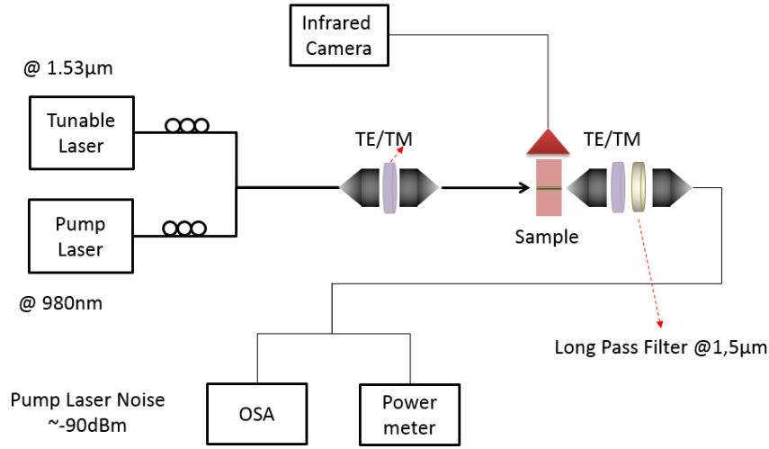
Figure 3.22 Schematic figure of the optical setup that we used to measure the signal gain ( 1.53\mu\text{m} ) by pumping with 980nm laser source.
