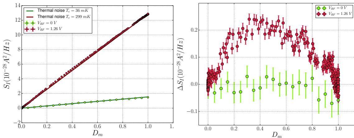
Figure 5.5: (Left) Measured noise as a function of mean transmission D_m , without RF pulsing (green dots) and with RF pulsing (red dots). Parameters are : V_{RF} = 1.26 \text{ V} , \nu = 6.15 \text{ GHz} , \Delta\varphi = \pi , no magnetic field. The solid lines represents the thermal noise: S_I^{th.} = 4k_B T \frac{2e^2}{h} D_m at 36 mK (green line) and 299 mK (red line). A deviation appears for RF pulsing between experimental points and adiabatic limit, that corresponds to the QS noise. (Right) Excess noise as a function of mean transmission D_m , without RF pulsing (green dots) and with RF pulsing (red dots). RF pulsing adds an excess noise in addition to the thermal noise.
