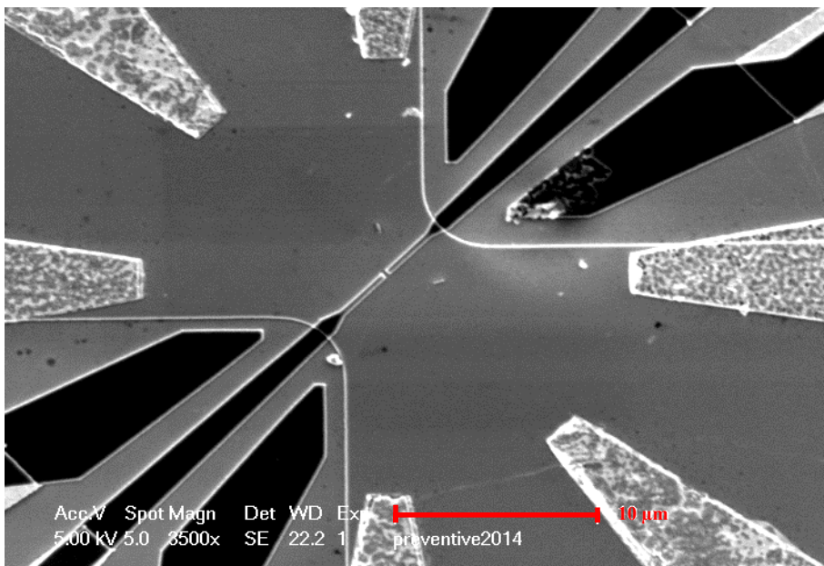
Figure 2.13: SEM image of the gates of sample 2. Black color correspond to aluminium. 300 \times 300 nm square shape of the gate is visible.
