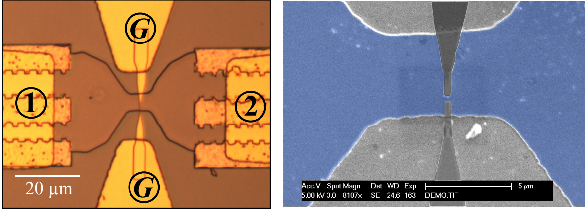
Figure 2.10: ( Left ) Optical picture of the mesa of sample sample 1, recognizable with its hourglass shape presented in figure 2.3. The coplanar waveguides indexed by 1 and 2 (resp. G) are connected to the two ohmic contacts (resp. to the gate). ( Right ) SEM picture with artificial colors of the gates of sample 1.
