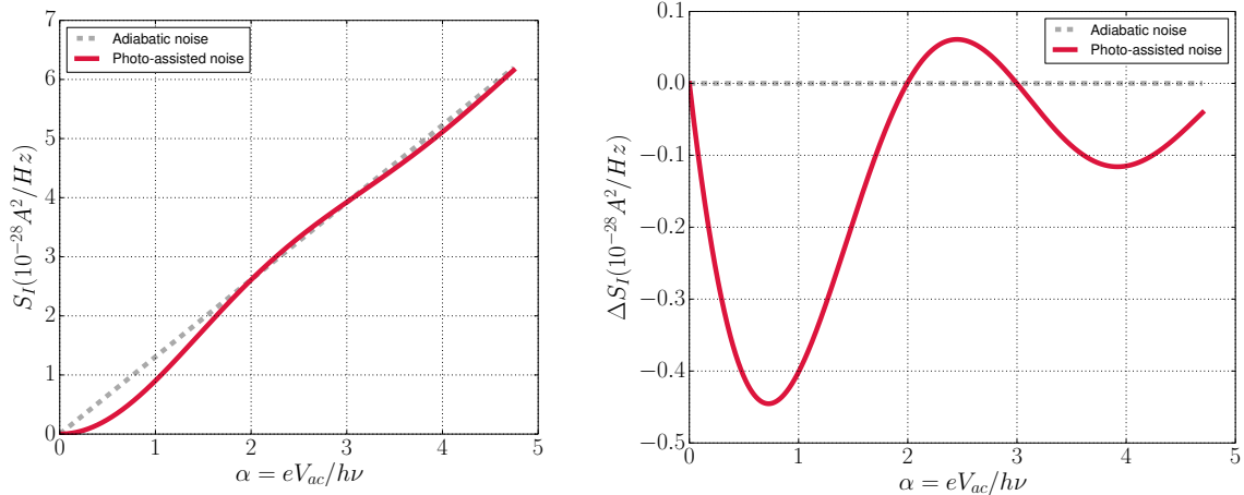
Figure 1.10: ( Left ) Photo-assisted shot-noise (red solid line) versus the reduced amplitude \alpha = eV_{ac}/h\nu , for V_{dc} = 0 . The classical modulation of DCSN represented by the grey dashed line is a pure linear function of V_{ac} . Parameters are : \nu = 18 GHz, T = 0 . ( Right ) Difference between the photo-assisted shot-noise and the classical noise versus the reduced amplitude \alpha , with the same parameters. The PASN exhibits clear oscillations as a function of \alpha .
