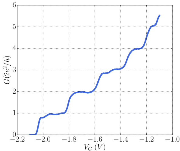
Figure 2.4: Experimental conductance of a 2-contacts QPC (sample 1) as a function of gate voltage V_G . The measurement is performed at 24 mK with no external magnetic field.
