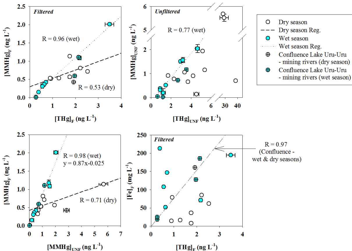
Figure 28 : Linear regressions for filtered (F) and unfiltered (UNF) total Hg (THg) vs. monomethylHg (MMHg) concentrations (upper 2 panels), filtered vs. unfiltered monomethylHg concentrations (lower left panel) and filtered iron (Fe) vs. total Hg (THg) concentrations (lower right panel) in surface waters collected along the Lake Uru-Uru transect (empty symbols) and downstream the confluence with mining effluents (crossed symbols) during the late dry season (white symbols) and the late wet season (blue symbols).
