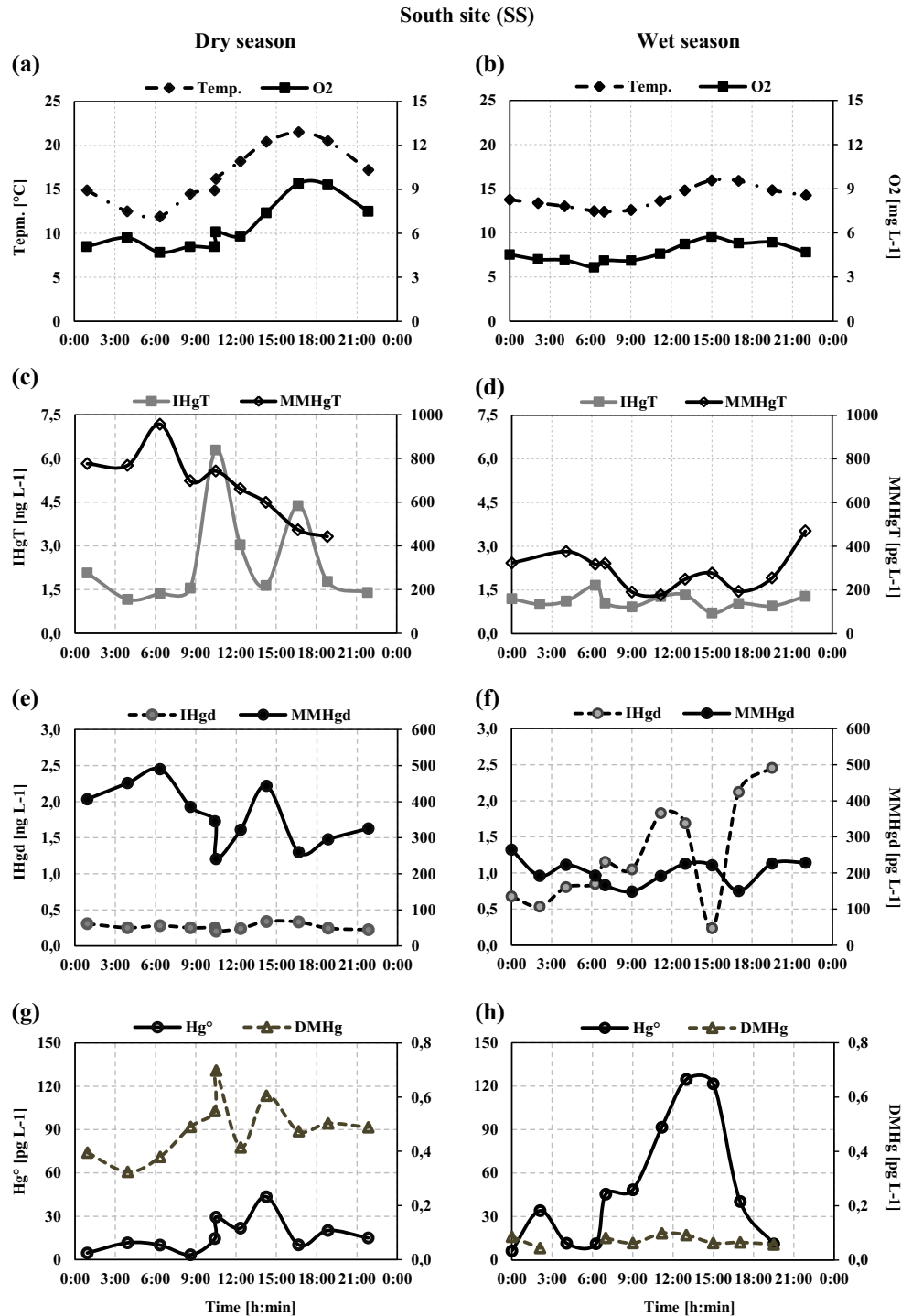
Fig. 2 a–h Diurnal variability (24 h) of the different Hg species (IHg T , IHg d , MMHg T , MMHg d , Hg 0 , DMHg) in comparison with oxygen and temperature at the southern site (SS) of Lake Uru Uru for late dry and wet seasons. T total, d dissolved
