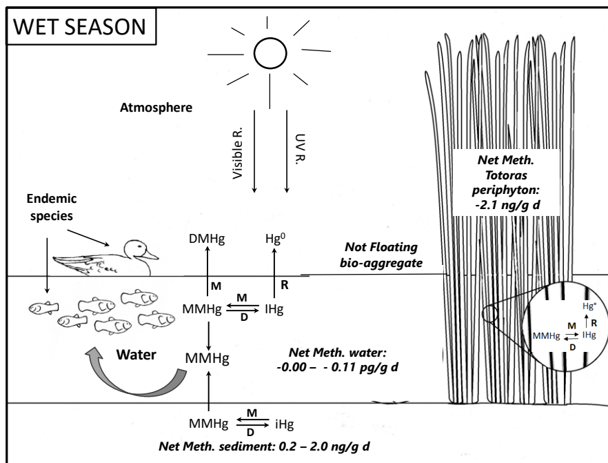
Figura 36: Schematic representation of the potential net methylation of Hg occurring in different compartments of Lake Uru-Uru for a dry season and b wet season. Net methylation are expressed in nanograms per gram per day in order to compare water, sediment, and bio-organic substrate incubation measurements.
