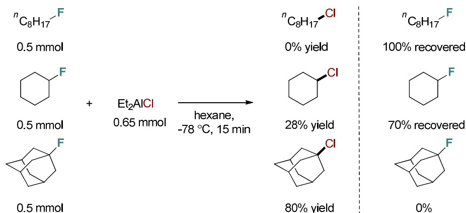
Scheme 5.3. Competition study between alkyl fluorides with AlEt_2Cl .
