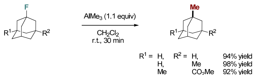
Scheme 5.4. Methylation of fluoroadamantanes with AlMe_3 .
