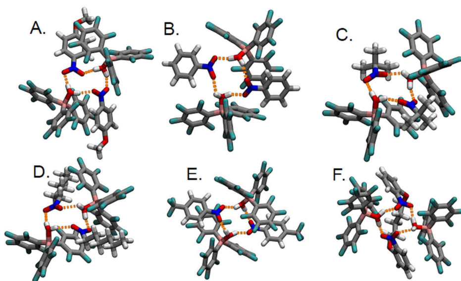
Figure 4.9. Initial results of computational modeling: w B97X-D/6-31G(d,p) DFT level of theory-optimized structures for the complexes of B(C_6F_5)_3 \cdot H_2O with: 4-nitroanisole (A), nitrobenzene (B), 2-methyl-2-nitropropane (C), 1-nitrohexane (D), 4-nitrobenzotrifluoride (E) bis-nitro compound 71 (F). H-white, C-grey, O-red, F-green, B-pink, N-blue
