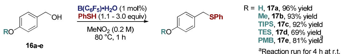
Scheme 2.6. B(C 6 F 5 ) 3 •H 2 O-catalyzed chemoselective benzylic alcohol activation in the presence of silyl ethers functionalities.
