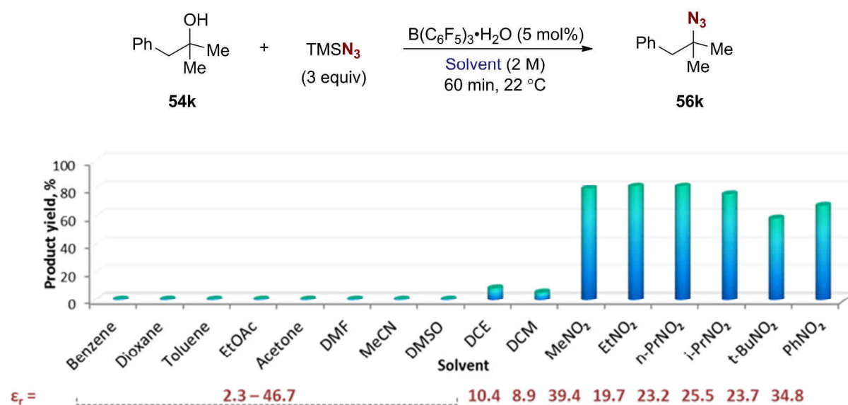
Figure 4.1. Solvent screen for azidation reaction (NMR yield).
