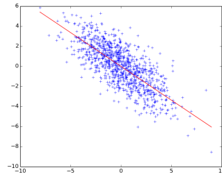
(b) \kappa = 2^{-1/2} : correlated case. The straight line is the theoretical optimal regression line (i.e. the line with equation y = ax where a minimizes the variance of Y - aX , computed thanks to the asymptotic formulas (1.16) and (1.17)): one can notice that it fits well with the empirical datas.
