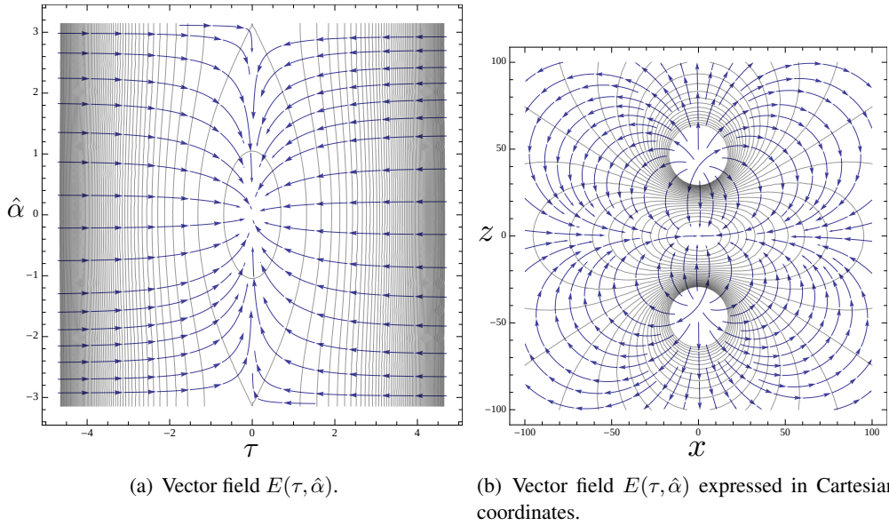
Figure 4.6: Vector field obtained as the gradient of F(\tau, \hat{\alpha}) with K = 1 .
