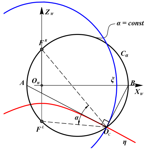
Figure 4.3: For any point O_c = (x, z) there always exists a circle C_\alpha passing through O_c and the projections in the motion plane of landmarks F^L and F^R . The angle at the circumference \alpha is constant along C_\alpha . Notice that, the tangent and perpendicular line in O_c to the hyperbola through O_c , intersect the X_W axis in points A and B , respectively. The segment \overline{AB} is the diameter of circle C_\alpha .
