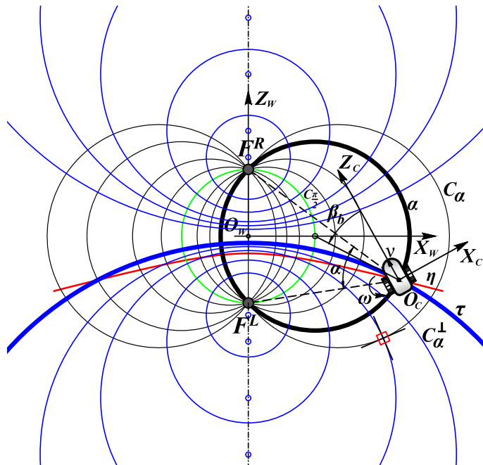
Figure 4.4: The bipolar coordinate system consists of two orthogonal bundles of circles. Starting from the same point O_c , circle C_\alpha^\perp crosses segment \overline{F^L F^R} in a point which is closer to the middle of the door than the one reachable by following the hyperbola through O_c .
