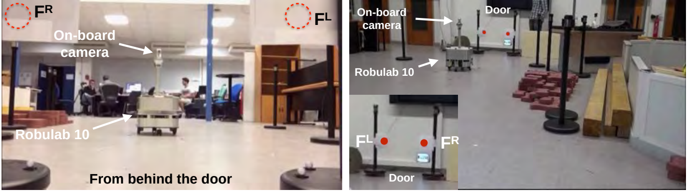
Figure 4.11: Experimental setup.
