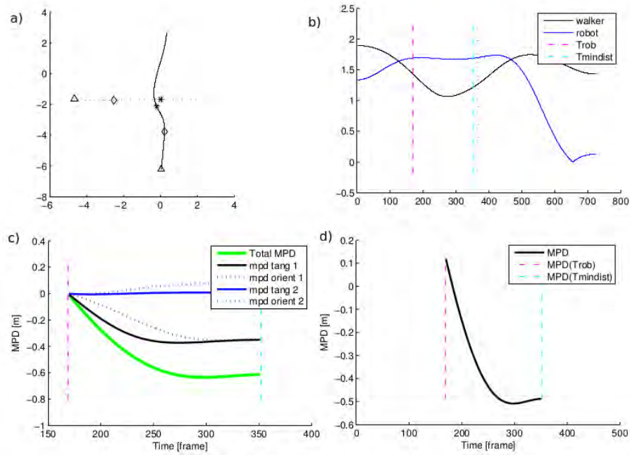
Figure 1.5: Example of the analysis of one trial in which a switch of mpd sign occurred. a) robot and pedestrian trajectories during the trial: triangles and star points are their position at t_{rob} and t_{cross} respectively. b) velocity profile of the walker and the obstacle. c) mpd components. d) mpd evolution during reaction phase (between t_{rob} and t_{cross} ).
