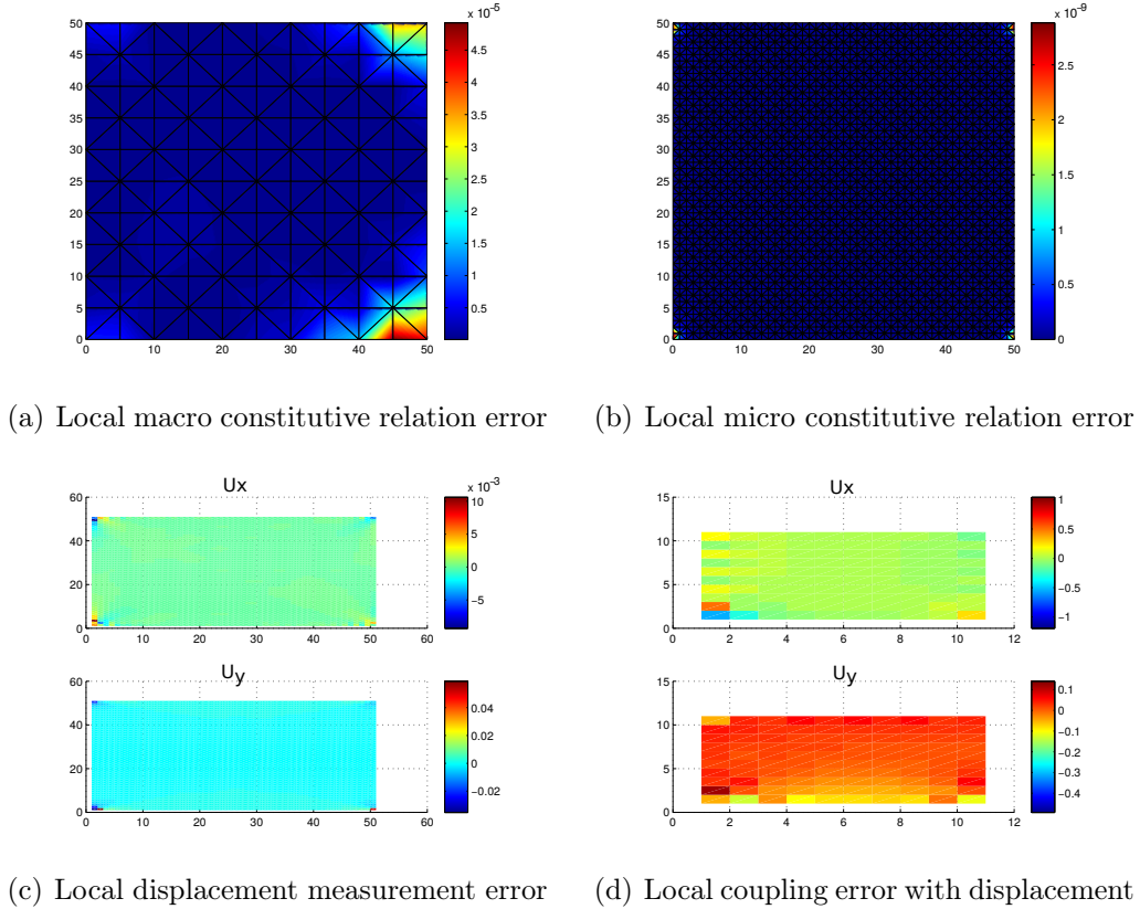
Figure 6.4: Local contributions to the terms of \mathcal{J} - case of a heterogeneous plate for identifying both macro and micro properties on the tension test
