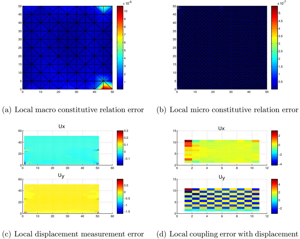
Figure 6.9: Local contributions to the terms of \mathcal{J} - case of a heterogeneous plate for identifying both macro and micro properties on the bending test
