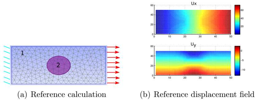
Figure 4.4: Numerical example of a plate with a single inclusion: reference calculation and simulated displacement exact measurement
