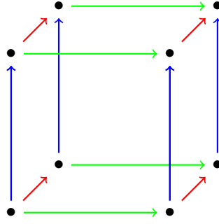
Figure 1.3: A cube for n = 3 ; each color corresponds to an event.
