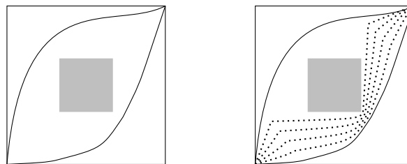
Figure 2.2: Non-(di)homotopic dipaths
