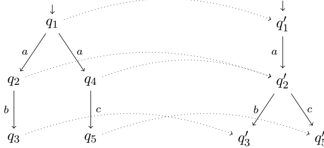
Figure 1.1: Two transition systems T (on the left) and S (on the right), and a morphism from T to S
