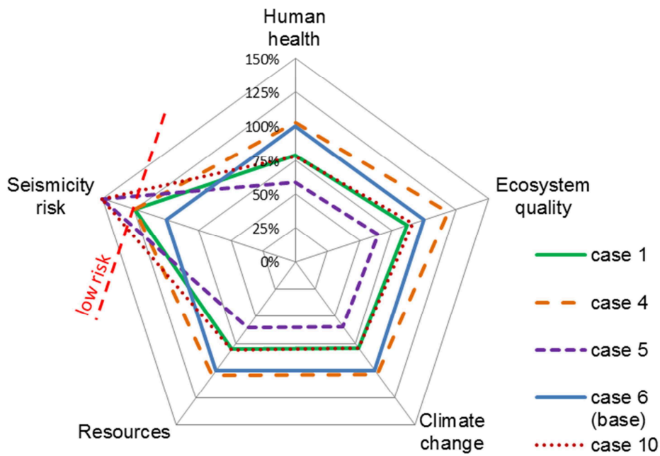
Figure 1.18 LCA results of case 1, 4, 5, 6 and 10 (production of 35-40 kg/s from one well)
