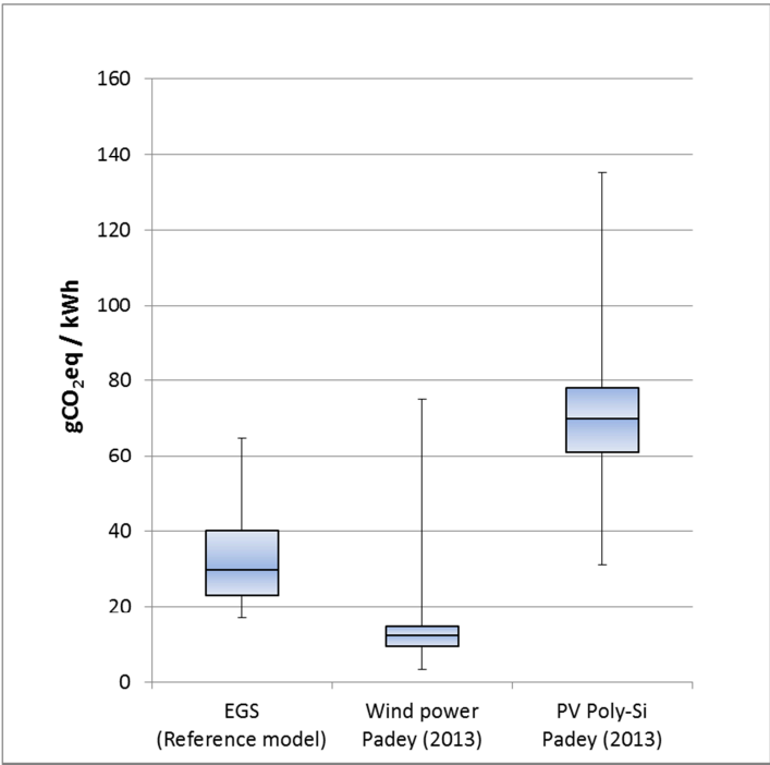
Figure A.13 Environmental profile of EGS issued from the Reference model , compared with the profile of two other renewable energy technologies: wind turbines and polycrystalline photovoltaic systems (Padey 2013).
