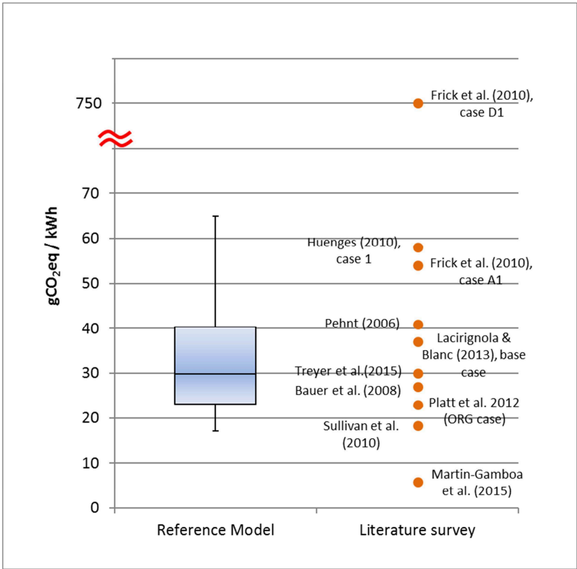
Figure 2.2 Environmental profile compared with results of detailed LCAs from literature
