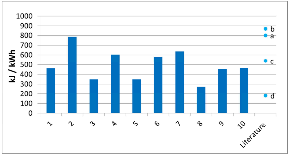
Figure 1.14 Results of the ten case studies (Resources) compared with literature. a: Frick et al. (2010) site A1; b: Huenges (2010) case 1; c: Pehtnt (2006); d: Sullivan et al. 2010. Other publications do not present estimates related to this impact category
