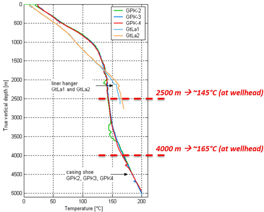
Figure 1.3 Temperature logs in Soultz-sous-Forêts (GPK-2, GPK-3, GPK-4 wells) and Landau (GtLa1, GtLa2 wells), adapted from Schindler et al. (2010)
