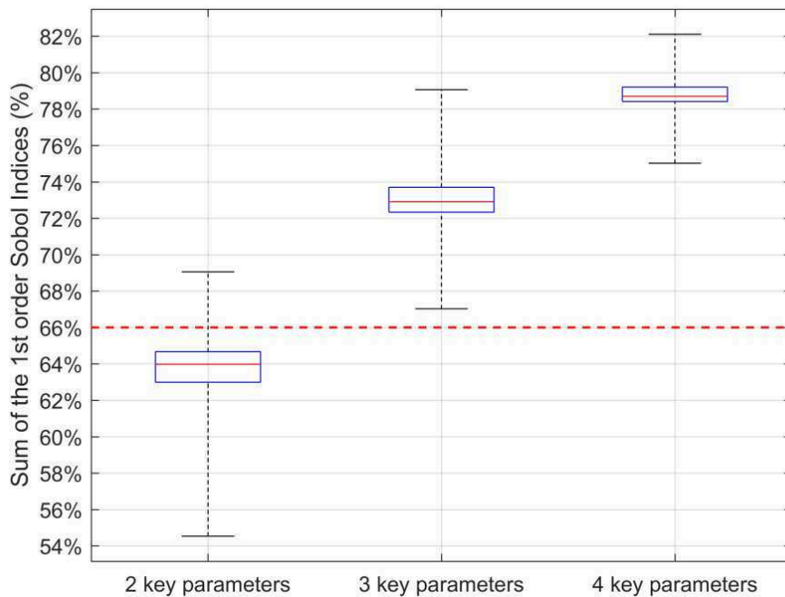
Figure 3.7 Sum of the S_i^{First} of the top two, three and four parameters in the ranking. The boxplots are based the results of 3500 GSAs as defined in Table 3.2
