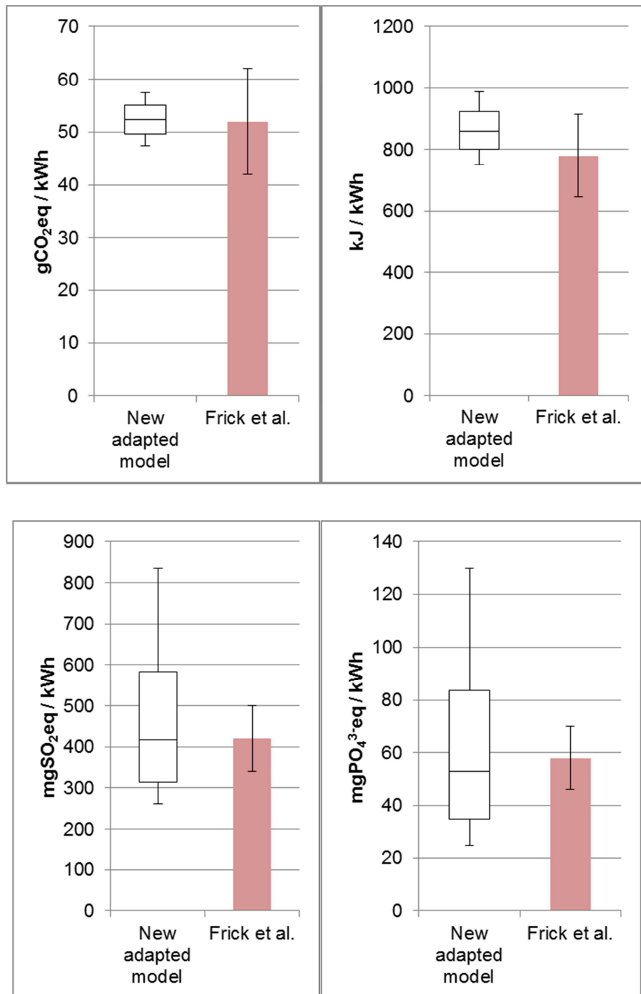
Figure A.5 Comparison of the results of our LCA model (adapted to the hypothesis of the scenario B1) with the results of Frick et al. (2010). Uncertainties are calculated with Monte Carlo Analysis (5000 simulations) Top and bottom of the box: 25 th and 75 th percentile.
