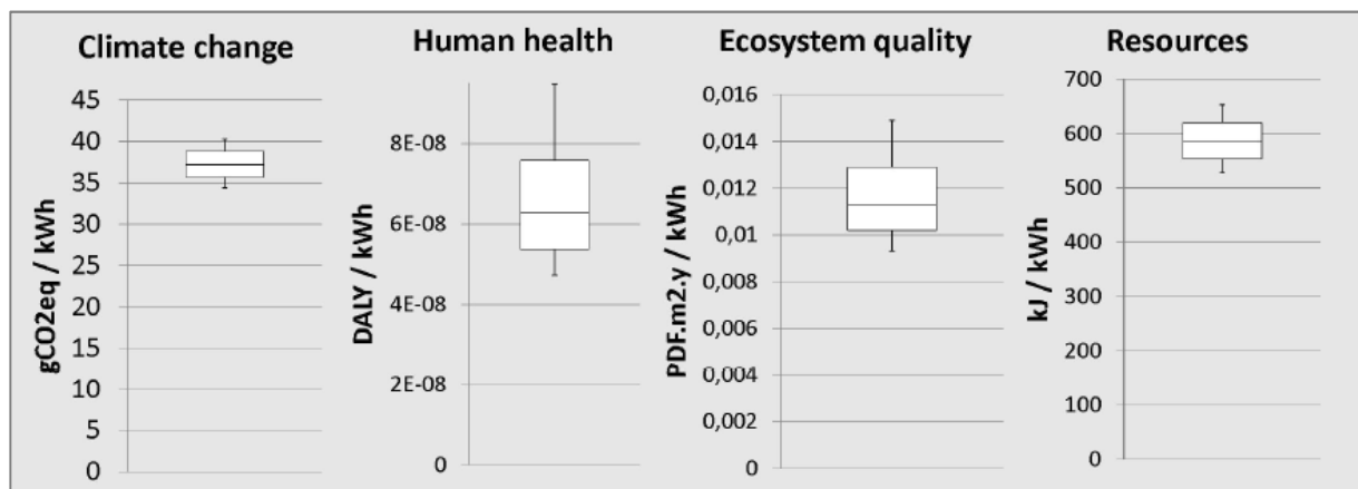
Figure 1.8 LCA results for the base case. Uncertainties calculated with Monte Carlo analysis. The central line indicates the median after 5000 simulations. Bottom and top of the box: 25th and 75th percentile. Whiskers: 10th and the 90th percentile.
