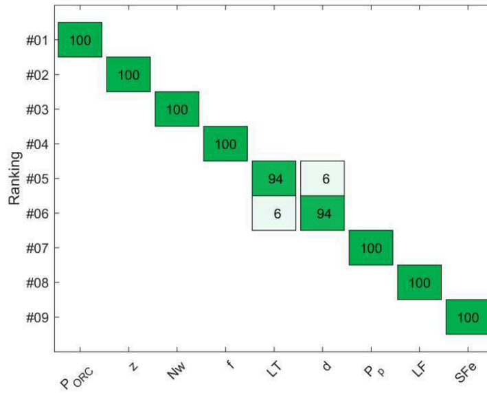
Figure 3.4 Results of the baseline GSA: ranking results for 100 bootstraps of the Baseline GSA. Given that the S_i^{First} of LT and d are very close, their ranking position can swap.
