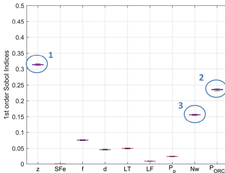
Figure A.15 Results of a GSA under a different hypothesis for the description of the variability of P_{ORC} (for all the other parameters, the baseline distributions are used): the blue circles indicate the three highest parameters of the ranking.
