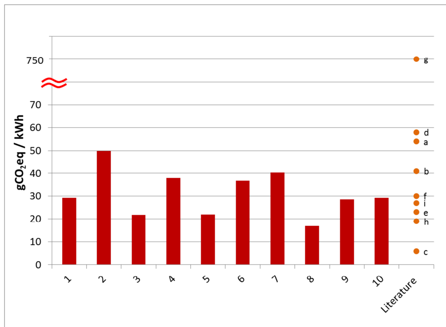
Figure 1.13 Results of the ten case studies (Climate change) compared with literature. a: Frick et al. (2010) site A1; b: Pehnt (2006); c: Martin-Gamboa et al. (2015); d: Huenges (2010) case 1; e: Platt et al. (2012); f: Treyer et al. (2015); g: Frick et al. (2010) case D1 (which is confirmed to be a “stand alone” estimate); h: Sullivan et al. (2010); i: Bauer et al. (2008)
