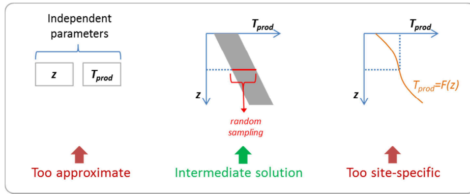
Figure 4.4 Solution for establishing a relation between the production temperature and the drilling depth
