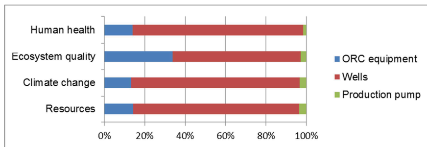
Figure 1.7 Contribution of the system elements to the four impact categories (base case)
