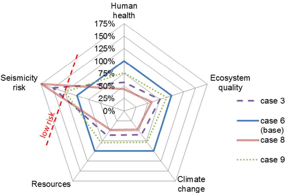
Figure 1.17 LCA results of case 3, 8, 9 (production of 70 kg/s from one well)
