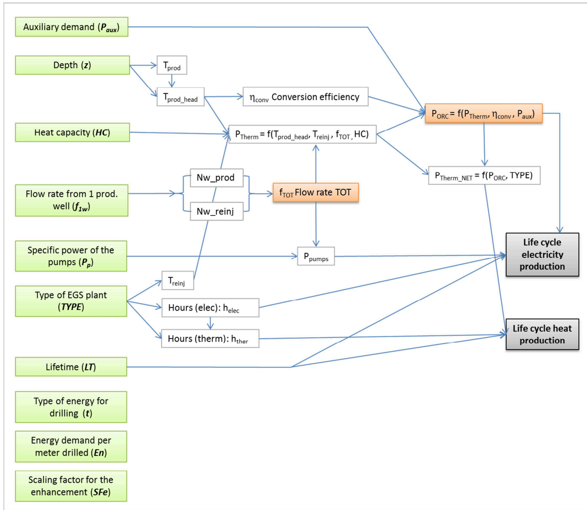
Figure 4.2 Ten independent parameters (green boxes) of a possible updated version of the Reference model. The installed capacity and the flow rate are now dependent variables (orange boxes)
