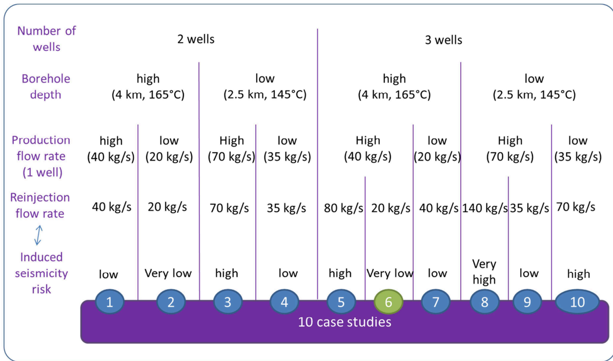
Figure 1.2 Features of the 10 case studies. Case no. 6 is selected as “base case”
