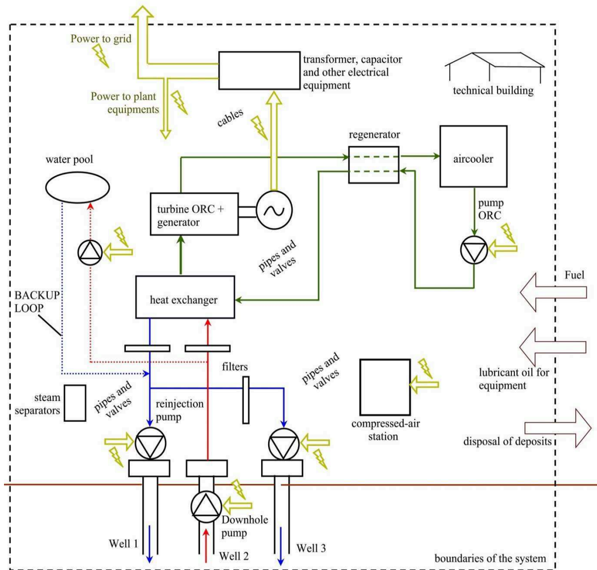
Figure 1.5 System boundaries for the analyzed EGS (base case)
