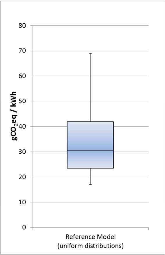
Figure A.12 Environmental profile of EGS, considering uniform variability distributions for the nine parameters
