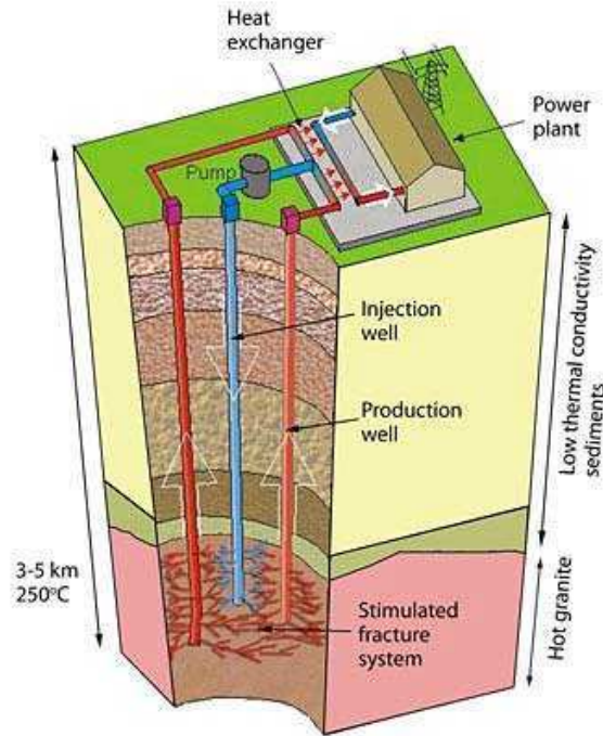
Figure I.3 Conceptual scheme of an EGS (from geothermalworldwide, 2016). In this picture two wells are used for production and one for reinjection, but other circulation schemes based on 2 or 3 wells are also possible as discussed in the manuscript.
