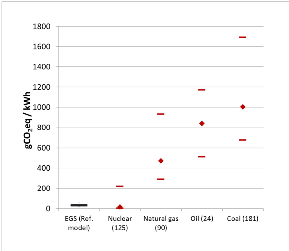
Figure 2.4 Environmental profile of EGS issued from the Reference model , compared with the LCA results of non-renewable energy technologies issued from a literature review performed by the IPCC (Moomaw et al. 2011). Between brackets: number of GHG estimates considered in the review.
