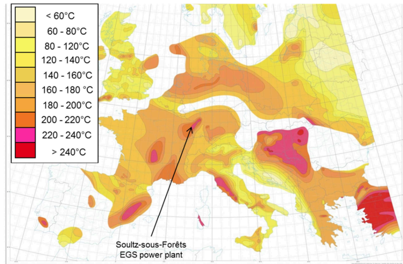
Figure I.2. Map of the temperature extrapolated at 5 km depth in Europe (from Hurtig et al, 1992)
