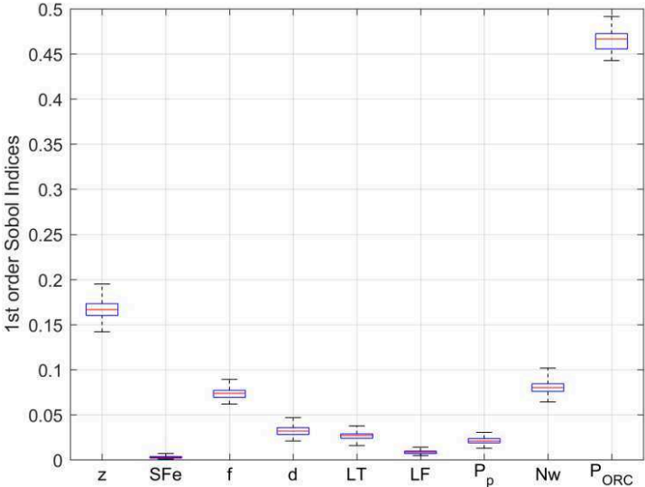
Figure A.14 Results of the baseline GSA (first order Sobol Indices of the nine input parameters) when a reduced sample (5000 values per input parameter) is used.
