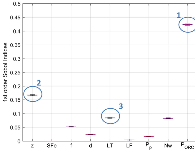
Figure 3.6 Results of a GSA under a different hypothesis for the description of the variability of LT (for all the other parameters, the baseline distributions are used): the blue circles indicate the three highest parameters of the ranking
