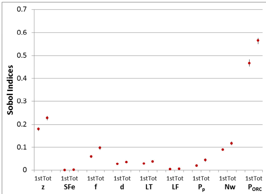
Figure 3.5 First order (“1st”) and total order (“Tot”) Sobol Indices for the Baseline GSA, calculated with samples of 500 000 values per parameter.
