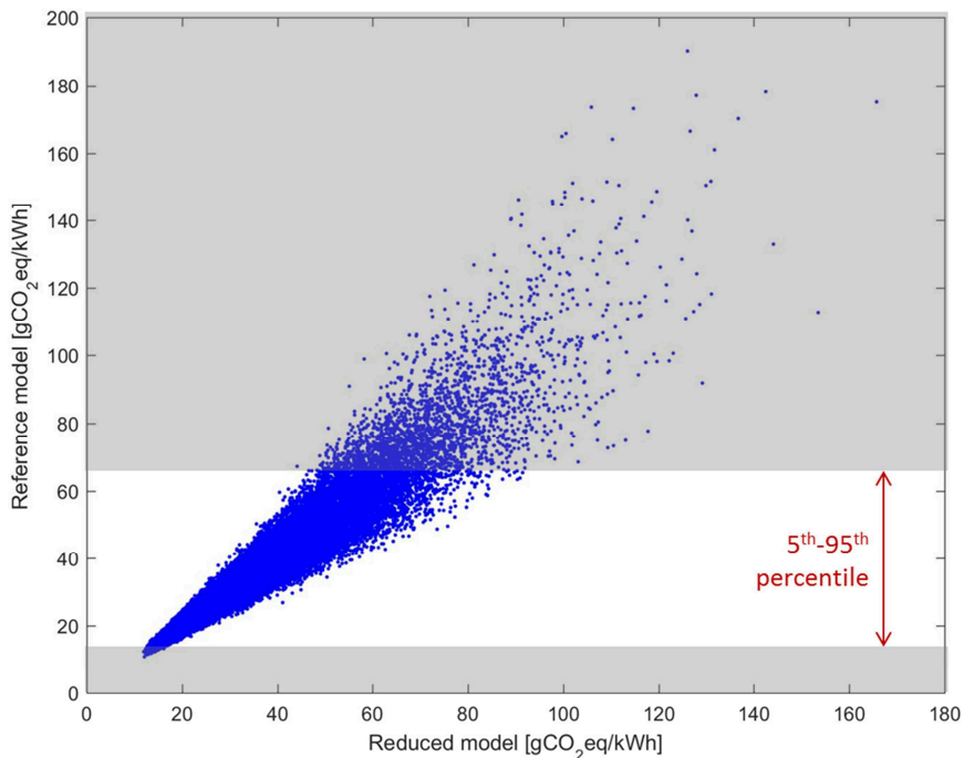
Figure A.17 Affinity between the Reference model and the Reduced model (50 000 simulations).
