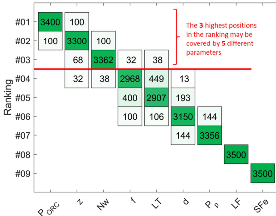
Figure 3.9 Sensitivity of the ranking with respect to the description of the input parameters: aggregated results of the analysis one parameter at a time
