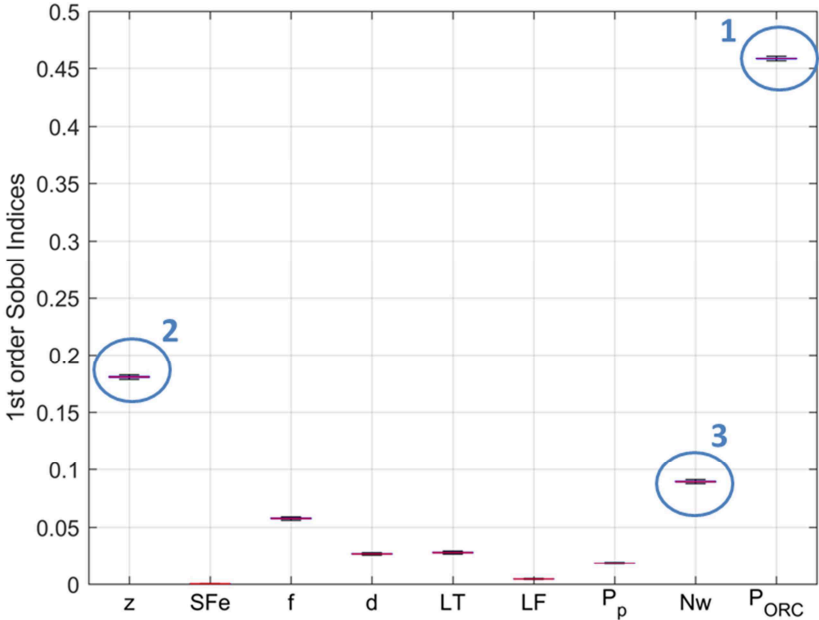
Figure 3.3 Results of the baseline GSA: first order Sobol Indices of the nine input parameters. The blue circles indicate the three highest parameters of the ranking.
