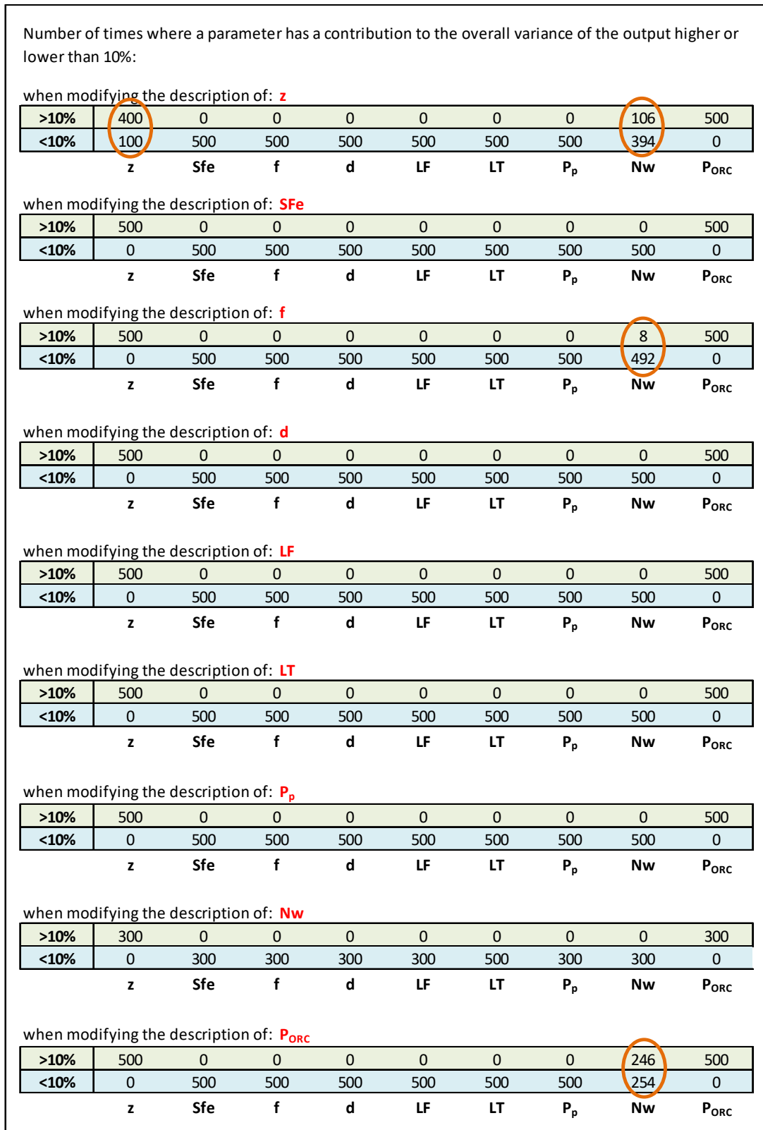
Figure A.16 Sensitivity of the GSA results with respect to the description of the input parameters: analysis one parameter at a time. The analysis is based on the threshold for the single contribution of each parameter to the overall variance of the output
