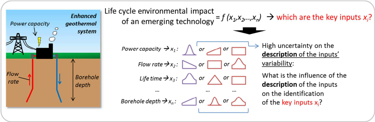
Figure 3.1 Representation of the high uncertainty on the description of the inputs as critical issue when identifying the key parameters
