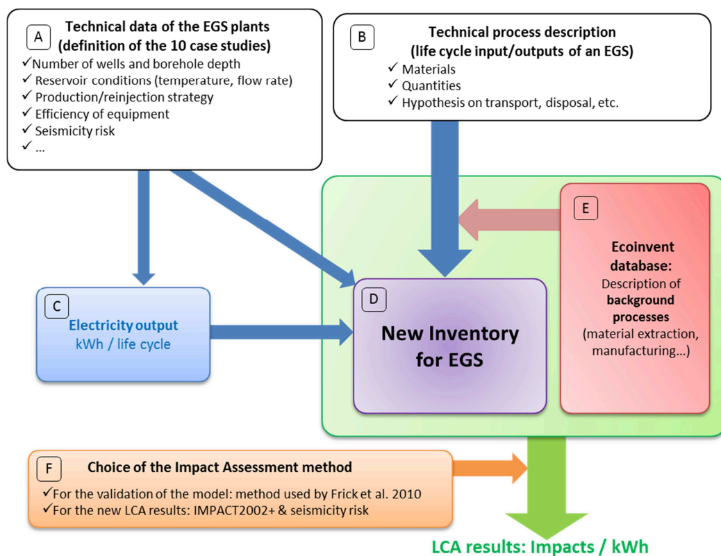
Figure 1.1 Methodology applied in this chapter for the detailed LCA of EGS
