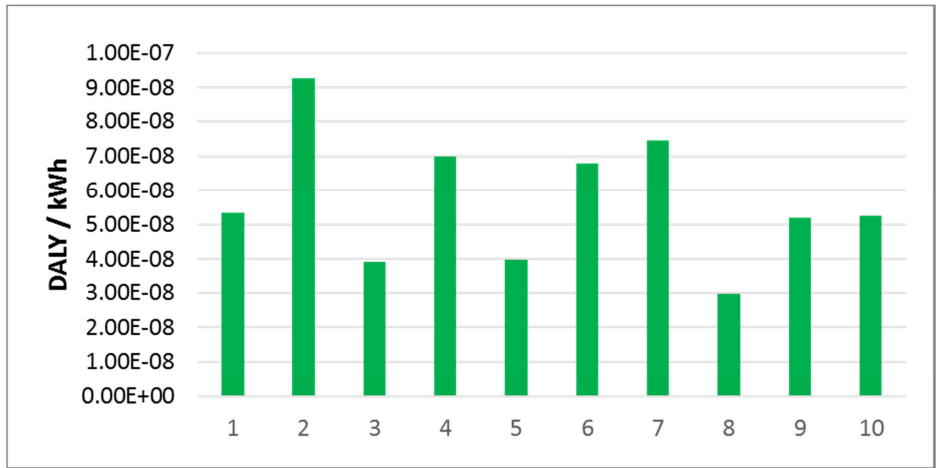
Figure 1.15 Results of the ten case studies (Human health)
