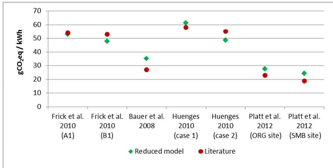
Figure 3.10 Comparison of the results of the 5-variables Reduced model with literature.
