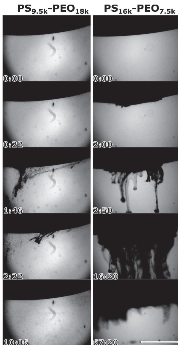
Figure 5 Evolution of the chloroform droplet from instability at minimum (1x) flow rate. On the left \text{PS}_{9.5\text{k}}\text{-PEO}_{18\text{k}} is shown. Upon visible surface instability, small droplets of chloroform in water are formed. This is followed by a more pronounced stream of chloroform droplets diffusing towards the water phase. As a result a chloroform in water micro-emulsion is formed within ten minutes from the onset of surface instability. Complete evaporation of the volatile dispersed phase will result in a water solution of spherical micelles. On the right the \text{PS}_{16\text{k}}\text{-PEO}_{7.5\text{k}} is shown. Upon surface instability, this copolymer caused the formation of elongated finger-like instabilities. The growth of these structures continued for approximately one hour. After this time, the solution appeared to be locally turbid. This was due to localized networks of elongated micelles. Scale bar 1 mm, time stamps in min:sec.
