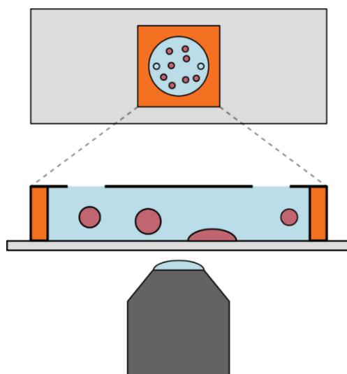
Figure 11 Schematic view of the experimental setup to observe the formation of micelles through the evaporating emulsion droplets. In the top is a top view of the glass slide and imaging chamber. Below this is close-up scheme showing, from the side, the emulsion droplets in the chamber and the position of the inverted microscope objective.
