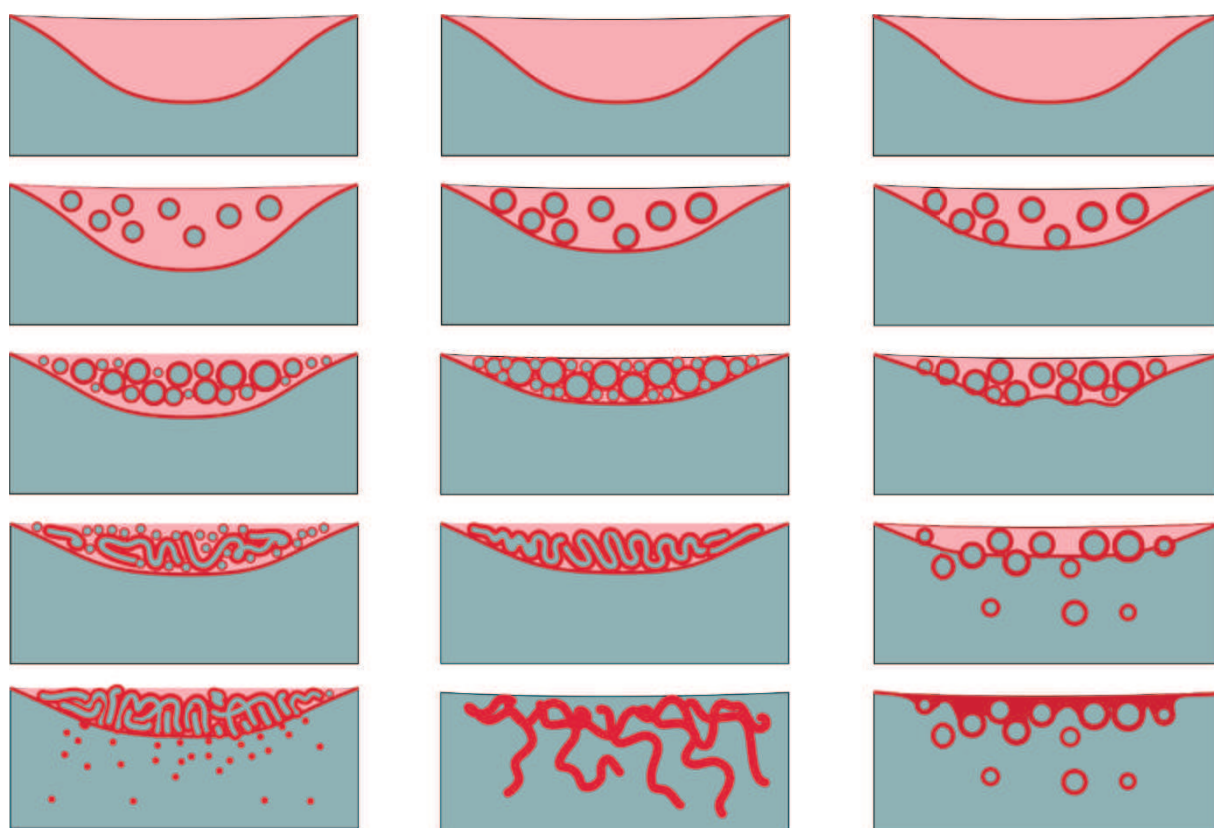
Figure 12 Overview of the different formation mechanisms of the \text{PS}_{9.5k}\text{-PEO}_{18k} micelles. From left to right is increasing the evaporation rate and from top to bottom are shown the characteristic timeframes in succession. In the initial moment a chloroform solution containing copolymer is placed on top of a water volume and the copolymer is adhering at the interface
