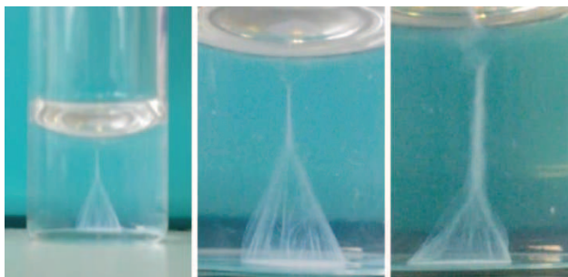
Figure 13 Bundles of elongated micelles of PS_{16k}\text{-}PEO_{7.5k} forming a microscopic thread.
