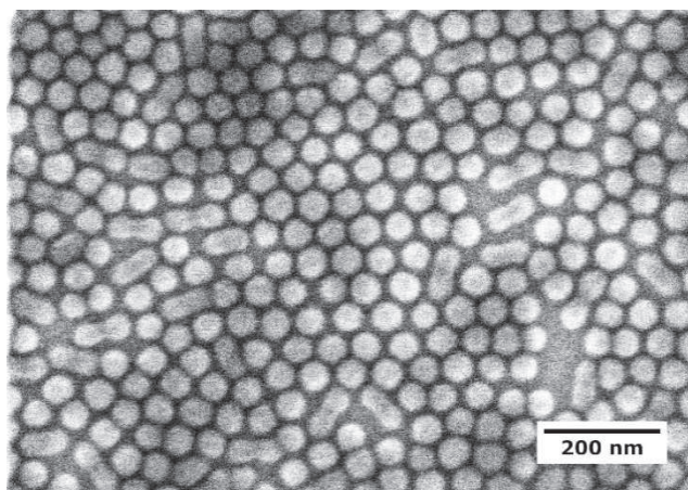
Figure 10 Scanning Electron Microscopy image of spherical micelles spontaneously formed at a chloroform water interface in presence of PS 9.5k -PEO 18k . A fraction of the micelles appears to have a 1:2 aspect ratio.
