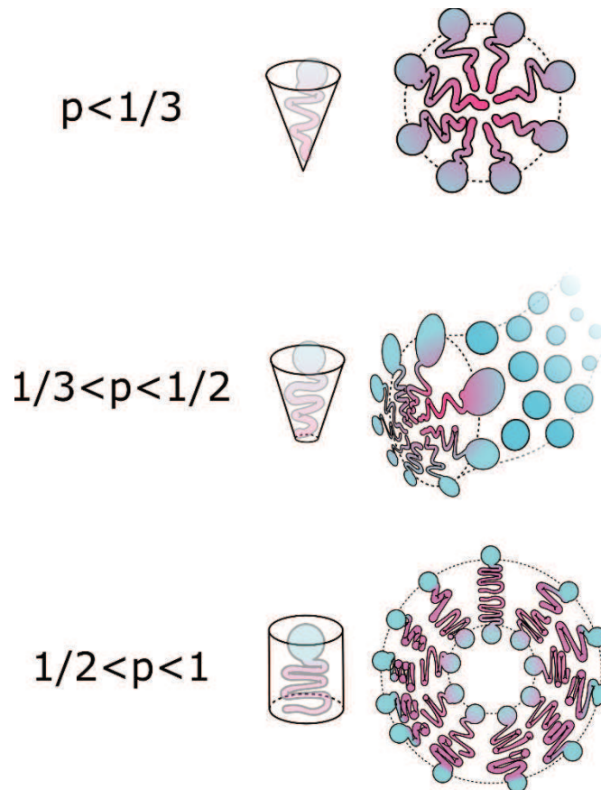
Figure 1 Overview of the different morphologies with their corresponding packing parameters. On the top are spherical micelles, in the center are elongated ones and on the bottom are bilayer morphologies (polymersomes or vesicles).
