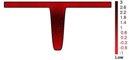
i Vertical actomyosin flow velocity ( v_y )
