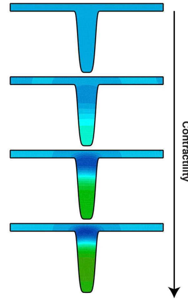
k Steady-state Myosin Concentration vs. Contractility
