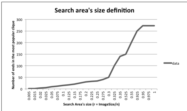
Fig. 3. A relation between the search area's size and the image resolution has been found. Large search areas reflect into cliques too popular ( n_{\text{members}} > 9 ), which are difficult to solve. The optimal search area has been chosen so that the largest cliques discovered in our training sets have nine segment ends.
