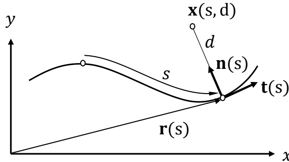
Figure 4.10 The Frenet frame on a curve
