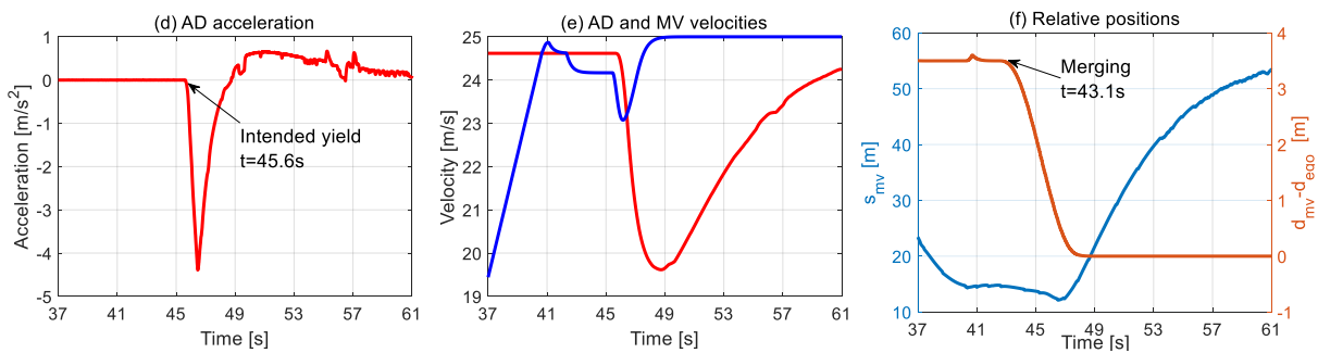
Figure 5.12. Comparison of the simulation results of the cooperative longitudinal control system and a standard ACC in S1
