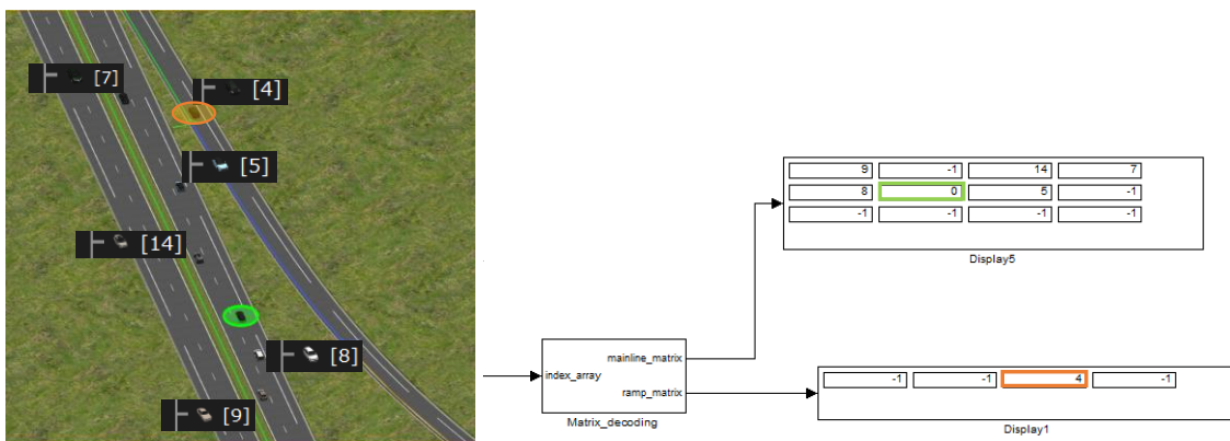
Figure 4.16 Illustration of a fluid traffic with a mainline road and a ramp. The ego vehicle is surrounded by a green circle. The on-ramp vehicle is highlighted in orange.
