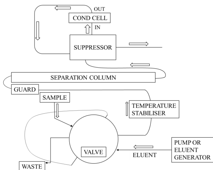
Figure 101. The general instrumental set-up of ion chromatography procedure.
