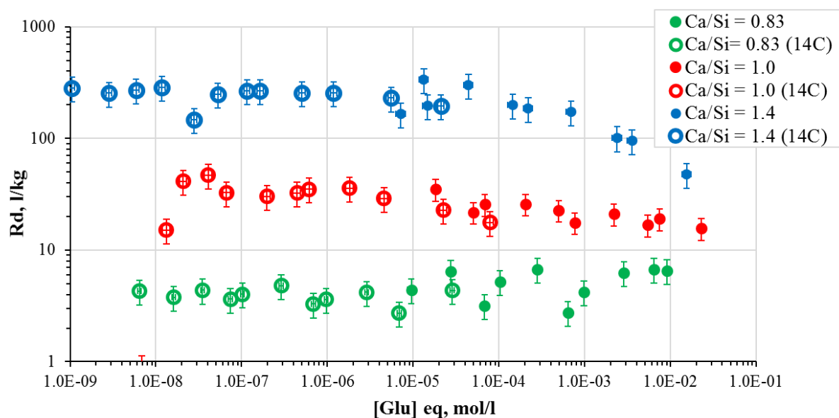
Figure 43. The distribution ratio ( R_d ) for gluconate adsorption on C-S-H phases with three \text{Ca/Si} ratios.
