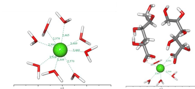
Figure 61. Simulation snapshots of the \text{Ca}^{2+} hydration shell and the complex with gluconate ions.
