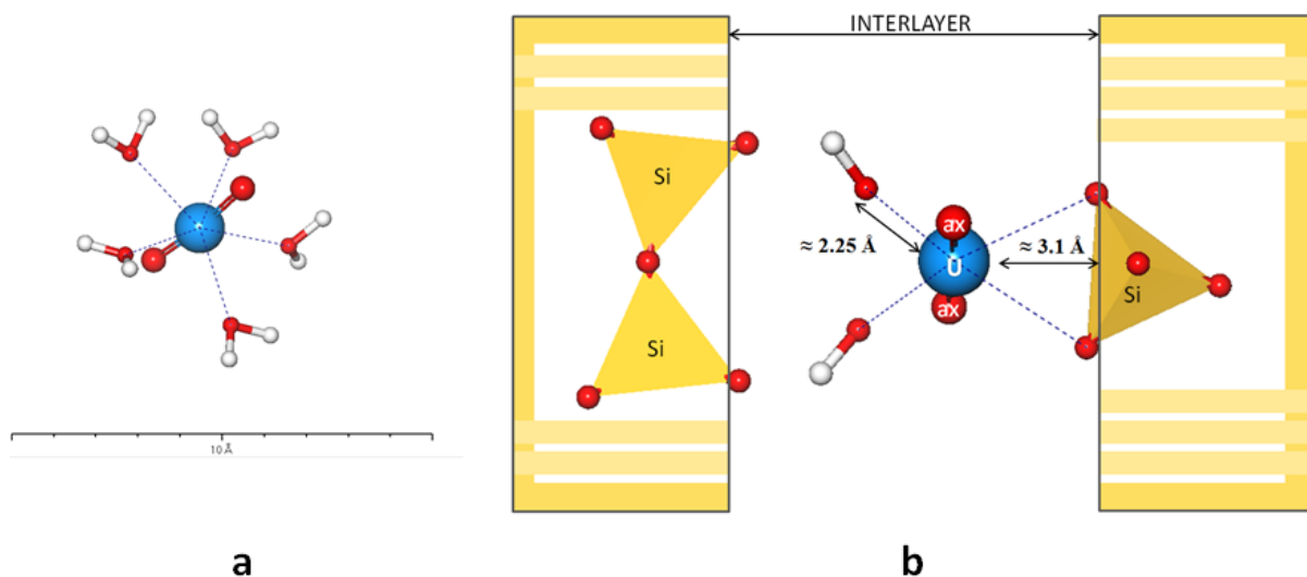
Figure 10. a – Uranyl cation ( \text{UO}_2^{2+} ) with its hydration shell; b – An interlayer incorporation model for \text{UO}_2(\text{OH})^{2-} in C-S-H proposed by Macé et al. (2013).
