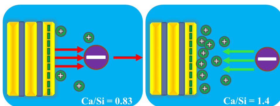
Figure 44. The mechanism of gluconate/C-S-H interaction. Yellow bricks – C-S-H particles, green circles – \text{Ca}^{2+} cations, violet circle – gluconate anion.
