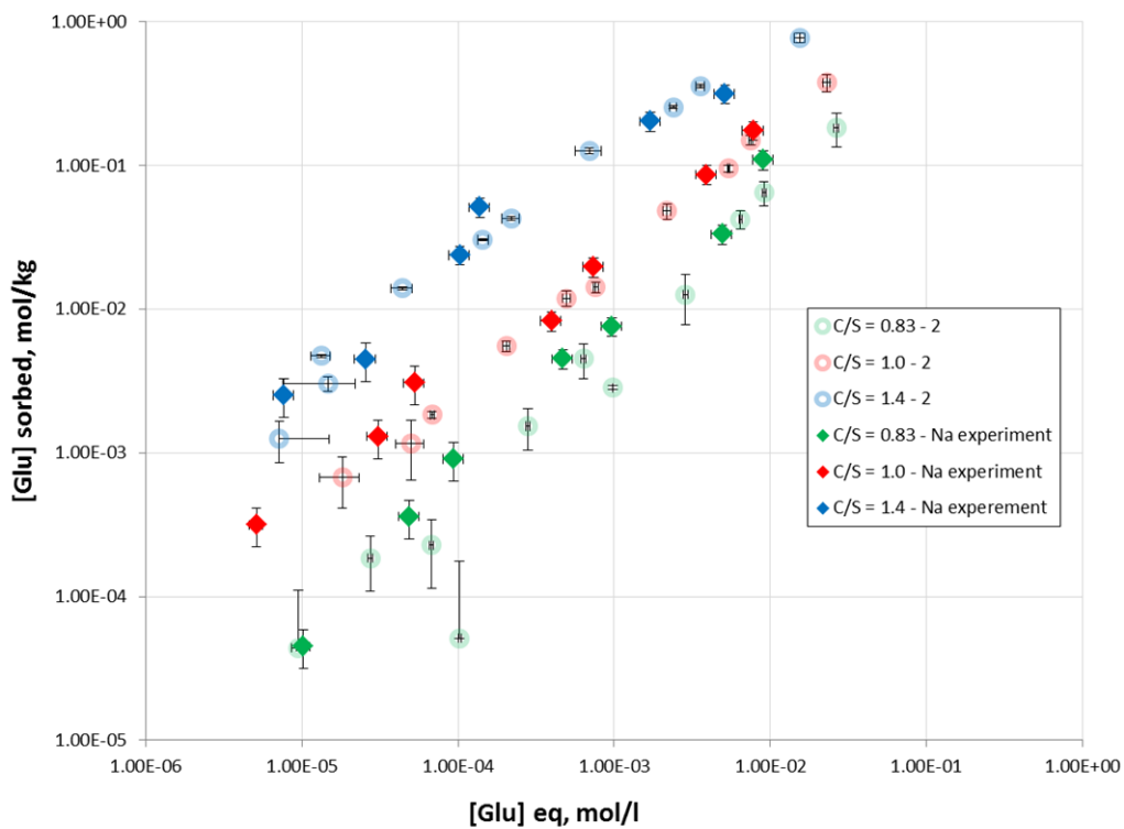
Figure 47. The isotherm of gluconate adsorption on C-S-H with different Ca/Si. The results of the previous study are shown for comparison (labeled by -2 here).
