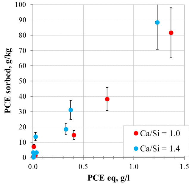
Figure 55. The isotherms of PCE adsorption on C-S-H phases with \text{Ca/Si} = 1.0 and \text{Ca/Si} = 1.4 .
