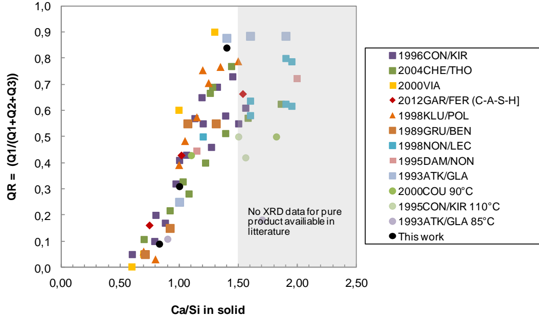
Figure 24. Correlation of Q_R value with Ca/Si ratio in the C-S-H structure (adapted from Roos, (2016) with permission)
