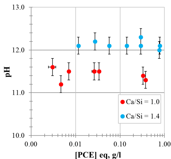
Figure 56. pH values of C-S-H equilibrated solutions as a function of the PCE concentration in the steady state.
