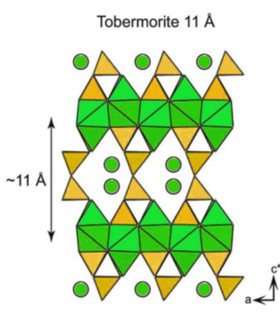
Figure 5. A three dimensional view of the tobermorite structure using the orthorhombic axis a/2 = 5.58 \text{ Å} , b = 7.39 \text{ Å} , and c/2 = 11.389 \text{ Å} (Hamid, 1981; Grangeon, 2013).
