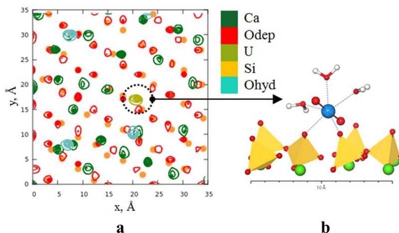
Figure 87. The time-averaged distribution of \text{UO}_2^{2+} ions at the CSH-1.4 interface within 1.0 – 2.0 Å from the surface: (a) - the first molecular layer; (b) – the inner-sphere \text{UO}_2^{2+} surface. The colour scheme is the same as in Fig. 86.
