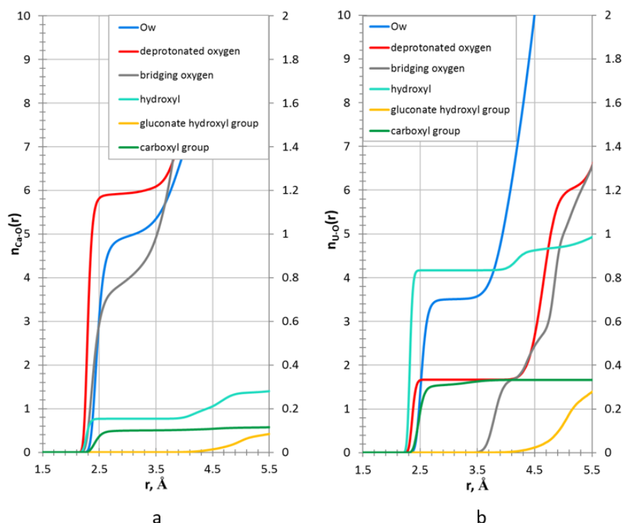
Figure 93. The running coordination numbers for pairs of \text{Ca}^{2+} (a) and \text{UO}_2^{2+} (b) and different oxygen atoms in the CSH-1.4 interfaces (left scale for Ow).
