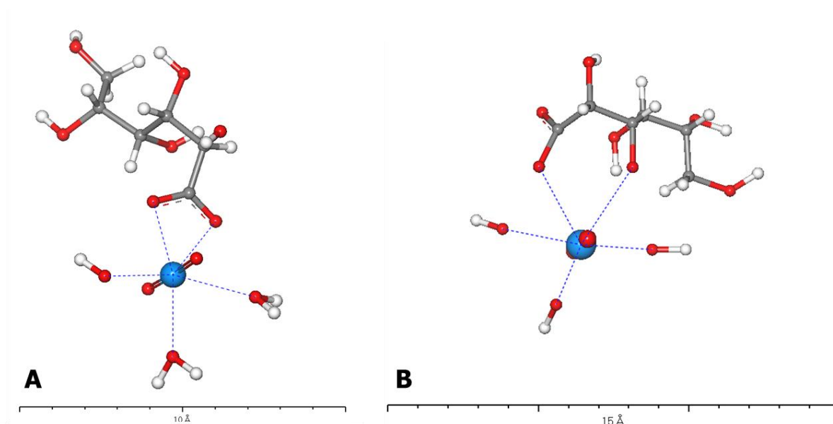
Figure 11. UO_2^{2+} / gluconate ion complexation (ratio 1:1): A – at pH < 13.9 ; B – at pH > 13.9 (Birjukumar et al., 2011).
