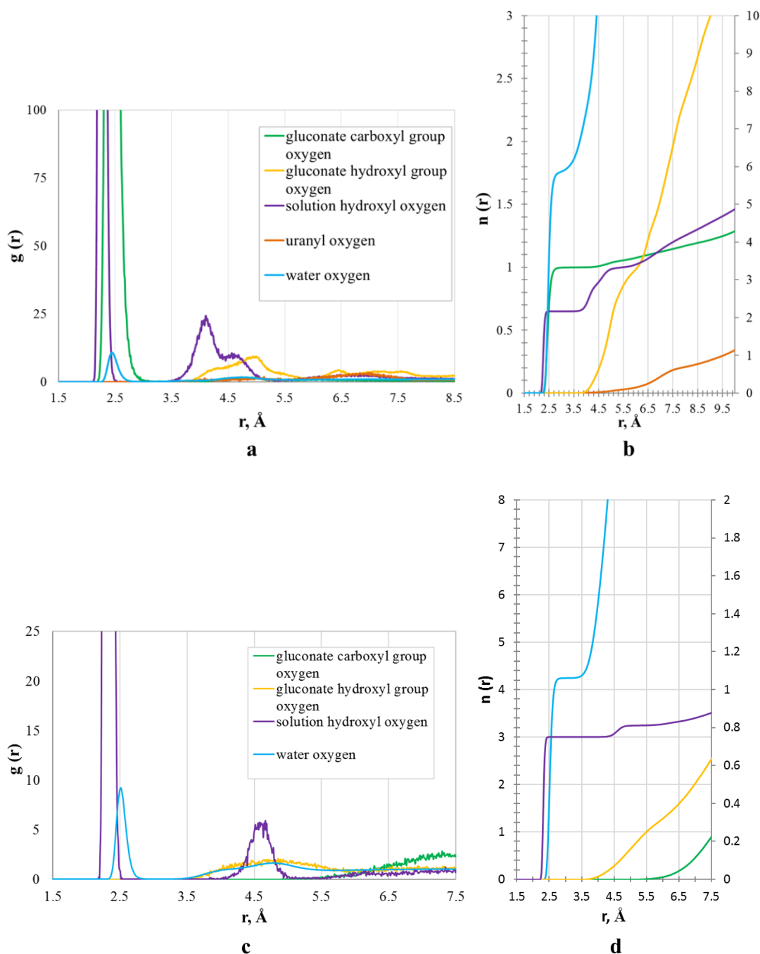
Figure 64. Local structural properties of calcium gluconate/uranyl solution: (a) – radial distribution functions for Ca-O pairs; (b) – running coordination numbers; (c) – radial distribution functions for U-O pairs; (d) – running coordination numbers.
