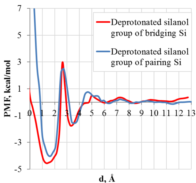
Figure 81. The potential of mean force as a function of distance between \text{Ca}^{2+} and two chosen deprotonated silanol groups of the CSH-0.83 surface.
