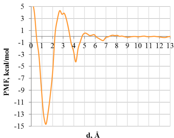
Figure 91. The potential of mean force as a function of distance between \text{UO}_2^{2+} and deprotonated silanol groups of the CSH-1.4 surface.
