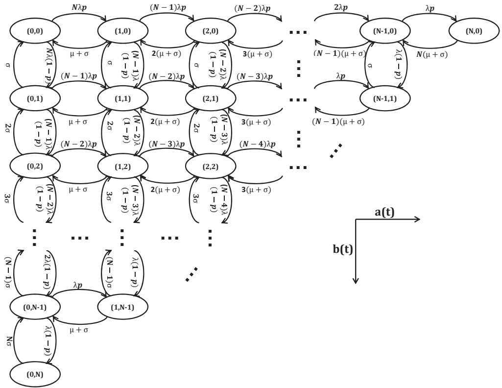
Figure 3.3: Bi-dimensional Markov chain diagram
