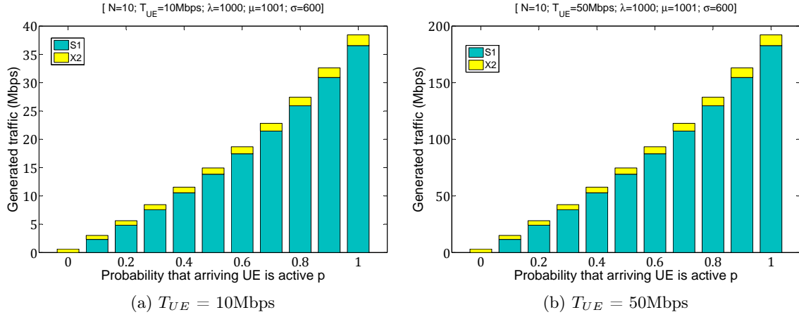
Figure 3.7: Generated traffic flows shares on interfaces S1 and X2 versus p
