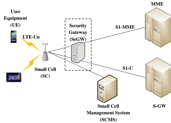
(c) 4G Small Cells Architecture (Variant 2)
