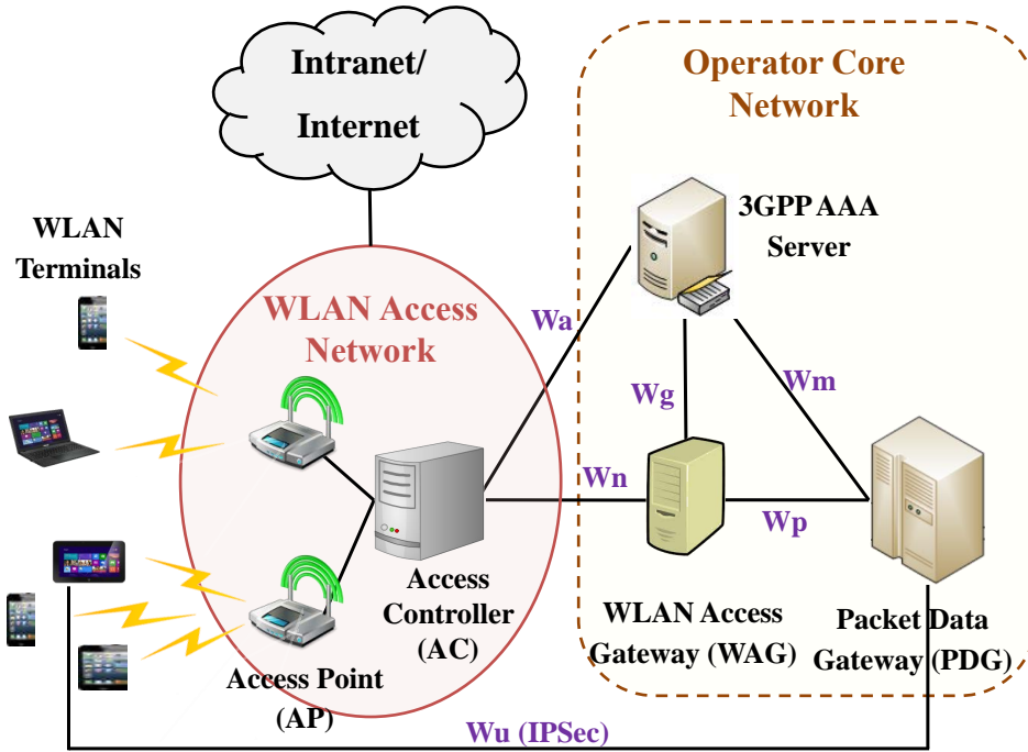
Figure 1.3: A simplified Operator WLAN architecture
