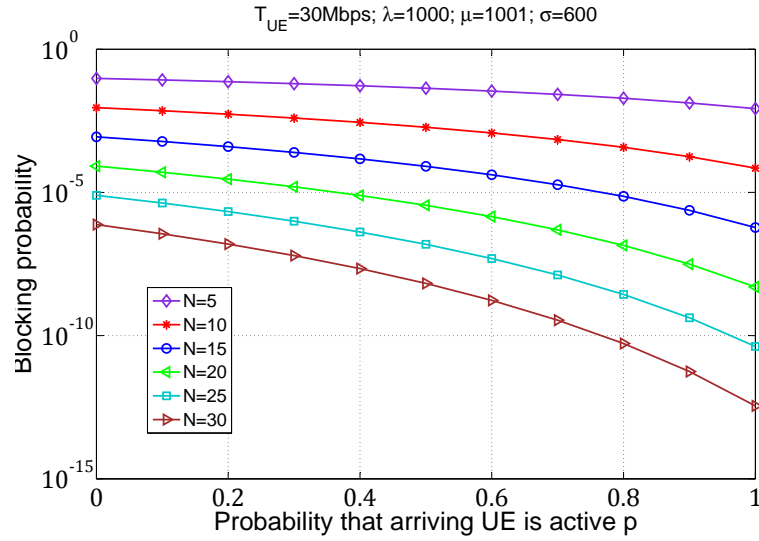
Figure 3.8: Blocking probability versus p
