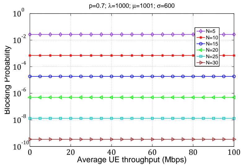
Figure 3.9: Blocking probability versus T_{UE}
