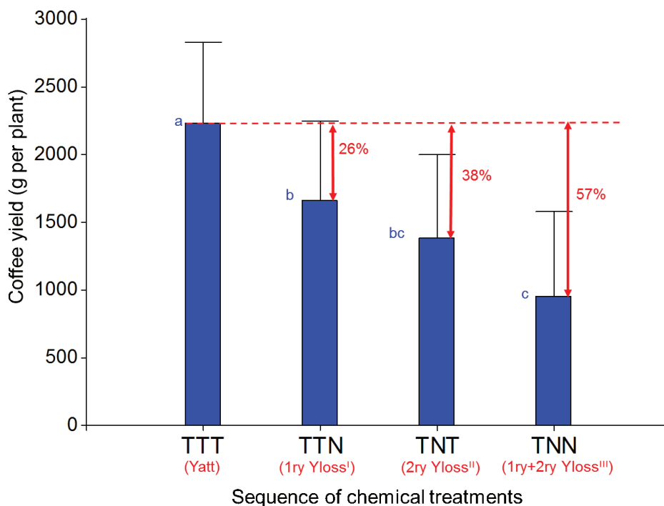
Fig. 4.3. Yields and primary and secondary yield losses resulting from the sequences of chemical treatments TTT, TTN, TNT, TNN
