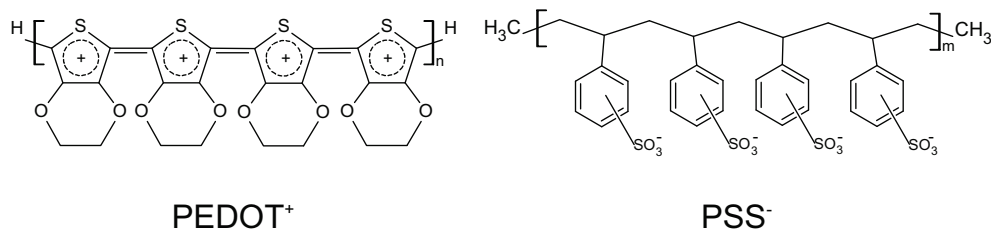
Fig. 4.1. Chemical structure of poly(3,4-ethylenedioxythiophene) ( PEDOT ) and polystyrene sulfonate ( PSS )
