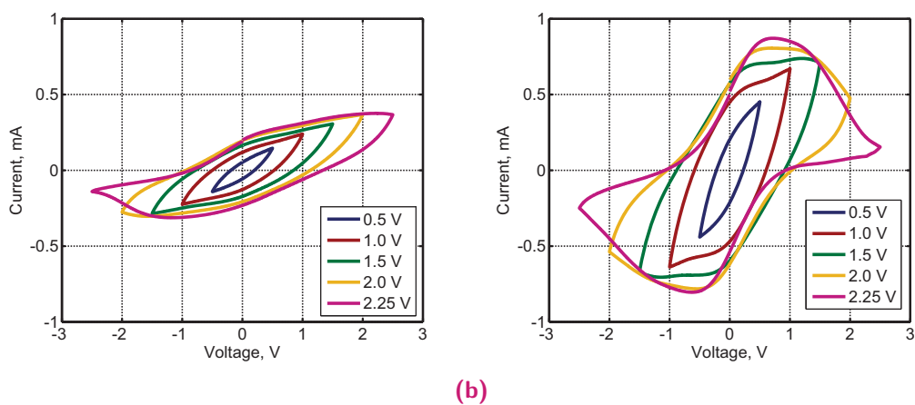
Fig. B.6. Cyclic voltammograms of the trilayer PEDOT:PSS/mPVDF/PEDOT:PSS actuators obtained with 100\text{ mV/s} scan rates and different voltages indicated in the legend. PEDOT:PSS was secondary doped with (a) 1 vol% or (b) 2 vol% of PEG400.
