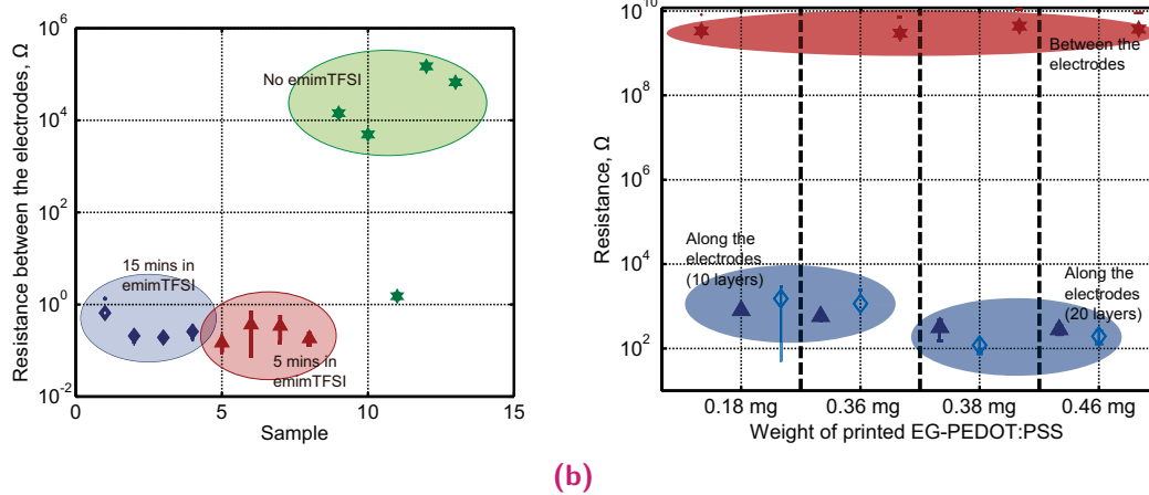
Fig. B.13. (a) Resistance between the electrodes before (green) and after incubation in ionic liquid for 5 (red) or 15 minutes of actuators fabricated by drop casting. (b) Electrical resistance measurements of printed PEDOT:PSS actuators. Resistance along the electrodes is shown in blue (different shades of blue indicate the conductivities measured on different sides), resistance in between the electrodes is shown in red.
