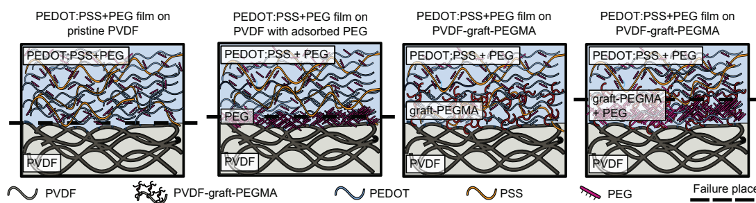
Fig. 3.16. Schematic drawing of different PVDF functionalisation methods and their influence on adhesion with PEDOT:PSS
