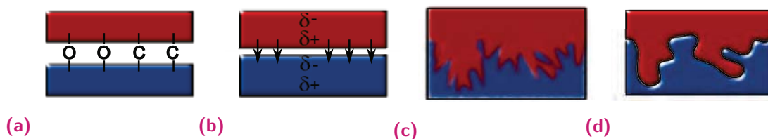
Fig. 3.1. Illustration of different mechanisms playing important role in the adhesion of two polymer solids: (a) formation of a covalent bond, (b) van der Waals interactions, (c) interdiffusion of the polymer chains during welding, (d) direct mechanical interlocking.
