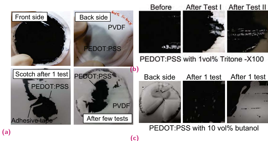
Fig. 3.7. (a) Pictures of PEDOT:PSS (with 1 vol% Triton X – 100) film deposited by solvent casting on pPVDF . Top: front and back sides after deposition and drying, bottom: adhesive tape after one adhesion test showing that most of PEDOT:PSS remained on the tape and the front side of the PVDF membrane after several application of adhesive tape showing that only at areas where PEDOT:PSS penetrated through the membrane adhesion is strong. (b) Adhesion test with a cut grid: Test I - after 5 applications of adhesive tape in a dry state; Test II - after incubation in ionic liquid for 24 hours and another 5 applications of adhesive tape. (c) Equivalent test performed on PVDF-PEDOT:PSS (diluted with 10vol% of i-butanol) sandwich showing that only at the penetration through area adhesion is strong.
