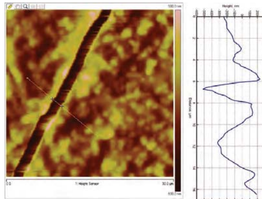
Fig. B.17. (a) SEM image of the PEDOT:PSS layer printed on the PVDF membrane (tilted) and (b) AFM image of the crack on the surface of printed PEDOT:PSS and the height profile.
