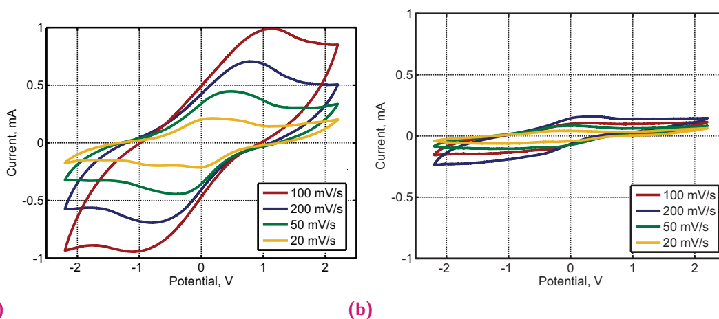
Fig. B.14. Cyclic voltammograms of actuators with (a) and (b) without post treatment with CNT . Scans were obtained at different scan rates indicated in the legend.
