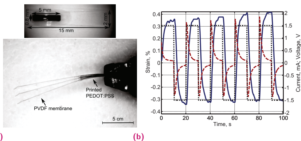
Fig. 5.8. (a) Merged images of the actuator at its initial position and extremities during the actuation with 1.5 V square wave at 50 mHz. The position of printed PEDOT:PSS is indicated with arrows. Dimensions of used actuator (2x15 mm) and printed PEDOT:PSS layer (0.8x5 mm) are shown above. (b) Displacement (blue line) and transferred current (red dashed line) profiles of printed actuator (10 layers, 0.36 mg) during actuation. The voltage waveform used is shown as black dotted line.
