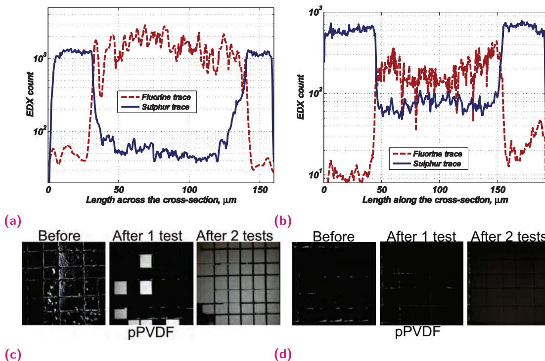
Fig. 3.13. EDX line scans for fluorine (red) and sulphur (blue) traces along the cross-section of the trilayers PEDOT:PSS/pPVDF/PEDOT:PSS ((a)-(b)) and adhesion tests of the PEDOT:PSS film deposited on the rough side of the membrane ((c)-(d)). For (a) and (c) PEDOT:PSS is secondary doped with 2 vol% PEG400, for (b) and (d) with 5 vol% PEG400.
