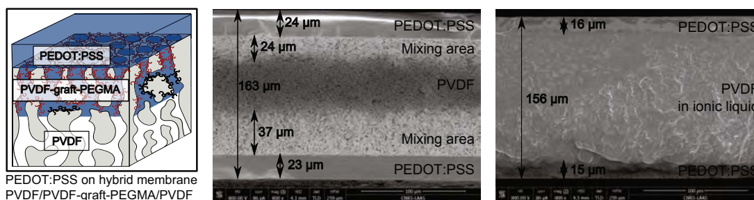
Fig. 4.6. Scheme of the interface and the mixing depth (penetration depth) of PEDOT:PSS and PVDF-graft-PEGMA and the SEM images of the cross-sections of the PEDOT:PSS/mPVDF/PEDOT:PSS trilayers before the immersion in the ionic liquid and after the immersion (2 hours). Different actuators fabricated on the membranes with GD - 0.22 \pm 0.03 were used for the measurements.
