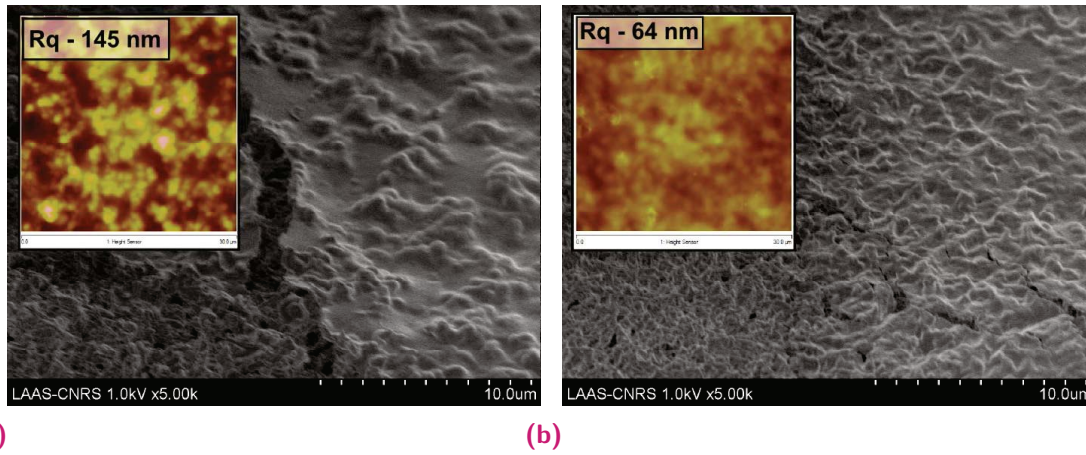
Fig. 5.3. SEM of PEDOT:PSS layer printed on (a) rough and (b) smooth side of the PVDF membrane at the printing borderline. Inset: AFM surface scan of the PEDOT:PSS printed on each side of the membrane.
