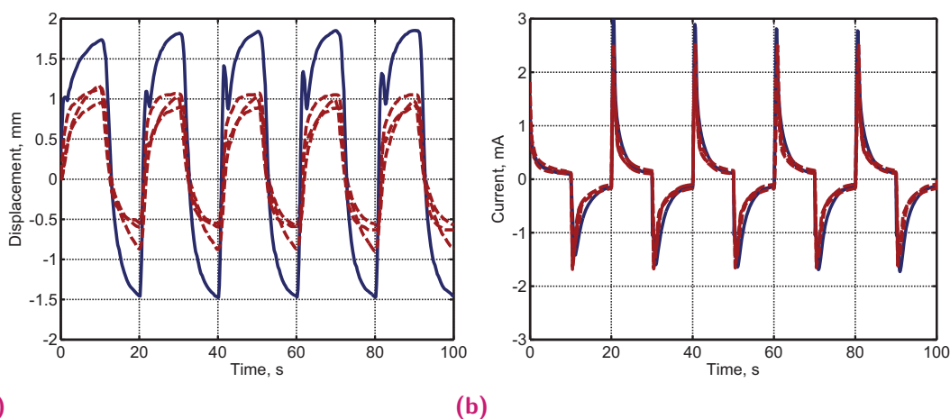
Fig. 4.18. (a) Bending and (b) transferred current profiles of the standard (red dashed line) actuators and actuators treated with sprayed sodium dodecyl sulfate (SDS) (blue full line). 1.5 V square voltage wave at 50 mHz was used for actuation.
