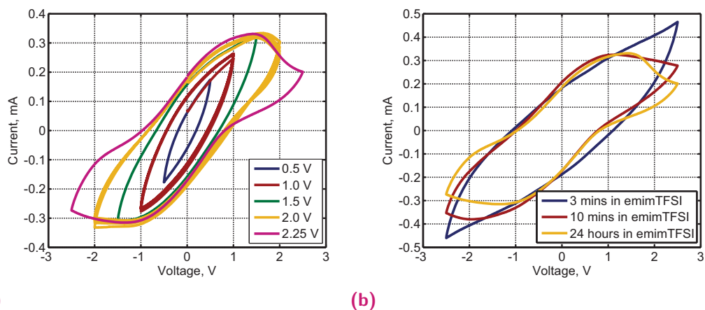
Fig. 4.10. Cyclic voltammograms of the PEDOT:PSS/mPVDF/ILs trilayer actuators in air recorded in two electrode set-up ( 100\text{ mV/s} scan rate) (a) measured up to different voltages 5 consequent cycles are shown for cyclic voltammetry (CV) up to 1 V and 2 V showing the stability in time. (b) CV of the PEDOT:PSS/mPVDF/ILs actuators after different incubation in ionic liquid times.
