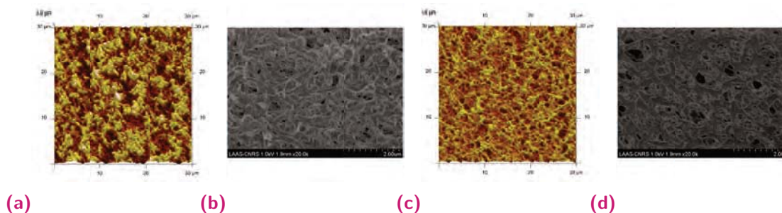
Fig. C.11. AFM and SEM images of surfaces of the pristine PVDF membrane. (a)-(b) - rough side (Rq - 351 nm) (c)-(d) - smooth side (Rq - 182 nm)
