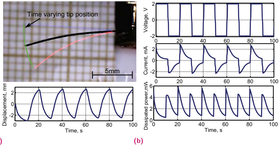
Fig. 4.8. (a) Merged images of the actuator at its extremities during actuation applying square wave with frequency of 50\text{ mHz} and 2.0\text{ V} amplitude. Blue and red actuators show its maximum and minimum displacement position, green dots show the tip position calculated from recorded videos. Actuator displacement profile in time is shown in the figure below. Actuator is bending towards the negative electrode. (b) Applied voltage, current and power dissipation measured during the actuation.
