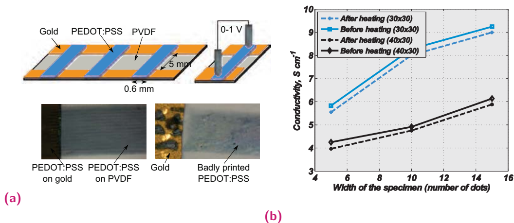
Fig. A.5. (a) Illustration of the setup used for the electrical conductivity measurements of inkjet printed lines and example of well and badly printed rectangulars. (b) Influence of the width of the line on calculated conductivity of printed PEDOT:PSS as well as the influence of printing resolution (indicated in legend).
