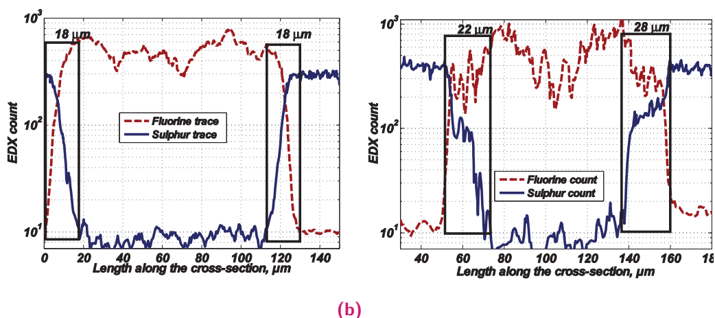
Fig. 2.9. EDX sulphur (blue) and fluorine (red) line scans across the cross-section of the PEDOT:PSS/PVDF-graft-PEGMA/PEDOT:PSS trilayers, where PEGMA was deposited on PVDF by (a) dipping and filling the pores, (b) spray coating.
