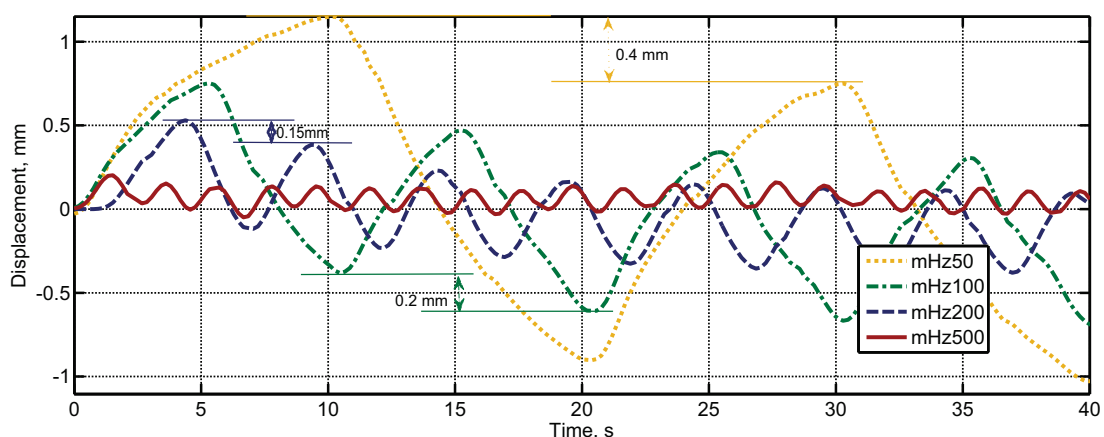
Fig. B.7. Bending profile of a trilayer actuator in time at different frequencies (indicated in the legend). Square voltage wave of 2\text{ V} was used for actuation. The level of the irreversible expansion causing creep is indicated with arrows.
