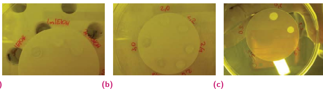
Fig. A.1. Pictures of drops of ethanol-water mixtures with different ratios (indicated next to the drop in red) on pristine PVDF membrane. (a) 1 – 3 vol%, (b) 2 – 3 vol%, (c) same as (b) but picture taken from below.
