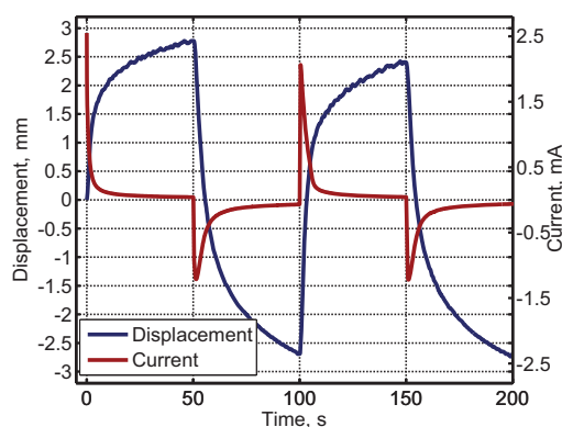
Fig. B.12. Displacement (blue) and transferred current (red) profiles of the (a) trilayer actuator made with PEDOT:PSS doped with 5 vol% PEG400 electrodes (infiltrated through and percolated), (c) A5 actuator and (d) trilayer actuator made on completely hydrophilized PVDF membrane (also infiltrated though and percolated). 2 V square wave at 10 mHz was used for actuation. (b) CV voltammograms of the actuator with the percolated electrodes (with 5 vol% PEG400) obtained during scans at 100 mV/s until different voltages.
