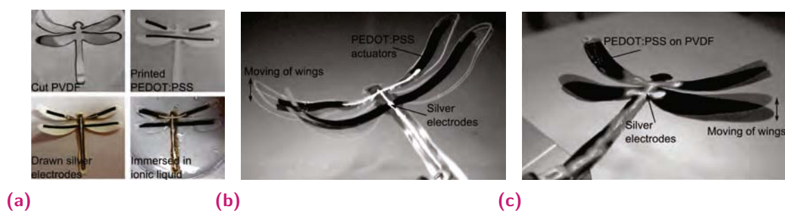
Fig. 5.9. (a) Fabrication steps for printed actuators: (1) PVDF membrane of wanted shape is cut; (2) PEDOT:PSS rectangular actuators were printed on each side of the membrane in the place where actuation was desired; (3) silver paste electrodes are drawn to connect different electrodes; (4) PVDF is impregnated with ionic liquid. Merged images of two actuation positions ( +/- 2 V at 1 Hz ) of dragonfly with (b) printed actuators and (c) actuators produced by drop casting and cutting.
