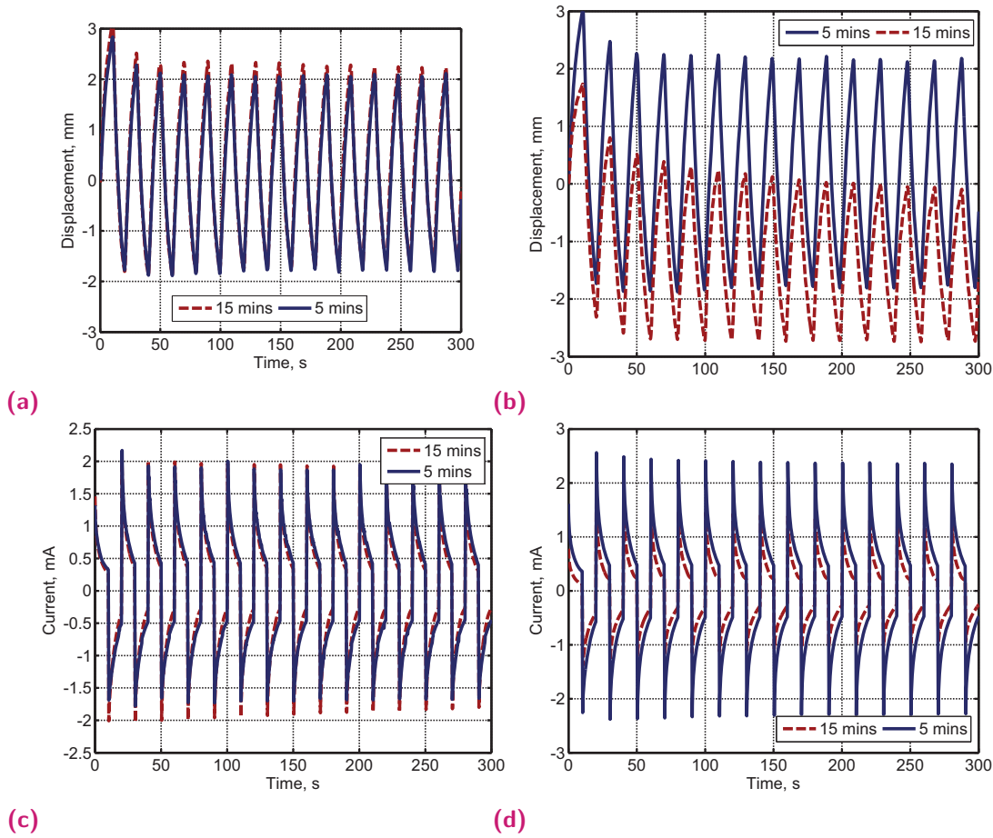
Fig. B.8. Displacement ((a)-(b)) and transferred current ((c)-(d)) profiles of the same actuator after 5 (blue) and 15 (red) minutes in the ionic liquid. (a,c) Both PEDOT:PSS layers are fine, (b,d) one of the PEDOT:PSS electrodes damaged during handling making the electrode very asymmetrical for the second measurement. 2 V square voltage wave was used for actuation at 50 mHz
