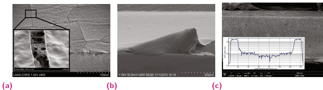
Fig. 5.4. (a) SEM of one pure PEDOT:PSS layer printed on PVDF membrane cracked after drying, (b) SEM of 10 PEDOT:PSS layer having 10 vol% glycerol printed on PVDF membrane showing easy delamination caused by handling and (c) SEM image of the cross-section of PEDOT:PSS/PVDF/PEDOT:PSS trilayer, when surfactant (1 vol% Triton-X100) was added to PEDOT:PSS ink. Inset: EDX line scan along the cross-section, indicating PEDOT:PSS abundance through the PVDF membrane.
