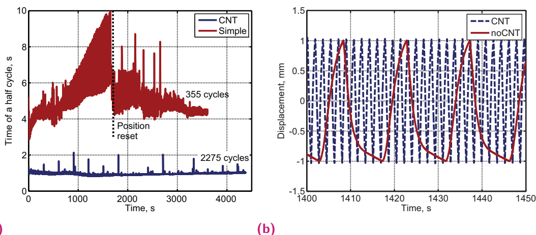
Fig. 4.20. (a) The change in the actuation frequency in time for the CNTs (blue) and simple (red) actuators measured as a time needed to move from/to \pm 1 mm. \pm 1.5 V was used to change the direction of bending as soon as the actuator tip reached set value. For actuator without CNTs the value was reset to +1.2 - -0.8 mm due to the large creeping (shown as dotted line). (b) Bending profiles in time for actuators with (blue dotted line) and without (red line) CNTs carpet. The voltage polarity ( \pm 1.5 V) was changed everytime the actuator reach the set \pm 1 mm value.
