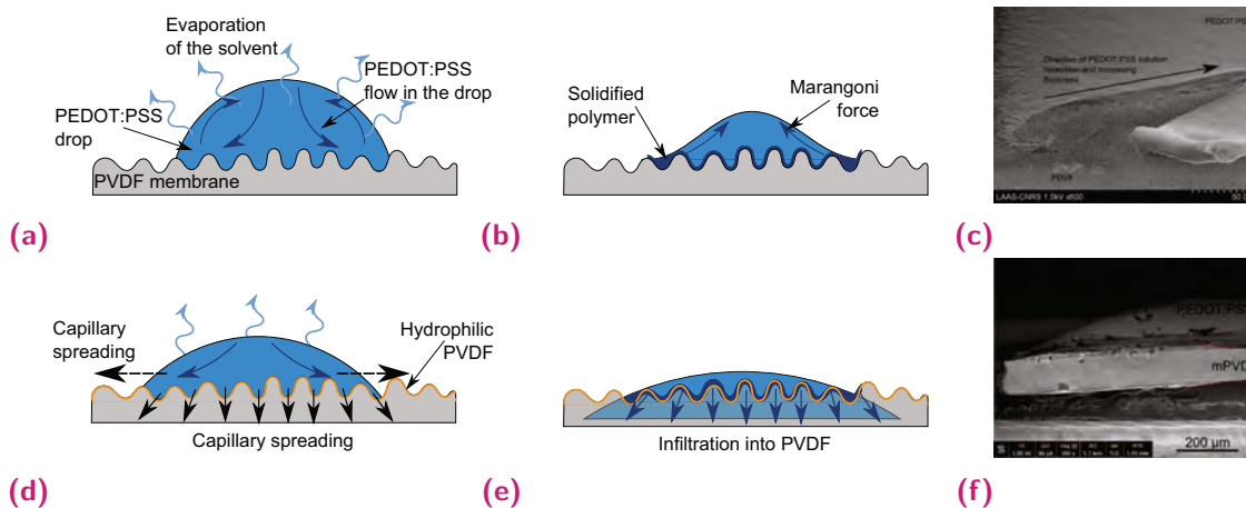
Fig. 5.5. Schematic illustration of some substrate-ink interactions, when (a)-(b) hydrophobic or (d)-(e) hydrophilic membrane is used as a substrate. SEM pictures of PEDOT:PSS printed on the (c) hydrophobic and (f) hydrophilic PVDF membranes.
