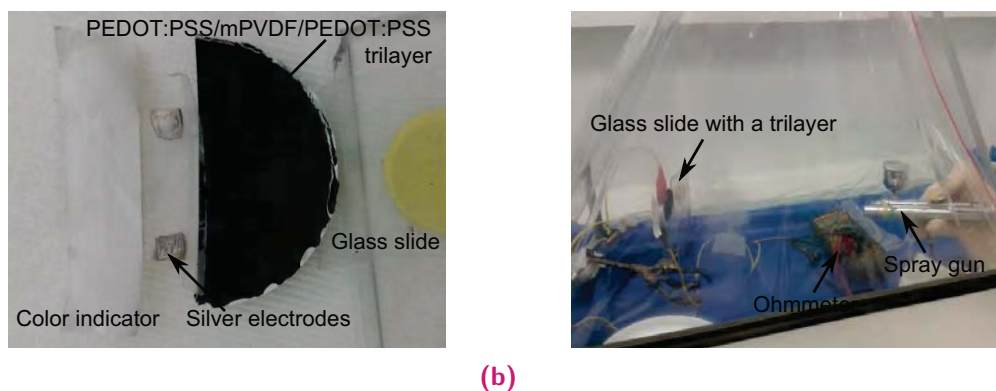
Fig. A.4. (a) Picture of PEDOT:PSS/mPVDF/PEDOT:PSS trilayer attached on the glass slides next to silver electrodes. (b) Picture of the set-up used for spraying carbon nanotubes.
