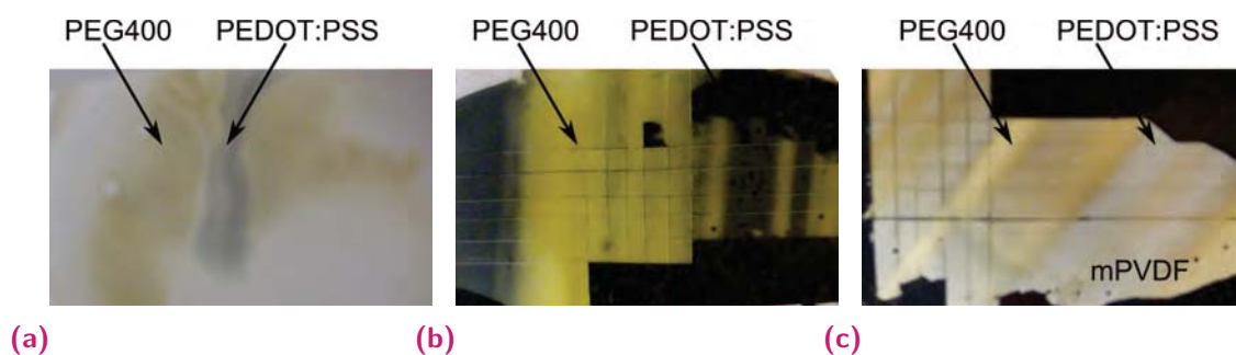
Fig. 3.15. (a) Back side of the membrane 24 hours after deposition of pegPEDOT (with 5 vol% PEG400). Penetrated PEG400 is visible as yellow and PEDOT:PSS as black marks. (b) PEDOT:PSS/pPVDF/PEDOT:PSS (with 5 vol% PEG400) trilayer after upper PEDOT:PSS layer is removed. The part of the PVDF membrane filled with mainly PEG400 is visible in yellow, part infiltrated with PEDOT:PSS is visible as black. (c) PEDOT:PSS/mPVDF/PEDOT:PSS (with 2 vol% PEG400) trilayer after upper PEDOT:PSS layer is removed. Yellowish surface shows mainly PEG400 on the PVDF (pores not completely filled - membrane is not translucent), black areas probably correspond to PEDOT:PSS infiltrated mPVDF.
