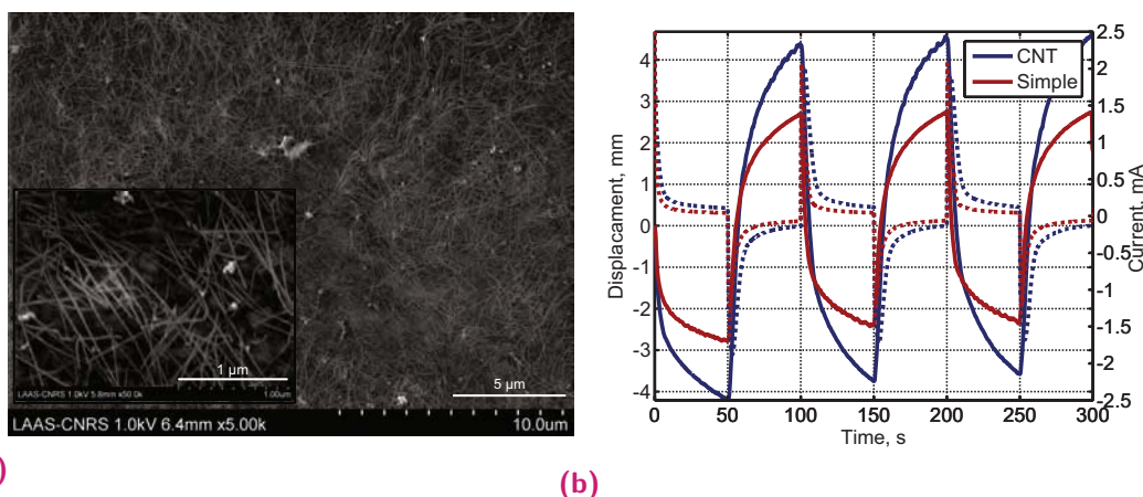
Fig. 4.19. (a) SEM image of the PEDOT:PSS electrode surface with sprayed CNTs carpet. (b) Displacement (solid line) and transferred current (dashed line) profiles of the actuators with (blue) and without (red) carbon nanotube carpet. Actuation with the square voltage wave of \pm 2V and 10\text{ mHz} was used for actuation.
