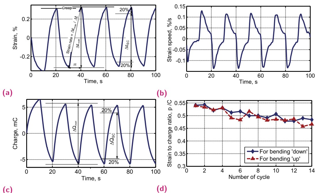
Fig. 4.9. (a) Actuator bending profile shown as calculated strain versus time. Strain is calculated using Equation 4.3 for every point detected during video processing. Min to max strain ( \Delta\epsilon_{max} ) is defined as strain difference between extremities during one actuation period ( T ), strain rate is a ratio of ( \Delta\epsilon_{max} ) and T/2 . (b) The speed of the actuator is calculated at every point as \delta\epsilon/\delta t . (c) Transferred charge calculated from the measured current during the actuation. The measures are equivalent to (a). (d) Strain to charge ratio calculated for each period separately for an actuator moving towards the positive ('up') and negative ('down') electrodes. The \Delta\epsilon_{SC} and \Delta Q_{SC} used for calculation are shown in (a).
