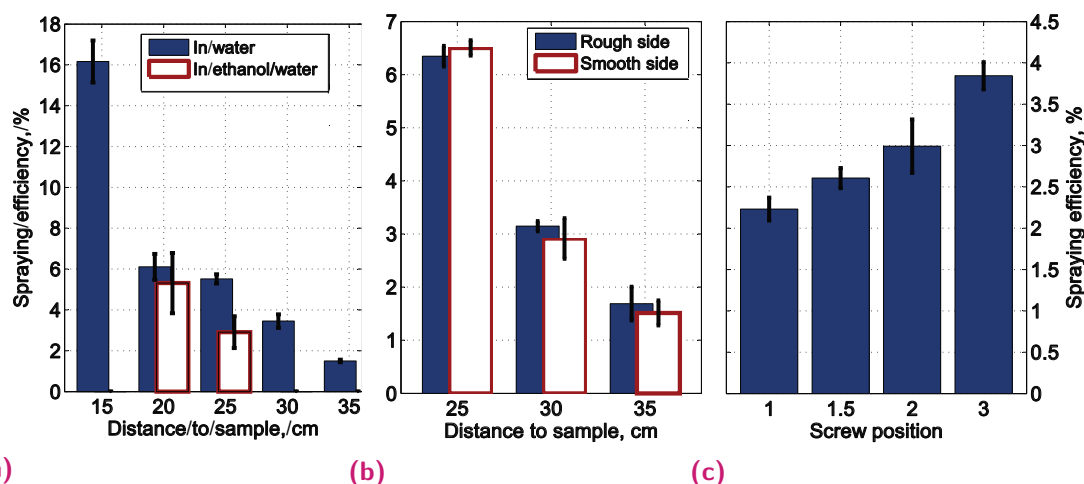
Fig. 2.10. Spray efficiency of PEGMA in ethanol/water solution on PVDF membranes with different spray parameters
