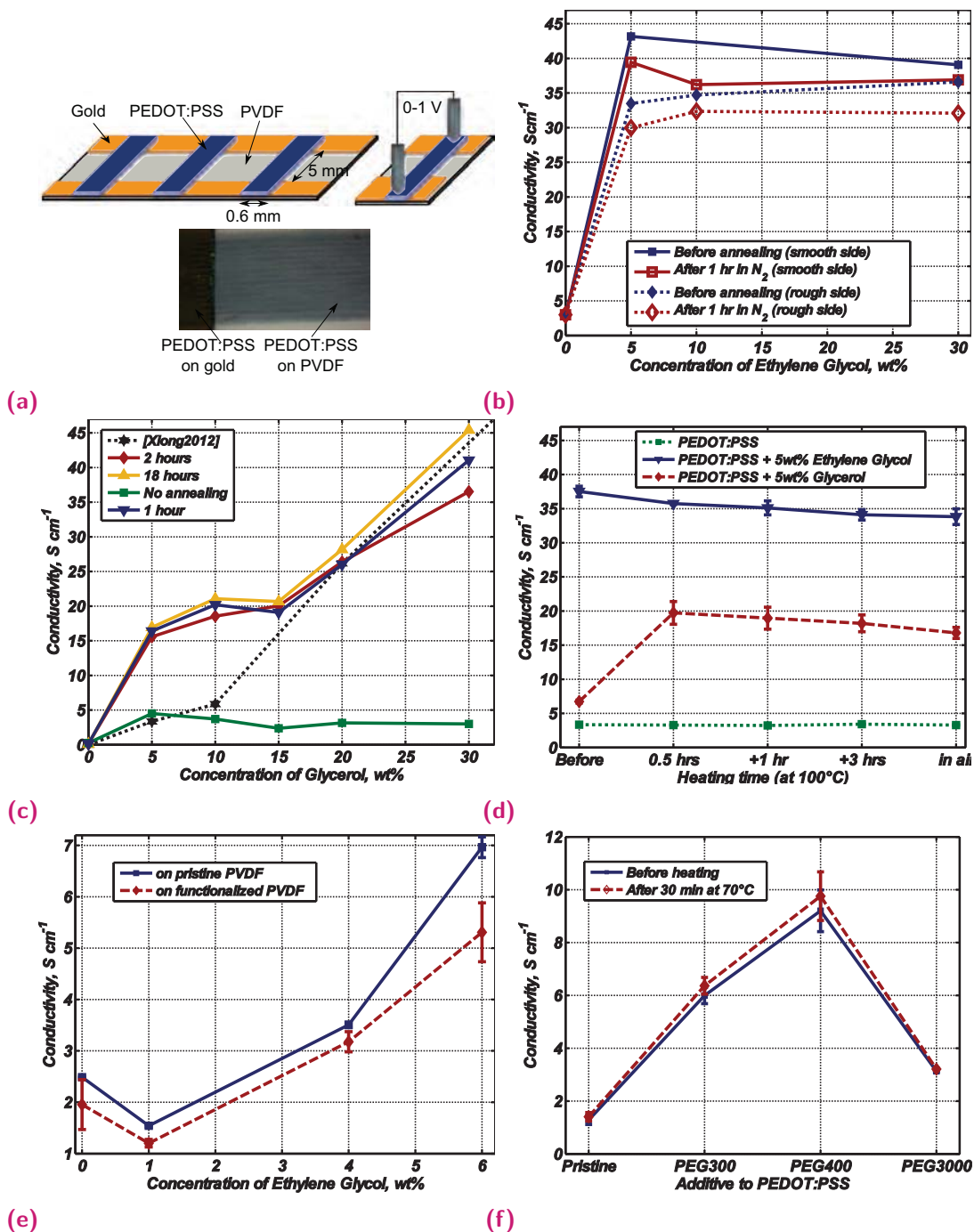
Fig. 5.7. (a) Schematic illustration of the set-up for conductivity measurement. 10 lines of PEDOT:PSS with 40 \times 40 \mu\text{m} resolution were printed on the PVDF membrane in between two sputtered gold electrodes. Picture of the printed film on the membrane and the electrode is shown below. The lines were cut and the resistance of the electrodes was measured. The conductivity was calculated assuming dimensions of 0.6 \text{ mm} \times 5 \text{ mm} \times 500 \text{ nm} . Conductivity of PEDOT:PSS secondary doped with different amounts of (b) ethylene glycol or (c) glycerol before and after thermal annealing. Annealing conditions are indicated in the legend. Films were printed on the smooth side of pristine PVDF membrane (pPVDF) unless indicated differently. Conductivity of G-PEDOT reported by [403] is plotted as a black dotted line. (d) Summarized influence of thermal annealing on conductivity of PEDOT (green dotted line) EG-PEDOT (red dashed line) and G-PEDOT (blue line). (e) EG-PEDOT with 5 vol% of Triton-X100 printed on the pristine (blue line) and functionalized (red dashed line) PVDF membrane. (f) Conductivity of PEDOT secondary doped with 1 vol% of PEG of different molecular weights and printed on functionalized PVDF membrane. Thermal annealing conditions are indicated in the legend.
