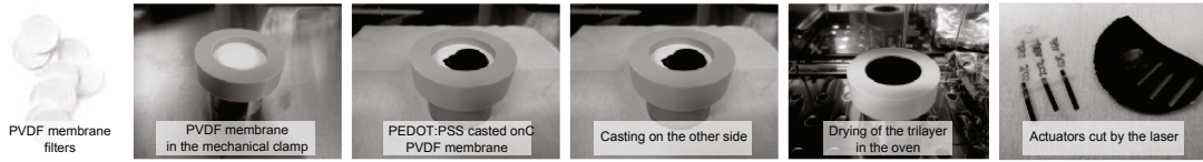
Fig. A.2. Pictures of the main fabrication steps of PEDOT:PSS/mPVDF/PEDOT:PSS actuators. Functionalized as in Section A.2 PVDF membranes were used. Membrane was then fixed in a metal mechanical clamp and 3 ml of PEDOT:PSS solution was drop casted on one side. After drying in air for about 24 hours, PEDOT:PSS was deposited and dried on the opposite side of the membrane. Then membrane with PEDOT:PSS on both sides was dried in oven at 70°C for 2 hours, occasionally reversing the clamp. After drying rectangular shaped actuators were cut with CO 2 laser. Actuators were immersed in ionic liquid before characterization (not shown).
