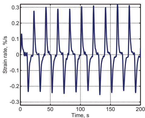
Fig. B.18. (a) Strain rate profile of printed actuator (10 layers on each side resulting in 3.35 mg of printed PEDOT:PSS . Actuated with 1.5 V, 50 mHz square voltage wave.). (b) Strain and transferred charge profiles of the same actuator.
