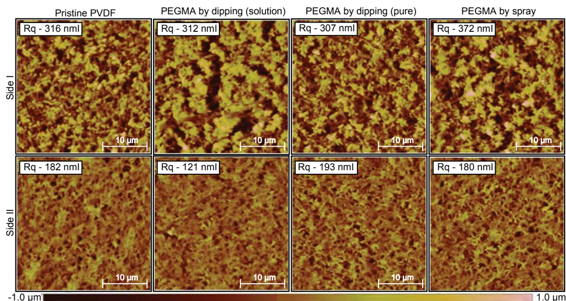
Fig. 2.8. AFM surface scans of the two sides of the pristine and functionalized membranes. PEGMA deposition method is indicated above.
