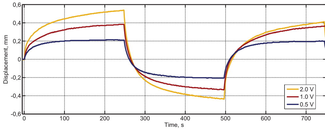
Fig. B.3. Trilayer actuator bending profiles during actuation with low frequency ( 2\text{ mHz} ) voltage square wave. The voltage used is indicated in the legend.
