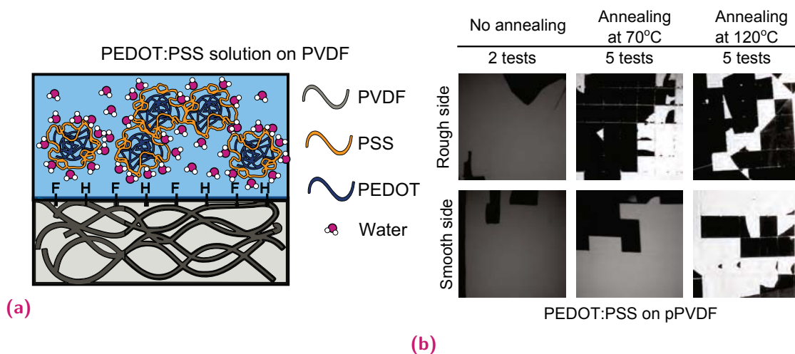
Fig. 3.4. (a) Illustration of PEDOT:PSS core/shell structured nanoparticles in aqueous solution with PEDOT chains in the core (blue) and PSS around (yellow). The hydration shell on PSS presumably prevents the polymer adsorption on the PVDF (grey) surface. (b) Pictures of the remaining PEDOT:PSS films (black) on the PVDF membrane (white) surface (rough and smooth) after adhesion tests. The annealing condition and the number of tests performed before taking the picture is indicated above.
