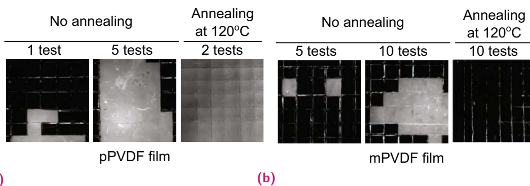
Fig. 3.11. Adhesion tests of PEDOT:PSS (with 1 vol% PEG400 ) and flat PVDF films in a dry state. Annealing condition and the number of adhesive tape applications is indicated above each picture. Type of the film is indicated below ( mPVDF - functionalized film, pPVDF - pristine film).
