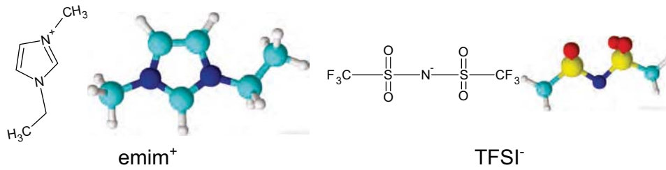
Fig. C.4. Chemical and 3D structures of the ionic liquid 1-Ethyl-3-methylimidazolium bis(trifluoromethanesulfonyl)imide (emimTFSI)
