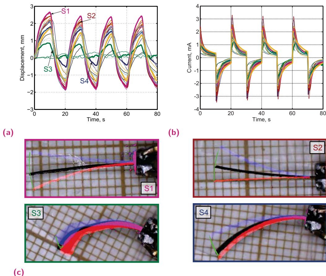
Fig. 4.14. (a) Displacement and (b) current versus time of various actuators made with or without post-treatment from four different membranes. Actuators made with the equivalent fabrication procedure are represented by the same colour. Performance versus other parameters of the same actuators are plotted in Fig. B.10, special cases shown with a thicker line, correspond to the filled markers. (c) Merged images of the several actuators at the initial (black) and extremities during actuation (red and blue). All measurements were recorded during actuation by 1.5 V and 50 mHz square wave.
