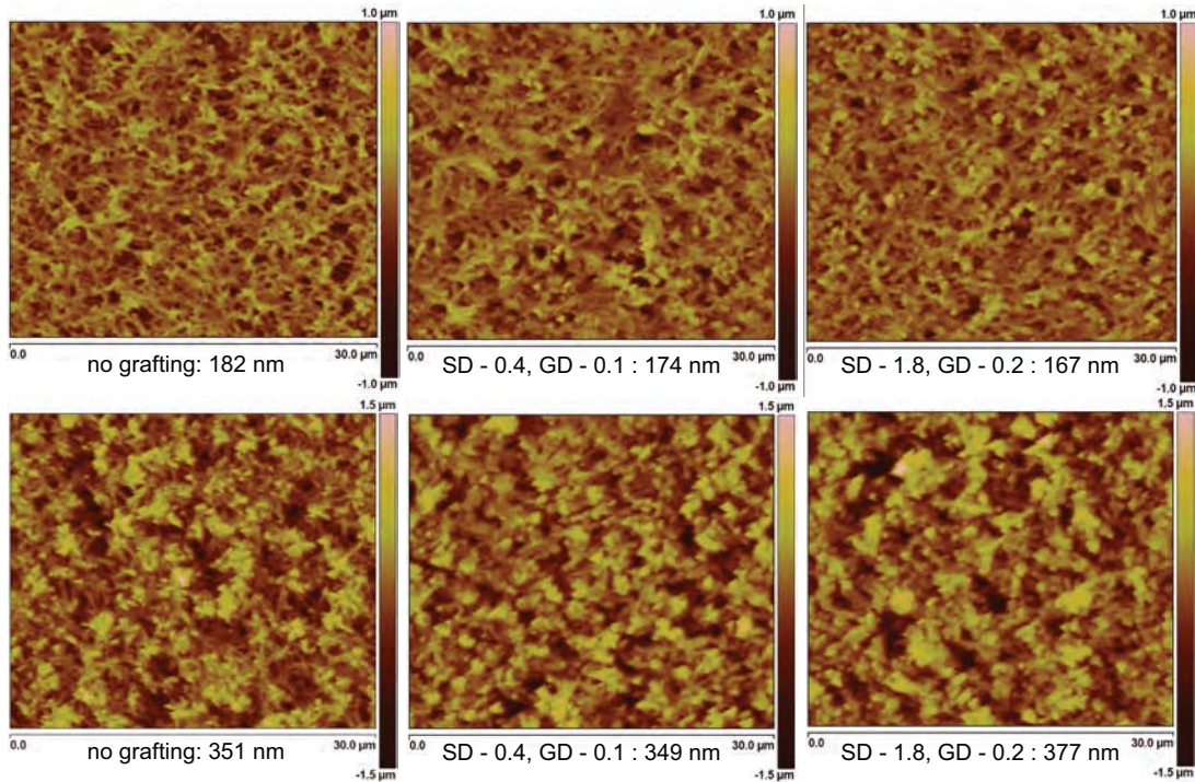
Fig. B.1. AFM surface scans of membranes functionalized with different amount of PEGMA. Measured surface roughness and the spray and graft densities are indicated below.
