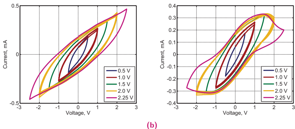
Fig. B.5. Cyclic voltammograms of the trilayer PEDOT:PSS/mPVDF/PEDOT:PSS actuators obtained with 100\text{ mV/s} scan rates and different voltages indicated in the legend. The actuators were kept in the ionic liquid for (a) 3 minutes or (b) 24 hours.
