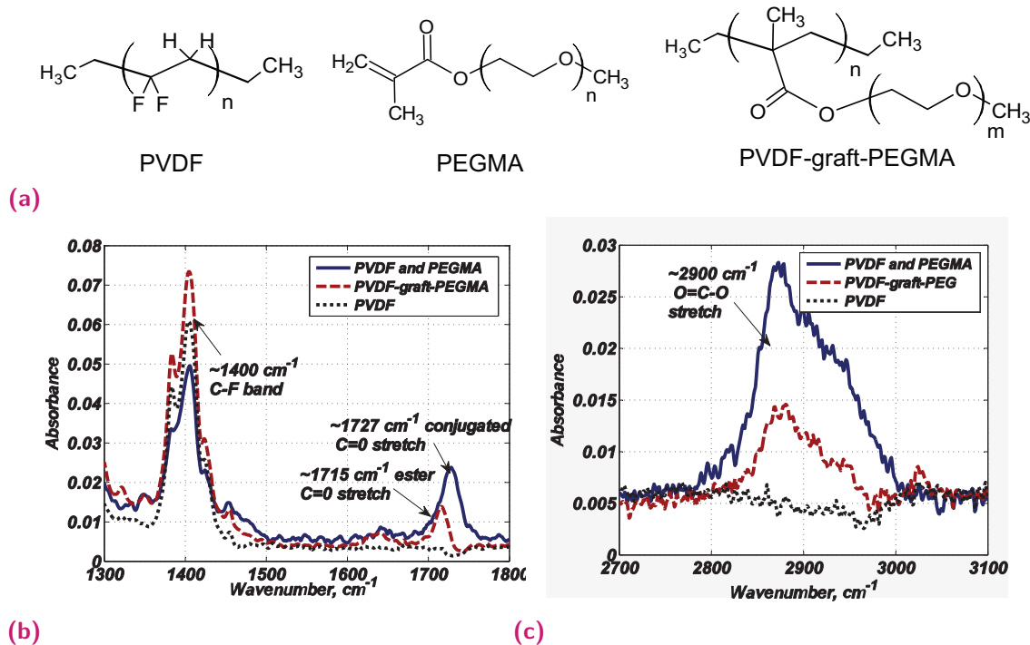
Fig. 2.4. (a) Chemical structure of PVDF, PEGMA and PVDF-graft-PEGMA and their IR signatures between (b) 1300 - 1800 \text{ cm}^{-1} and (c) 2700 - 3100 \text{ cm}^{-1}
