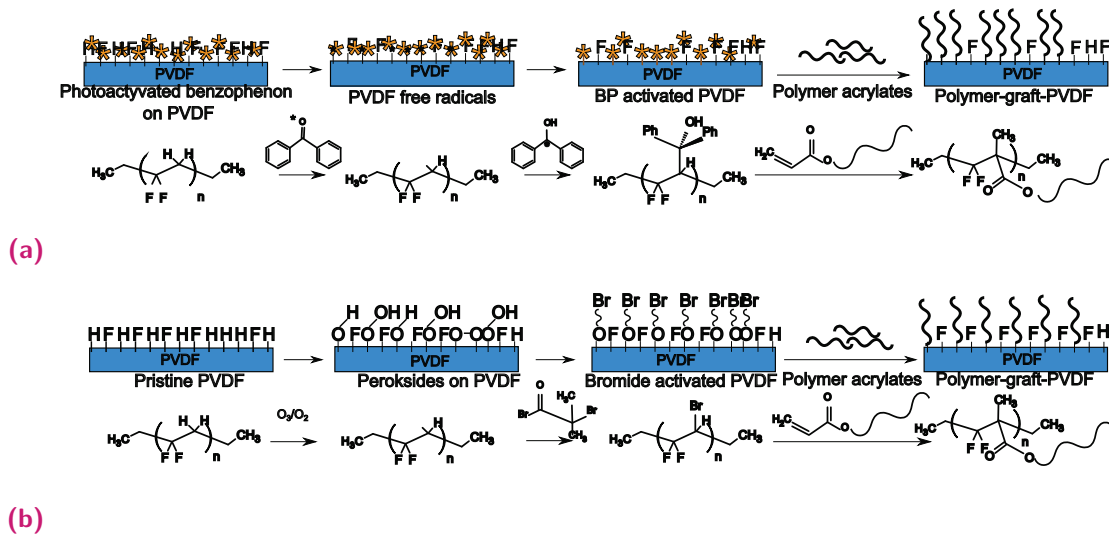
Fig. 2.1. Scheme and example of the grafting-to reaction of acrylate to PVDF membrane by (a) UV irradiation and (b) atom transfer radical polymerisation
