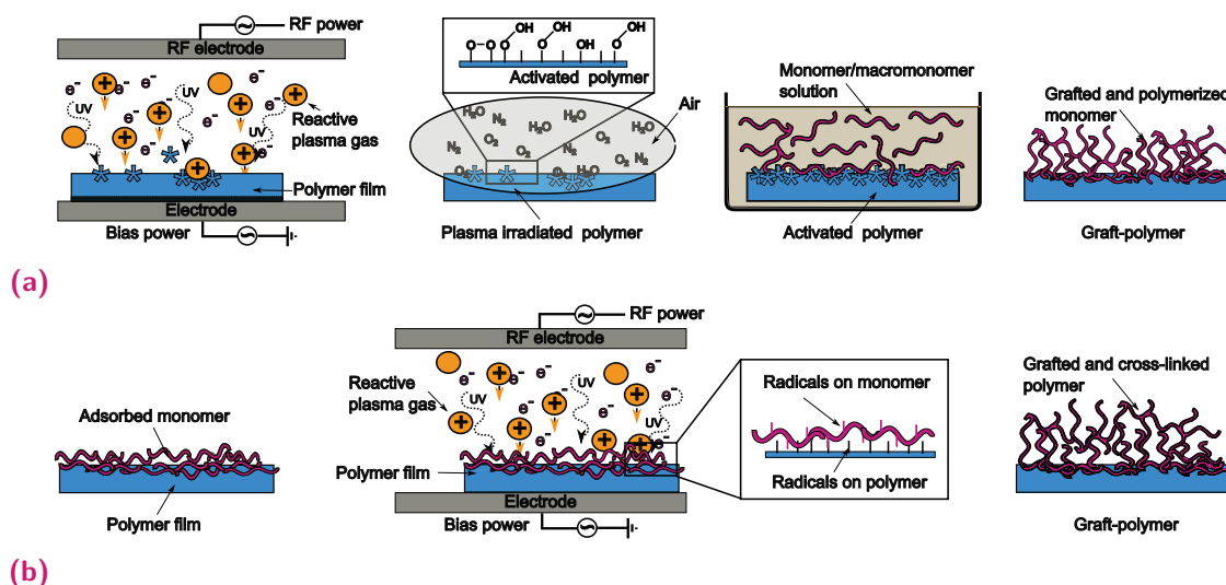
Fig. 2.3. (a) (1) Generation of radicals on the surface of the polymer film by plasma irradiation; (2) activation of the polymer surface with oxygen moieties during the exposure to the air; (3) incubation of the activated polymer in the solution containing polymer-to-be-grafted monomer or macromonomer. (b) (1) Immobilization of the monomer or macromonomer on the surface of the substrate; (2) activation of both: the polymer surface and monomer precursor by plasma creating radicals on both; (3) simultaneous reaction between active species: anchoring of the reaction precursor to the substrate and cross-polymerization.
