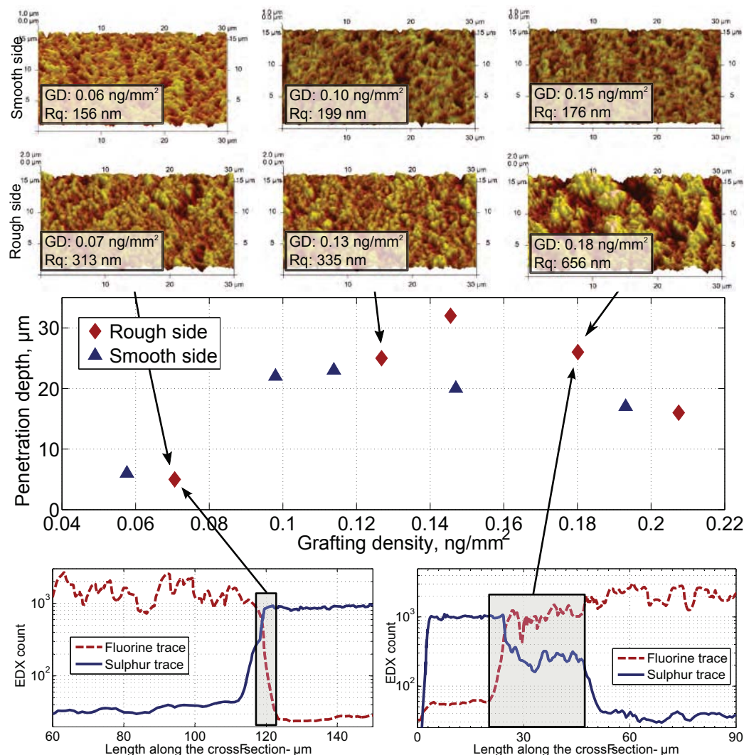
Fig. 2.13. (Bottom) EDX line scans for sulphur (blue full line) and fluorine (red dashed line) along the cross-sections of PEDOT:PSS/PVDF-graft-PEGMA with the GD indicated with the arrows. (Centre) The length of the depth of mixing versus the grafting density ( GD ) plotted separately for PEDOT:PSS deposited on the smooth side (blue \triangle ) and the rough side (red \diamond ) of PVDF-graft-PEGMA . (Top) AFM images of the rough and smooth surfaces of the PVDF-graft-PEGMA membranes with different grafting densities ( GD ). Grafting density and the roughness are indicated in the legends.
