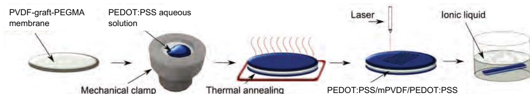
Fig. 4.5. Illustration of a fabrication process flow for a solvent casted actuators. Hybrid PVDF-graft-PEGMA ( mPVDF ) membranes are clamped mechanically in an aluminium holder and PEDOT:PSS aqueous solution (secondary doped) is deposited by drop-casting. After drying at room temperature, the clamp is reversed and the procedure is repeated for the another side of the actuator in order to produce the trilayer. Membrane with PEDOT:PSS on both sides is then dried in the oven at 70°C for 2 hours. 1.5 mm x 2 cm rectangular actuators are then cut by a laser, actuators are thermally annealed at 120°C (not shown) and are incubated in ionic liquid for 10 – 120 minutes.
