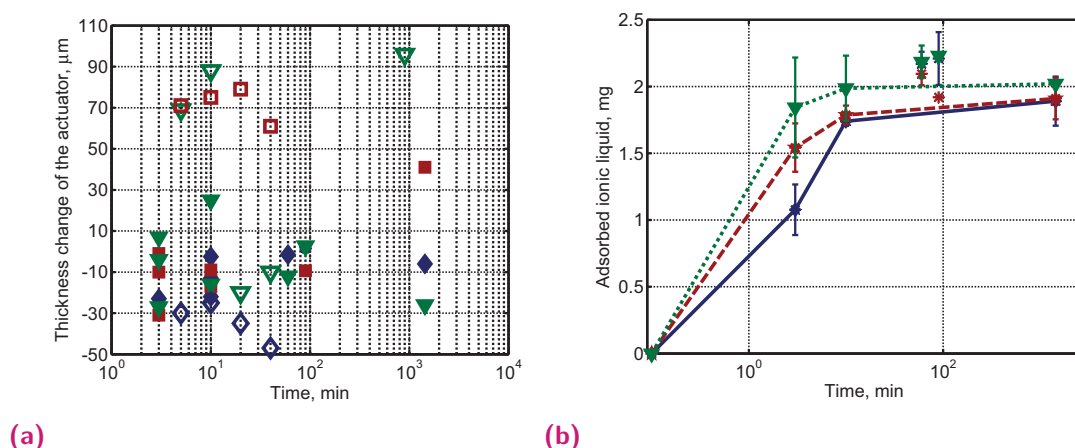
Fig. 4.7. (a) Difference of the thickness of the actuators and (b) increase in the actuators weight after different times of incubation in emimTFSI . Actuators produced on the membranes with GD 0.16 \pm 0.003 , 0.11 \pm 0.002 and 0.046 \pm 0.018 ng/mm^2 were corresponding to mixing depths of < 5 \mu m (green dotted line), 30 \mu m (blue line) and 25 \mu m (red dashed line) respectively. Thickness measurements done after incubation in ILs and 5 mins cycling with 2 V square wave at 200 mHz are indicated with open markers.
