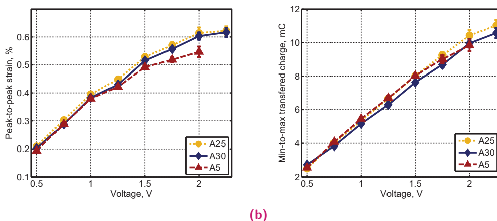
Fig. 4.16. (a) Peak-to-peak strain and (b) transferred charge for actuators with different mixing depth at different voltages.
