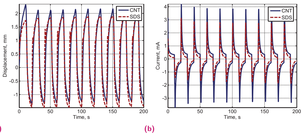
Fig. B.15. Displacement (a) and transferred current (b) profile of the actuators treated with CNT (blue) and with SDS (red). 1.5 V square voltage wave was used for actuation at 50 mHz .
