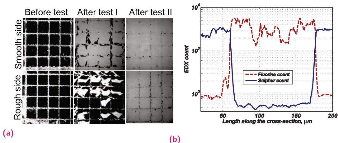
Fig. 3.6. (a) Pictures of the remaining PEG-PEDOT films (black) on the pPVDF membrane (white) surface (rough and smooth) after the adhesion test in a dry state (test I) and after incubation in ionic liquid for 24 hours (test II). (b) Energy-dispersive X-ray spectroscopy (EDX) scan along the cross-section of the pegPEDOT/pPVDF/pegPEDOT trilayer. The fluorine trace (signature of pPVDF) is shown in red (full line) and sulphur trace (signature of PEG-PEDOT) in blue (dashed line)
