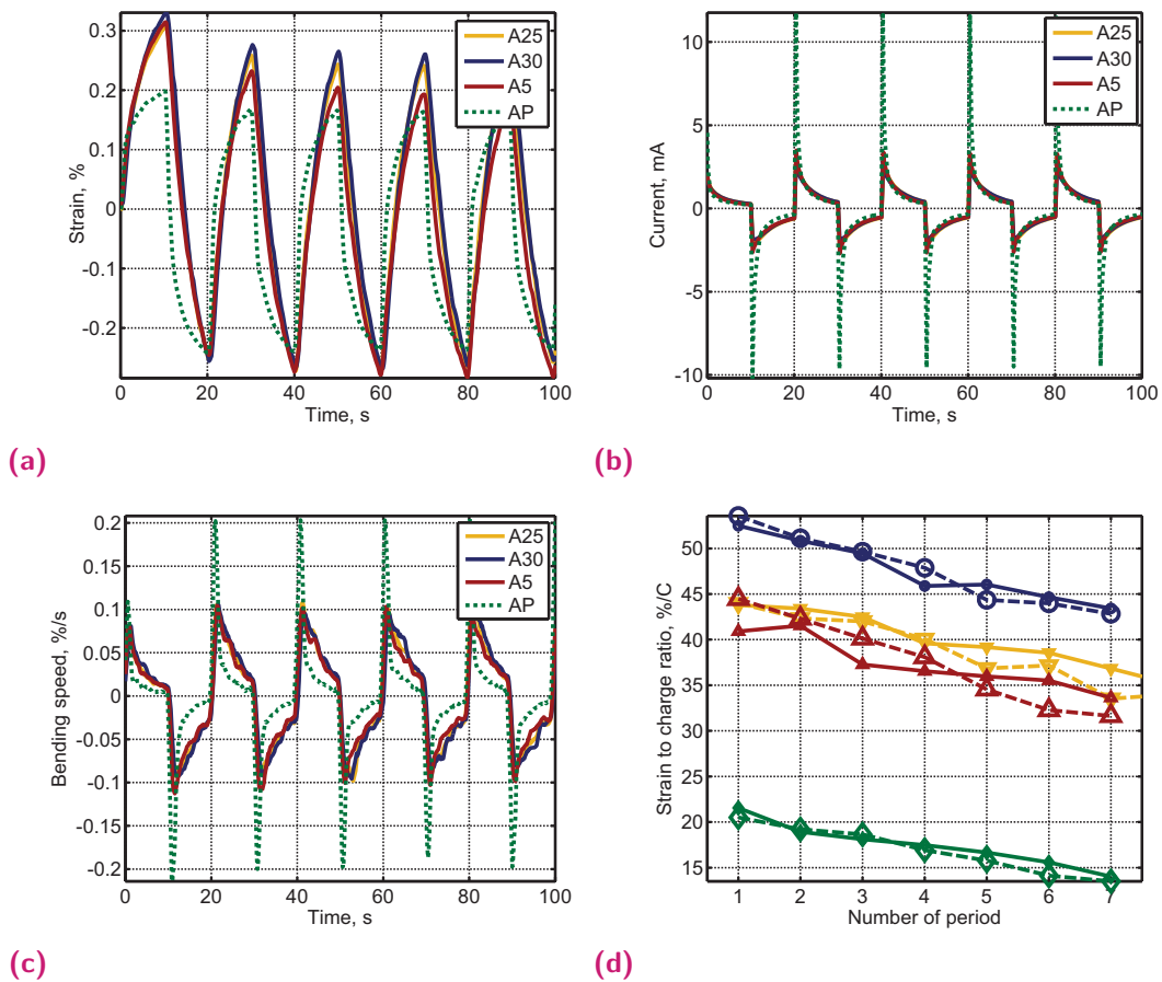
Fig. 4.15. (a) Strain and (b) transferred current and (c) bending speed profiles of the actuators having a different mixing depth (indicated in the legend as a number, AP - semi-trilayer with percolated electrodes (green dotted line)). 2.0 V square voltage wave at 50 mHz was used for actuation. (d) Calculated strain-to-transferred charge ratio for each cycle for different actuators (colors correspond to the legends in (a)-(c)). The ratio calculated for motion and upwards and downwards is plotted separately as dotted and full lines.
