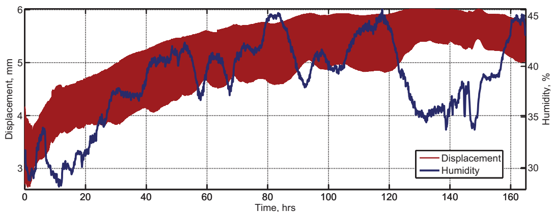
Fig. B.9. Displacement profile of the actuator during long time actuation. The ambient humidity is plotted as blue line. Square voltage wave of 1.5 V and 100 mHz frequency was used for actuation and the position was tracked with laser displacement sensor.
