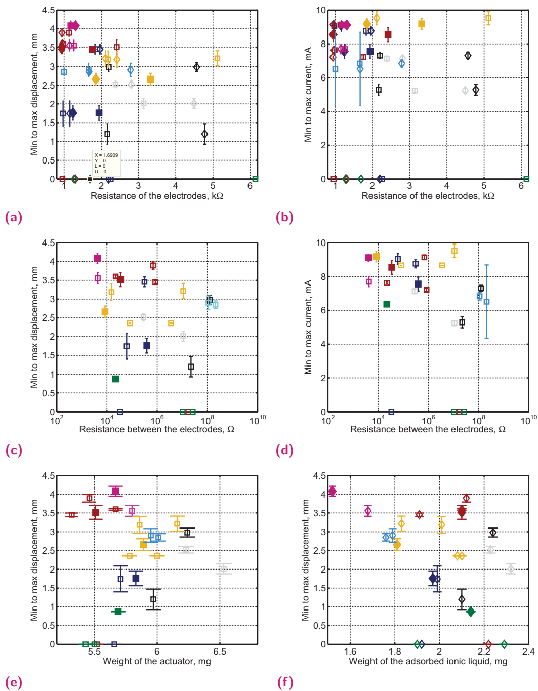
Fig. B.10. In order to identify factors affecting performance of the actuators, 4 PVDF membranes were functionalized in the equivalent way. Half of each membrane was then secondarily treated in order to create variety of resistances along the electrode and in between the electrodes as explained in Section A.4.3 (different amount of CNT , Ag nanowires, SDS were deposited by spray-coating on the surface). Peak-to-peak displacement ((a), (c)-(f)) and transferred current ((b), (d)) is plotted versus measured resistance along the electrode ((a)-(b)) and between the electrodes ((c)-(d)), weight of the actuator ((e)) and the amount of the adsorbed ionic liquid ((f)). Different batches are indicated in different colours. Filled markers represent the coloured displacement profiles and images of the actuators in the Fig. 4.14.
