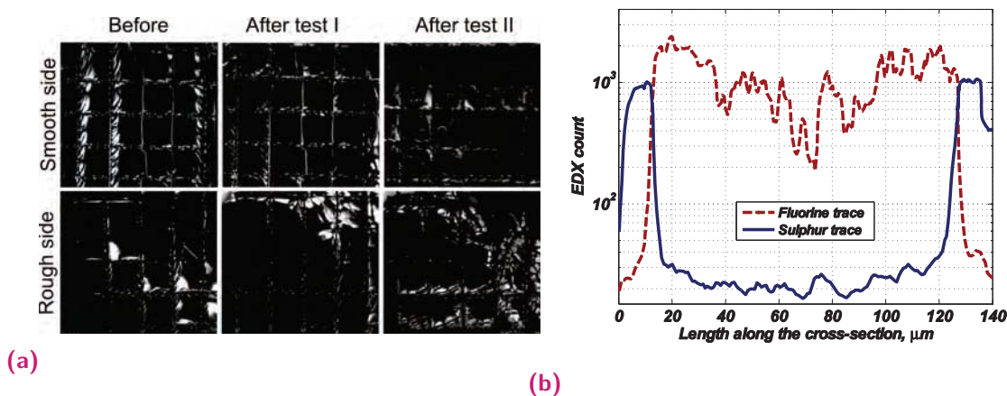
Fig. 3.10. Qualitative adhesion test of PVDF and PVDF-graft-PEGMA membranes and PEDOT:PSS. Pictures are taken before, after 5 Scotch™ Tape peeling tests (Test I) and 5 more peeling tests after incubation in ionic liquid for 48 hours (Test II)
