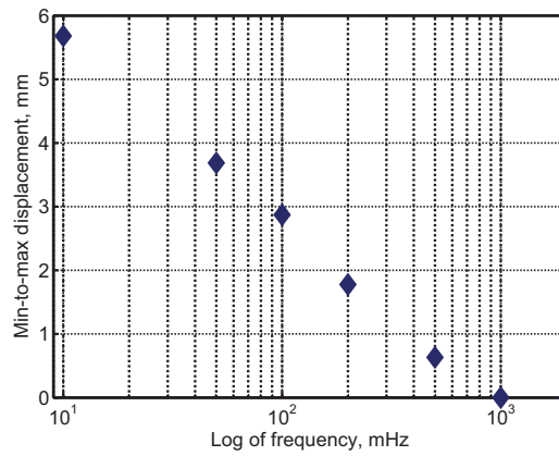
Fig. B.16. (a) Strain profile at different voltages and (b) frequency response of probably the best trilayer PEDOT:PSS/mPVDF/PEDOT:PSS actuator fabricated during our study.
