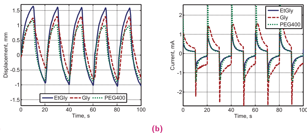
Fig. 4.17. (a) Bending and (b) transferred current profiles of the actuators with PEDOT:PSS electrodes that were secondary doped with 1 vol% of ethylene glycol (blue full line), glycerol (red dashed line) and standard PEG400 (green dotted line). 1.5 V square voltage wave at 50 mHz was used for actuation.
