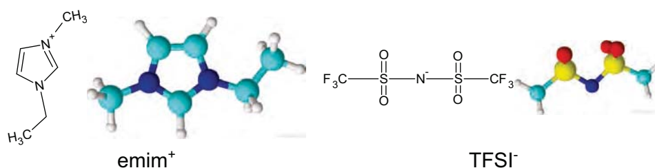
Fig. 4.4. Chemical and 3D structures of the ionic liquid 1-Ethyl-3-methylimidazolium bis(trifluoromethanesulfonyl)imide ( emimTFSI )
