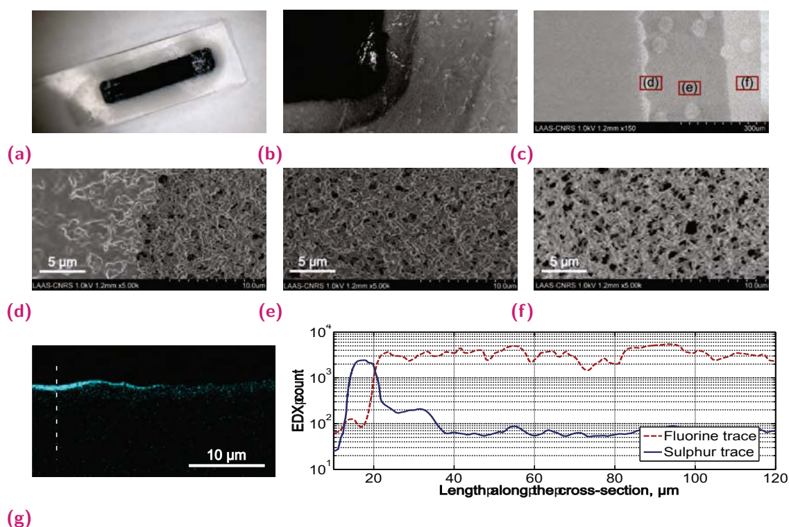
Fig. 5.6. (a) Picture of the PEDOT:PSS electrodes printed on PVDF membrane and PEDOT:PSS 'ring' on the surface after incubation in the ionic liquid. (b) Picture of the same actuator before immersion in ionic liquid showing two rings formed by PEDOT:PSS spreading on the surface. (c) SEM image of the edge of the printed actuator and the 'ring' (satellite droplets are also seen around the actuator (lighter rounds)), (d)-(f) shows enlarged areas of the membrane and different amounts of PEDOT:PSS on the surface. (e) EDX area and line scans along the cross-section of 10 layers of PEDOT:PSS printed on PVDF-graft-PEGMA membrane ( mPVDF ). Sulphur trace is shown in blue. The approximate place of the line scan is indicated with the white dashed line.
