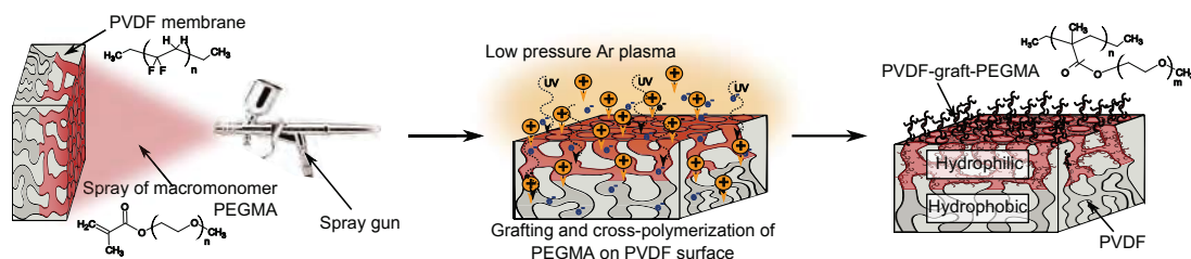
Fig. 2.14. Functionalization of PVDF membranes: deposition of reaction precursor (PEGMA) by spray coating only on the surface of the membrane and argon plasma induced grafting to PVDF backbone leading to hybrid hydrophilic-hydrophobic membranes.
