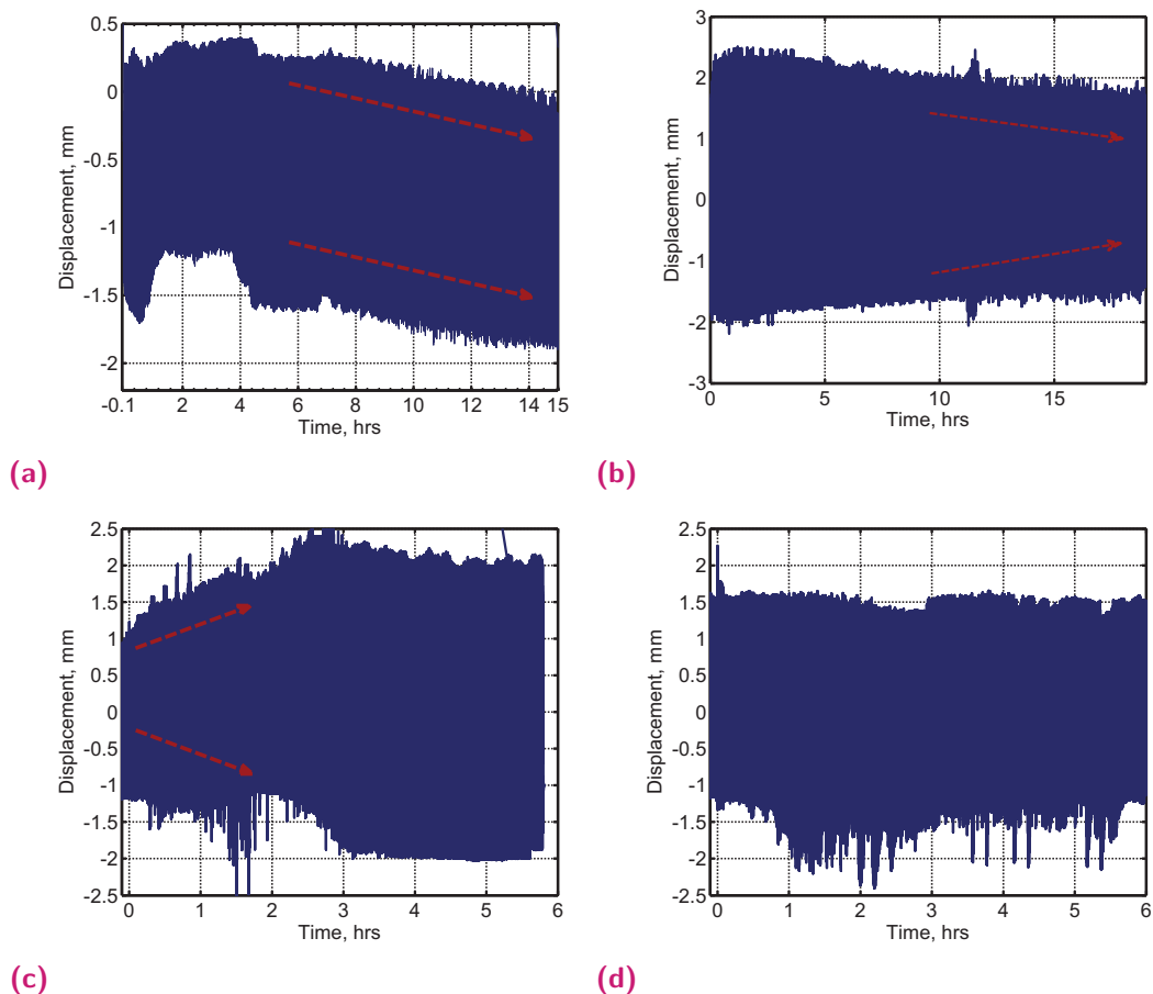
Fig. 4.11. (a) Actuation displacement profile of the PEDOT:PSS/mPVDF/PEDOT:PSS trilayer cycled in air with 2 V square wave with 100 mHz frequency. Significant creeping (indicated with red arrows) can be observed after 6 actuation hours. (b) Gradual decrease in the actuators displacement after 2 hours of actuation. Actuated with 1.5 V voltage sine wave with 50 mHz frequency. (c) Training effect (red arrows) shown during cycling of the actuator with 2 V square wave with 50 mHz frequency. The actuation profile of the same actuator after 20 hours in a static position is shown in (d)
