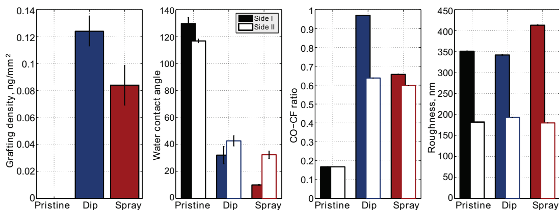
Fig. 2.7. Comparison of membranes prepared by filling the pores (dip) and spray coating (spray): (a) grafting density; (b) water contact angle; (c) integrated FT-IR OCO–CF ratio; (d) roughness of the membranes. Filled and empty bars indicate measurements on two sides of the membranes.
