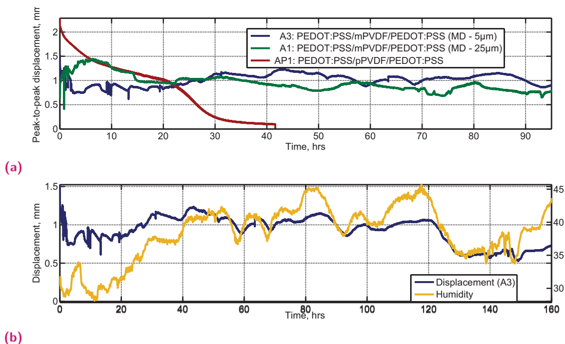
Fig. 4.13. (a) Lifetime measurement of actuators produced with hybrid PVDF-graft-PEGMA (mPVDF) and pristine membranes (PVDF). The mixing depth between PEDOT:PSS and mPVDF is indicated in the legend. (b) Amplitude of the displacement for PEDOT:PSS /PVDF-graft-PEG/ PEDOT:PSS with MD of 5\mu\text{m} based actuator in ionic liquid (blue) and the change in the humidity of the environment (yellow).
