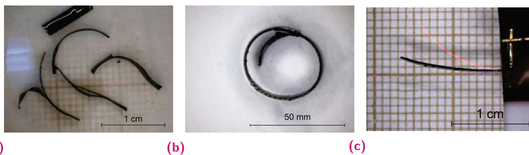
Fig. 4.12. (a) Picture of PEDOT:PSS/pPVDF/PEDOT:PSS actuators just after immersion in ionic liquid: adhesion is not strong enough and layers separate. If part of the PEDOT:PSS remain on the membrane, different expansion coefficients of the materials are causing bending and twisting of the rectangular. (b) Picture of PEDOT:PSS/mPVDF bilayer after immersion in ionic liquid: adhesion between materials is strong enough and due to difference in expansion of each material, bilayer roles into a cylinder. Nevertheless, adhesion is strong enough to sustain the stress at the interface. (c) Merged images of the trilayer actuator with a strong adhesion between layer at initial position (black) and at extremities during actuation (red and blue). Actuated with 2 V, 10 mHz square voltage wave.
