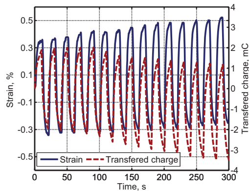
Fig. B.18. (a) Strain rate profile of printed actuator (10 layers on each side resulting in 3.35 mg of printed PEDOT:PSS . Actuated with 1.5 V, 50 mHz square voltage wave.). (b) Strain and transferred charge profiles of the same actuator.
