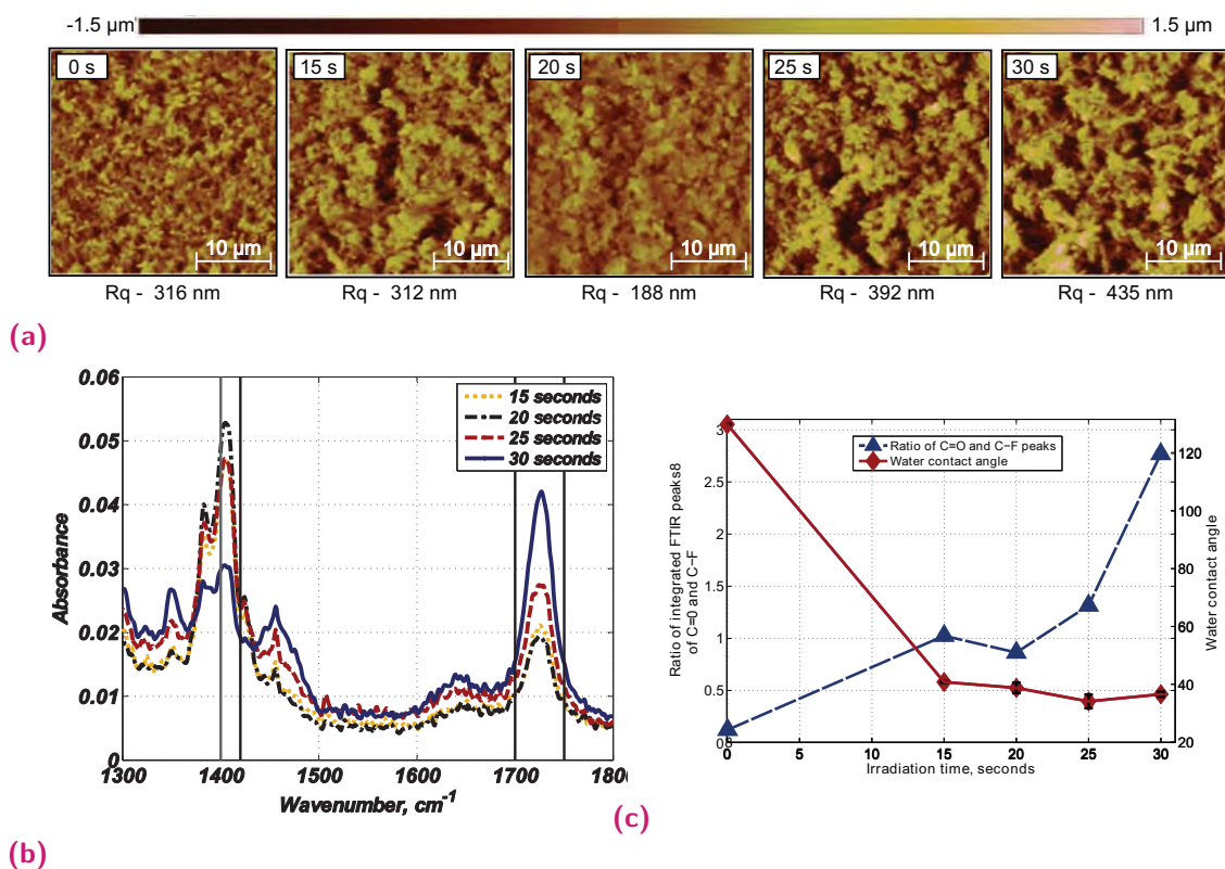
Fig. 2.5. (a) atomic force microscopy (AFM) surface scans of PVDF membranes after PEGMA grafting with different plasma irradiation times. Measured average roughness is indicated below. (b) FT-IR spectra of the same membranes and (c) Ratio of integrated OCO–CF FT-IR peaks (blue \triangle ) and measured water contact angle (red \diamond )
