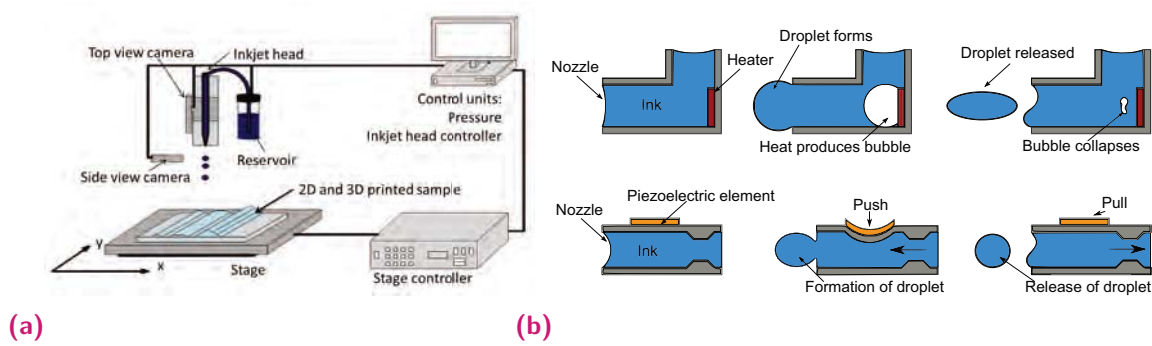
Fig. 5.1. (a) Schematic diagram of a drop-on-demand inkjet printer. (b) The schematic cycle of drop ejection in (above) thermal (rapid expansion and collapse of the bubble) and (below) piezoelectric (by direct mechanical deformation at typically 1 - 20 \text{ kHz} ) inkjet drop-on-demand printing.
