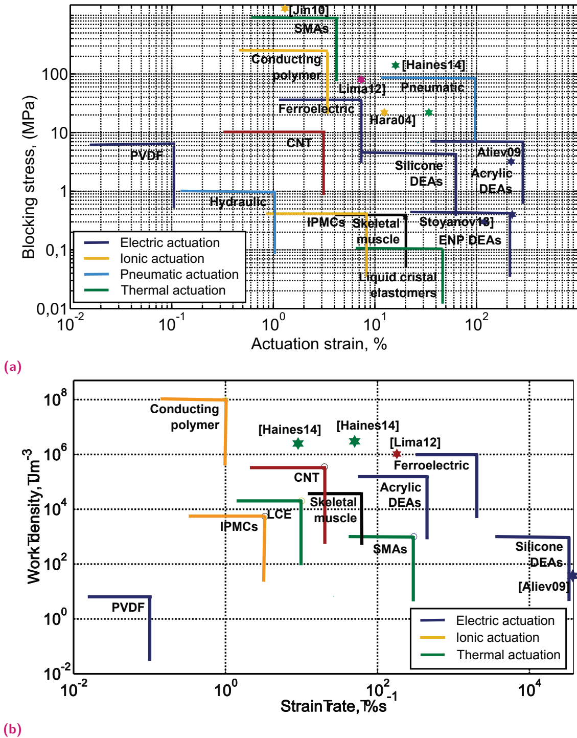
Fig. 1.1. (a) Stress versus strain and (b) work density versus strain rate of typical artificial muscles (defined by lines) and some state-of-the-art actuators (stars). Types of actuations: blue - electric, orange - ionic, green - thermal, red - CNTs, gray - others, black - mammal skeletal muscle. Adopted from [249, 269] and other sources mentioned in the text.
