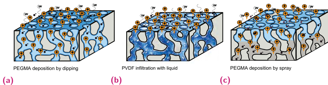
Fig. 2.6. Schemes showing three different precursor deposition strategies and subsequent plasma membrane interactions: (a) deposition by dipping in diluted solution leading to precursor adsorption on the surface of the membrane and subsequently activation and grafting by plasma throughout the thickness; (b) deposition by dipping in viscous liquid that prevents plasma gas diffusion and activation to the pores; (c) deposition by spraying that limits precursor deposition to a certain depth.
