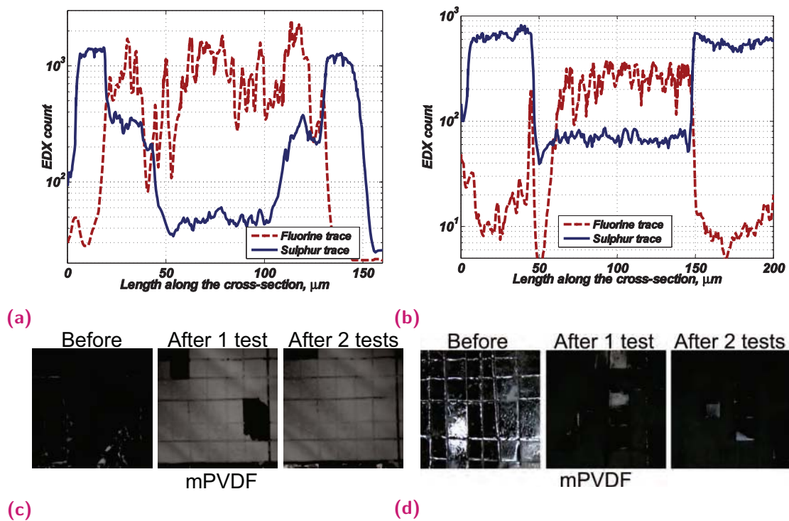
Fig. 3.14. EDX line scans for fluorine (red) and sulphur (blue) traces along the cross-section of the trilayers PEDOT:PSS/PVDF-graft-PEG/PEDOT:PSS (a)-(b) and adhesion tests of the PEDOT:PSS film deposited on the rough side of the functionalized membrane (c)-(d) For (a) and (c) PEDOT:PSS is secondary doped with 2 vol% PEG400, for (b) and (d) with 5 vol% PEG400.
