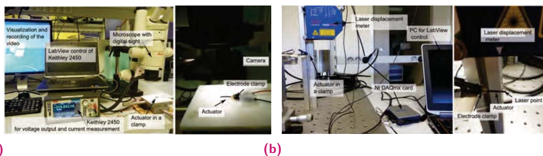
Fig. A.3. Picture of the experimental set-up used for bending characterization (a) by recording the bending and tracking the position of the tip and (b) by tracking bending using laser displacement meter.
