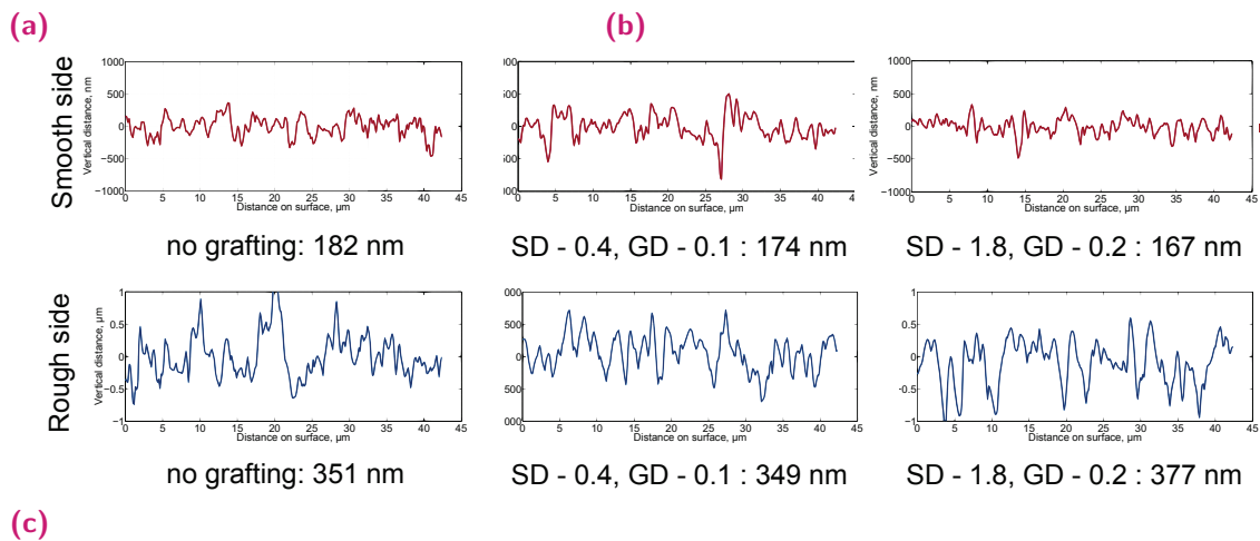
Fig. 2.12. (a) Ratio of integrated OCO and CF peaks of pristine (indicated with an arrow) and functionalized PVDF membranes versus sprayed amount of precursor (PEGMA) (blue \diamond - rough side, red \triangle - smooth side) and (b) Water contact angle of pristine PVDF (grafting density = 0 ng/mm 2 ) and PVDF-graft-PEGMA membranes at different grafting densities. (c) Topographic AFM measurements of the cross-sectional profiles of membranes with different grafting densities for the two sides.
