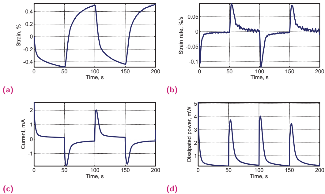
Fig. B.4. (a) Strain, (b) strain rate, (c) transferred current and (d) dissipated power profiles in time of a trilayer actuator, actuated with 2\text{ V} square voltage wave at 10\text{ mHz} .
