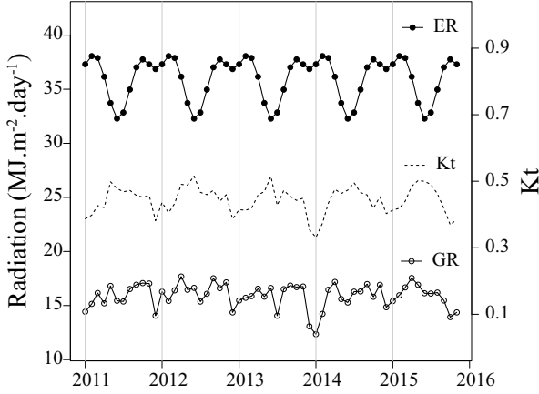
Figure III.4: Evolution of radiation in the Palembang region ( latitude = -2.99^\circ ). Left axis: extraterrestrial radiation (ER) and global radiation (GR); right axis: clearness index (Kt).
