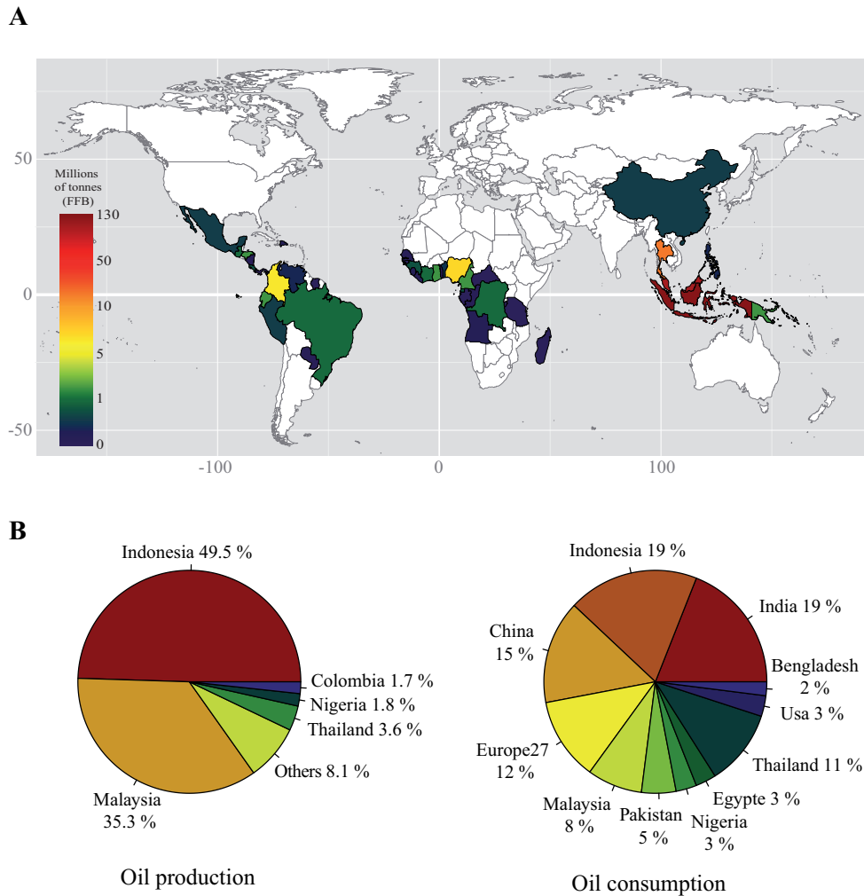
Figure I.4: A) Geographical distribution of oil palm production in the world (FAOSTAT 2014). B) Distribution of the main producing and consuming countries of palm oil in the world. (FAOSTAT 2013).
