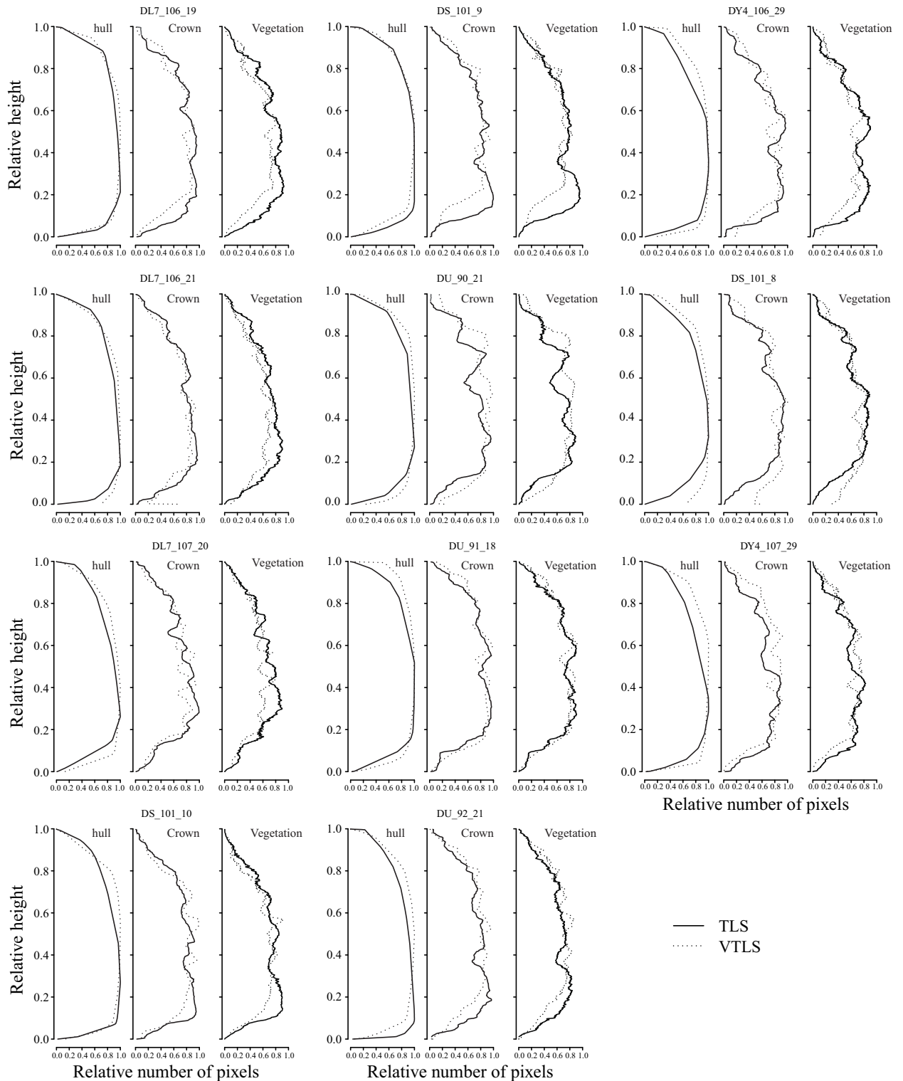
Figure III.13: Comparison of hull, crown (vegetation + microgaps) and vegetation profiles from TLS and VTLS orthographic views for the 11 studied palms. Number of pixels are expressed relatively to the number of pixels corresponding to the maximum width of the hull.
