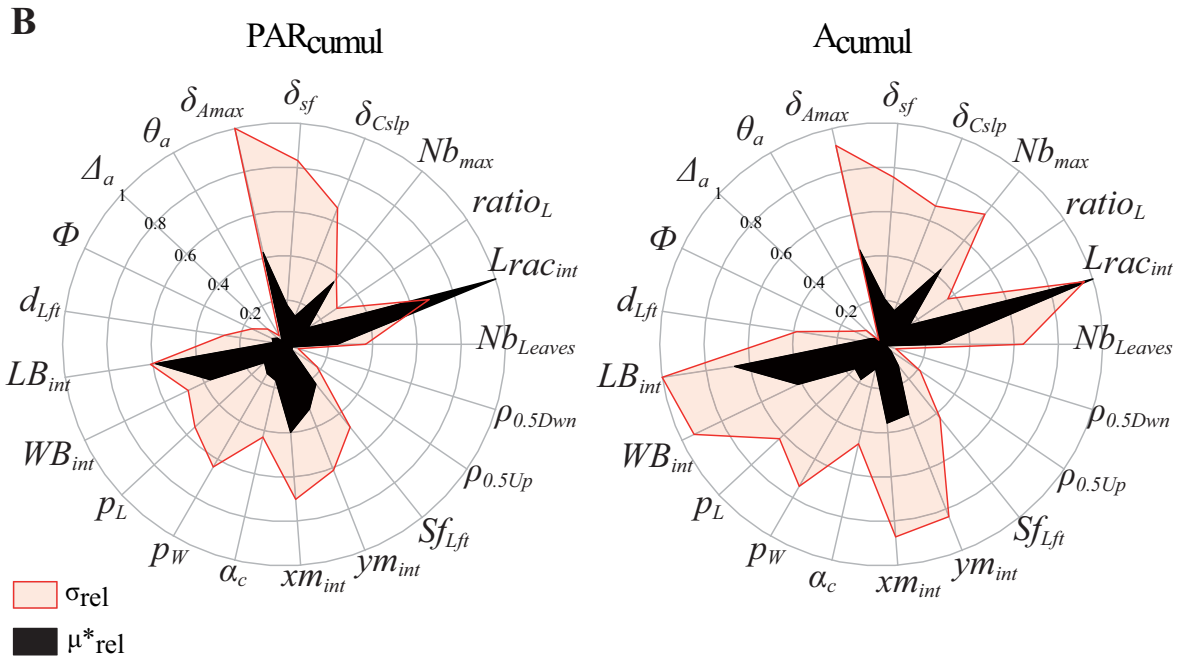
Figure IV.3: A) Heat map of relative mean values of elementary effects ( \mu_{rel} ) for 6 ages over plants development, calculated for the fraction of PAR intercepted by the canopy ( f_{PAR} ) and carbon assimilation ( A_d ). Values are given relatively to the most sensitive parameter at a given age. B) Morris sensitivity indices for cumulated PAR intercepted ( PAR_{cumul} ) and cumulated carbon assimilated ( A_{cumul} ). Index values are relative to the most sensitive parameter, \mu^*_{rel} is the relative absolute mean value of elementary effects.
