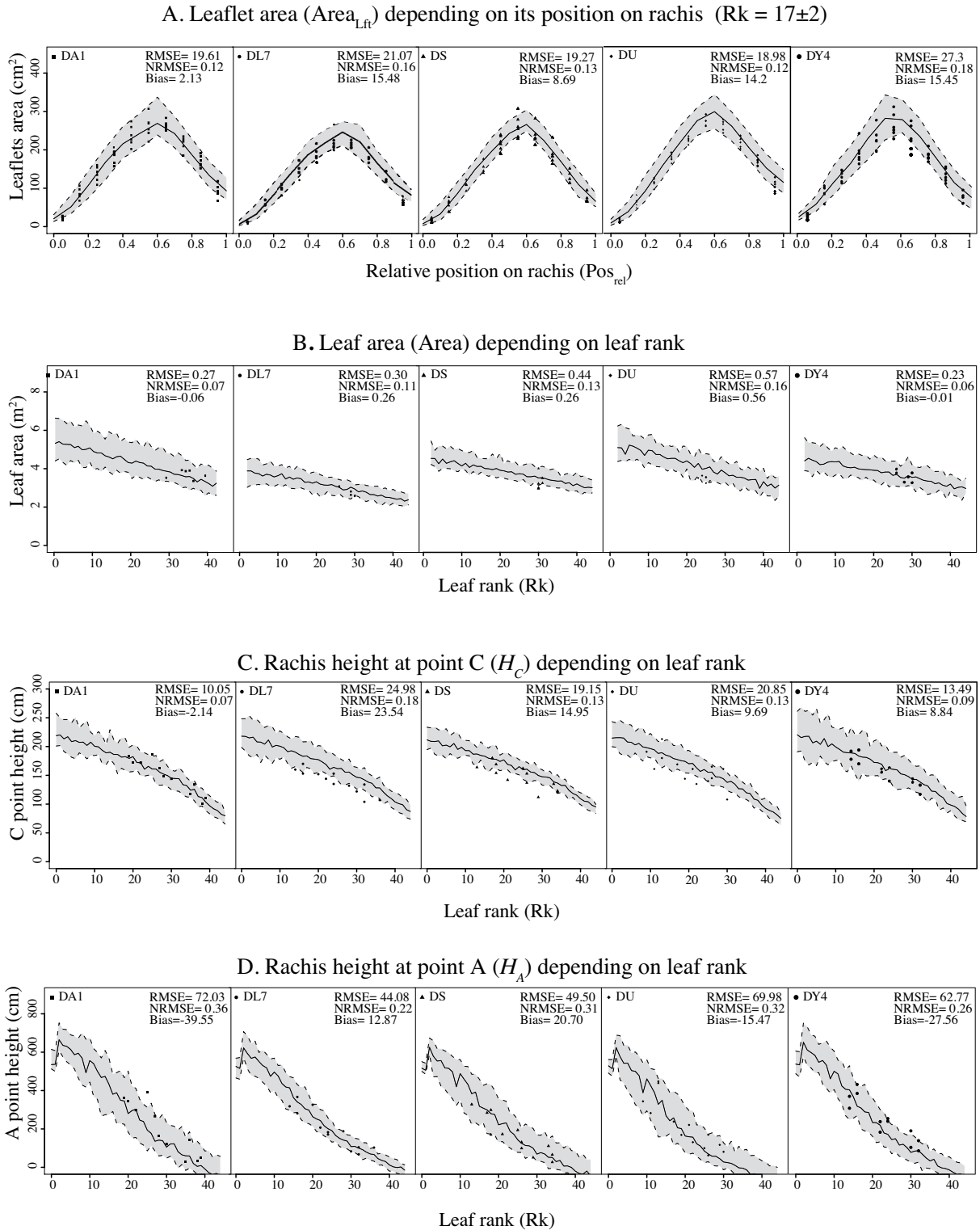
Figure II.5: Evaluation of model reconstruction for five progenies. Mean (continuous lines) and 95% confidence interval (envelopes) of predictions are calculated from 25 plants simulated with VPalm for each progeny. Points represent observed values.
