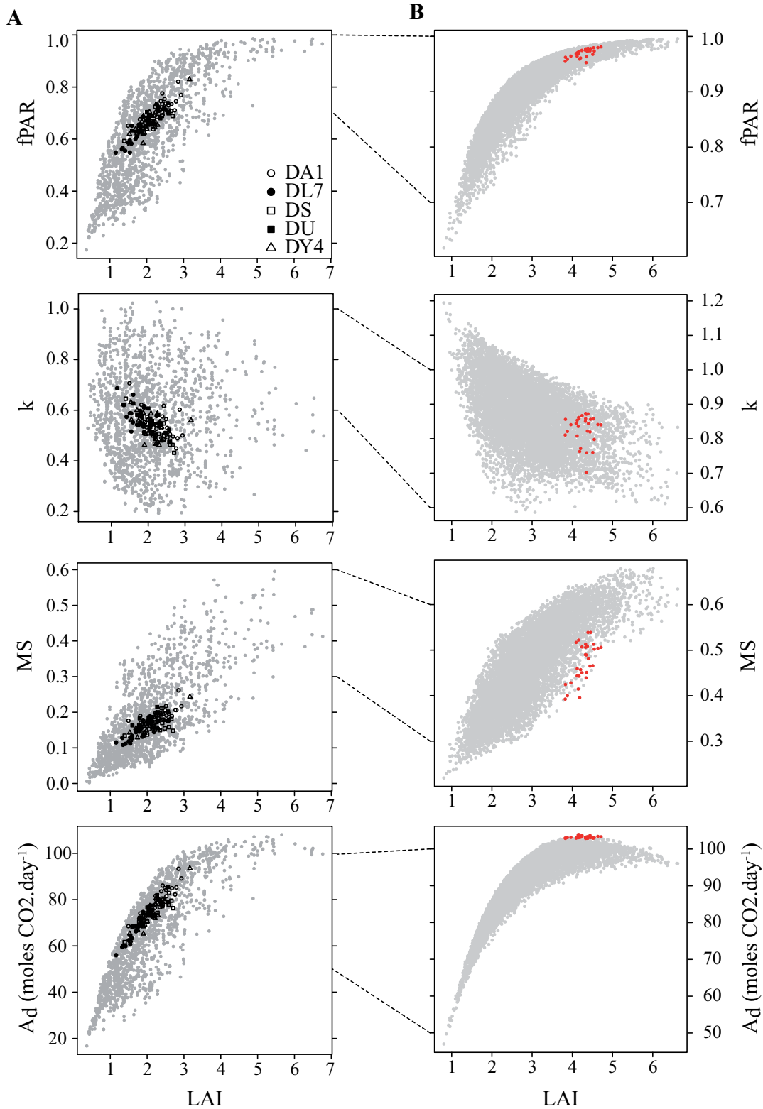
Figure IV.4: A) Dispersion of output variables for all the virtual plants generated with combinations of the 21 architectural parameters for the Morris analysis at 100 and 150 leaves emitted after planting (1760 mock-ups, grey points) and from mock-ups generated at equivalent age for the five studied progenies (20 individuals per progeny). B) Dispersion of output variables for all the virtual plants generated with combinations of the nine most sensitive architectural parameters at 450 leaves emitted (8192 mock-ups). Red points represents the 30 mock-ups with the highest values of A_d
