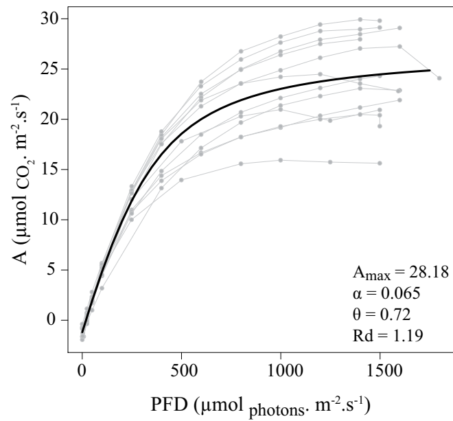
Figure IV.11: Calibration of non-rectangular hyperbola (NRH) curve for simulating leaf photosynthesis. Lines in grey represent the response curves measured on 12 different oil palm leaves (from 8 individuals, on leaflet at point B from leaf rank between 9 and 17). Black line represents average model adjustment (values of calibrated parameters are presented at bottom right of the graphic).
