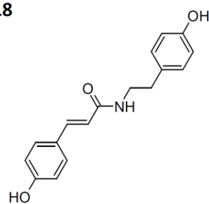
p -coumaroyl-tyramine
