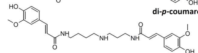
di-feruloyl-spermidine
