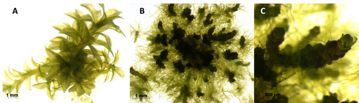
Figure 2.9 P. patens cyp98a34 mutant phenotype.
