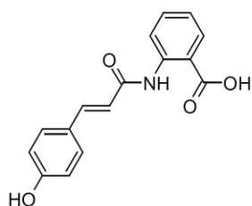
p -coumaroyl-anthranilate
