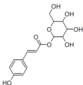
p -coumaroyl-β-D-glucose
