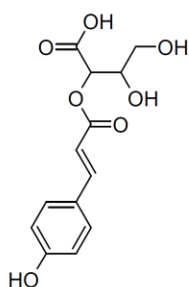
p -coumaroyl-2-threonate
