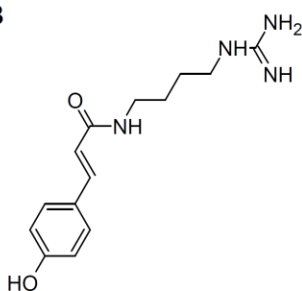
p -coumaroyl-agmatine
