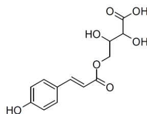
p -coumaroyl-4-threonate
