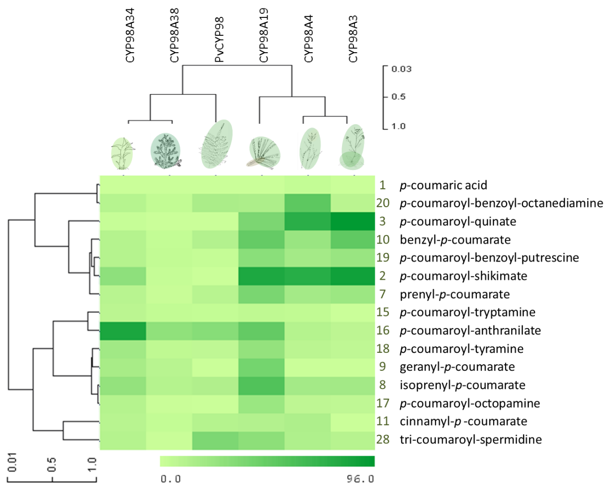
Figure 2.7 Hierarchical clustering of substrates and P450s tested in the substrate screening.
