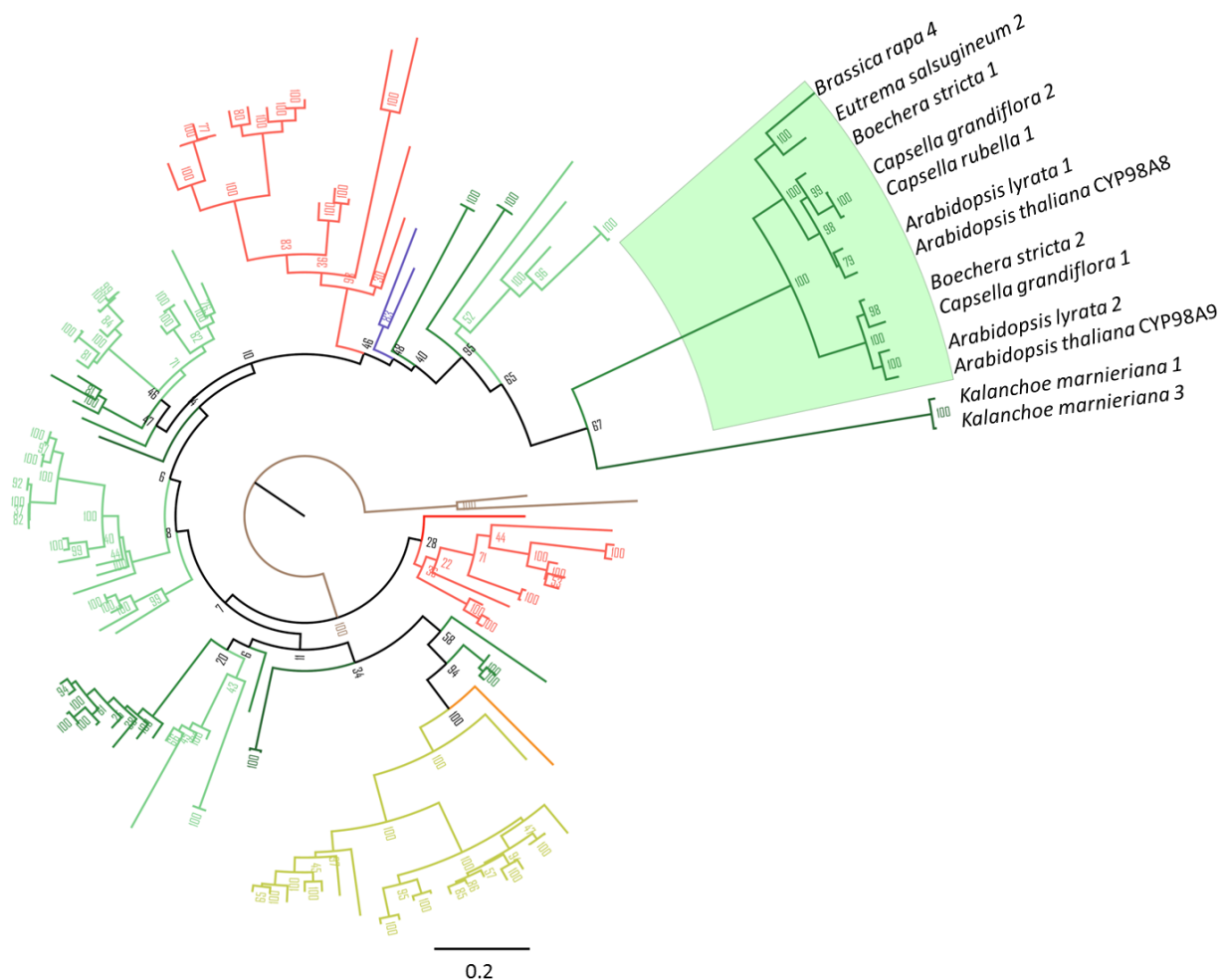
Figure 3.4 Phylogenetic reconstruction of CYP98 sequences from angiosperms with sequenced genomes and characterized CYP98s.
