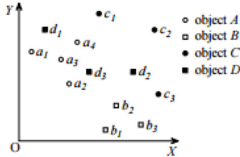
Figure 2.3: Uncertain objects
