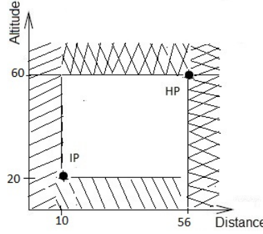
Figure 4.1: Marginal Points
