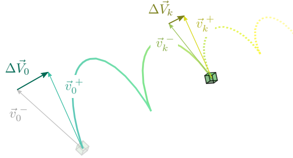
Figure 4.4: Impulsive maneuvers along the glideslope approach.
