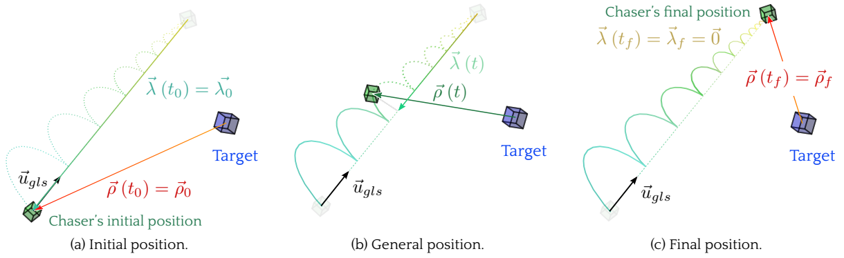
Figure 4.2: Chaser satellite following a glideslope approach.
