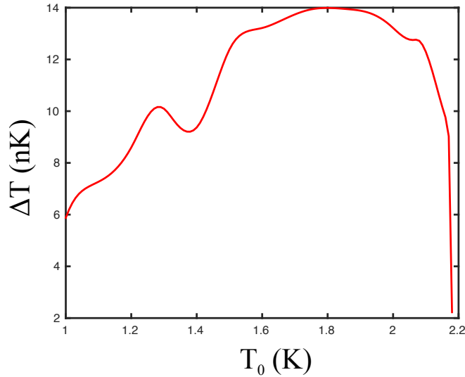
Fig.V.14 – The calculated \Delta T as a function of T_0 using Eq.(V.8).
