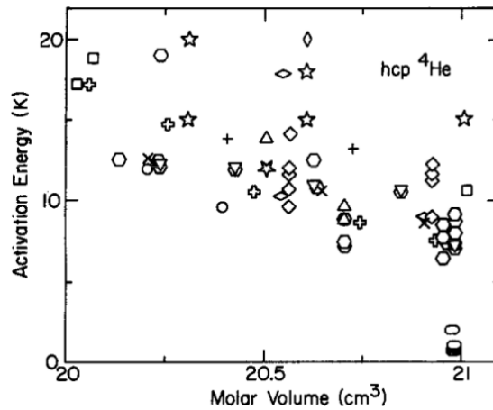
Fig.I.2 – The figure is extracted from [24]. It summarized the existing experimental results for E_v as a function of the molar volume. There is a big difference between different data points, because they crucially depend on the vacancy model used to analyze the measurements.
