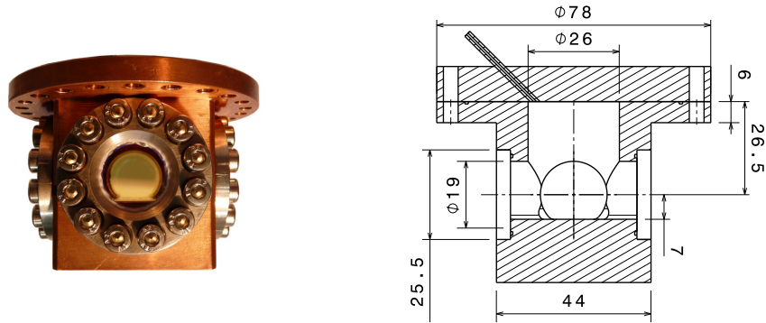
Fig.II.2 – Photo and blueprint of experimental cell. Its inner cavity is like a hollow cylinder with four circular ports. The floor of the cavity is flat and polished to allow free growth of helium crystals. There is a copper cover on top of the cell. The total inner volume is 30 cm 3 .
