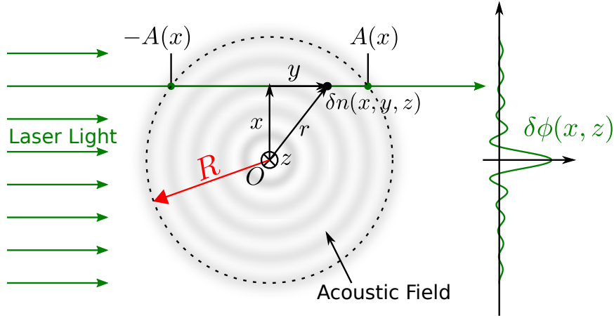
Fig.II.10 – The sectional plan of Fig.II.9, they share the same coordinate system. Laser beam propagates along y -axis. The sound field induced by the PZT is shown as blurred gray circles. The dotted circle R is the limit of the PZT, it defines the range of the sound field. On the right side of the figure, is the profile of \delta\phi as a function of coordinate x .
