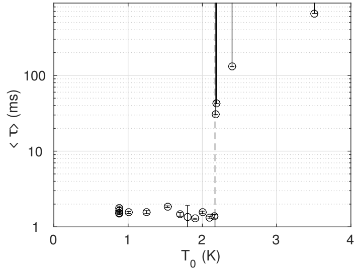
Fig.V.10 – Lifetime of bubbles in liquid helium as a function of temperature. The vertical dashed line marks the superfluid transition temperature ( T_\lambda = 2.17 K). Above T_\lambda , we can only estimate the lower bound of the lifetime.
