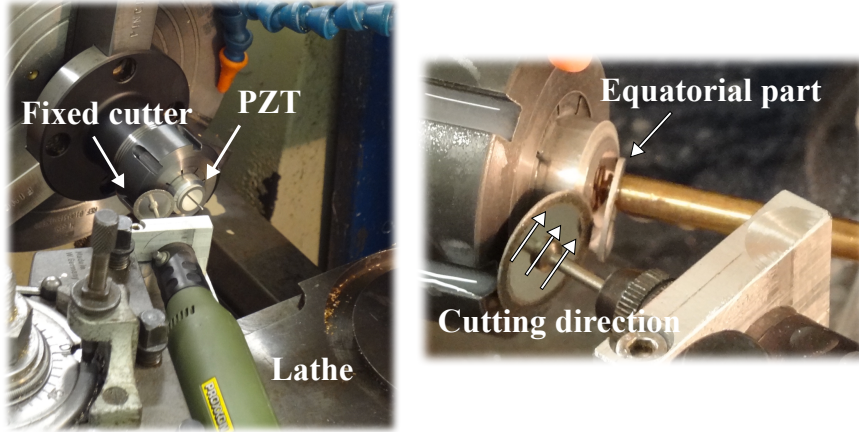
Fig.II.4 – Our first attempt of manufacturing PZT. Left: PZT is fixed on faceplate of lathe, and cutter is placed on carriage. We cut PZT with an attacking angle of 10 degree; Right: A small equatorial part of height 1.4 mm is removed from PZT.
