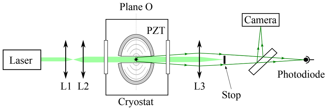
Fig.III.1 – Experimental arrangement to monitor the light scattered by the damaged region (plane O) at a microsecond time scale. The beam of a CW laser, expanded by two lenses ( L_1 and L_2 ), illuminates the region where the instability occurs. The unscattered light is focused by L_3 and absorbed by a beam stop, while the light scattered by the damage is collected by a fast photodiode. Using a semi-transparent plate, images of plane O can be simultaneously recorded on a standard CCD camera.
