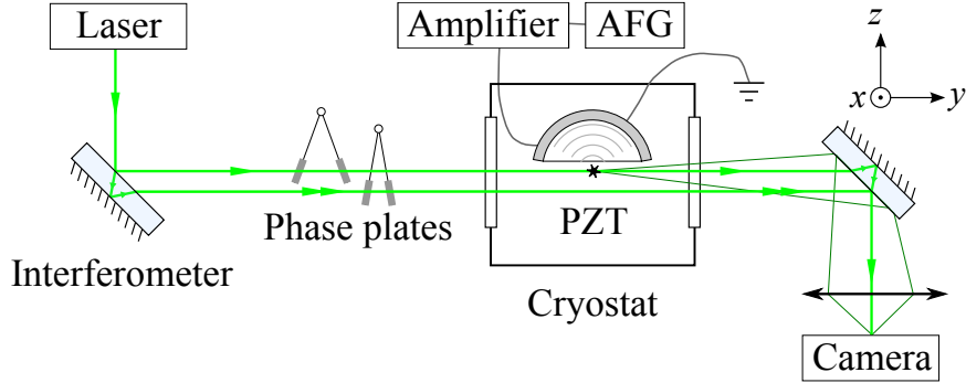
Fig.II.15 – Scheme of the entire optical system. At the center of the transducer, the small star is the acoustic focus. A CCD camera monitors the focus plane through a lens.
