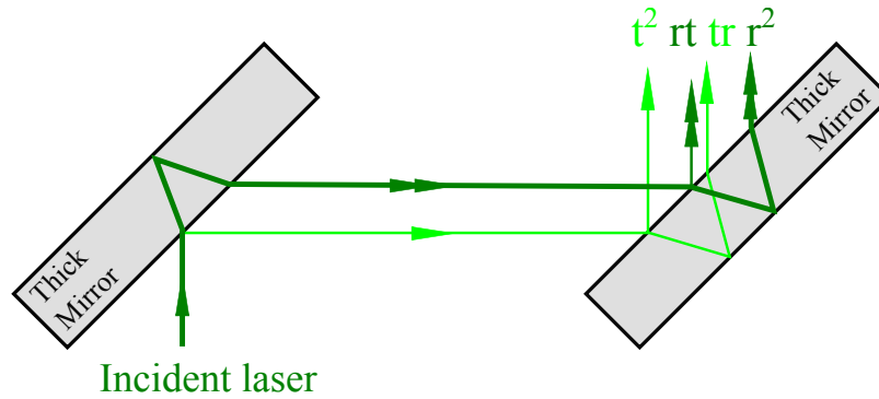
Fig.II.11 – Schematic plan of a typical Jamin interferometer. The two mirrors are parallel. While the first mirror separates the incident light into two beams, the second mirror combines them. In the figure, the second reflection of the two beams are marked with different colors and respectively noted by t^2 , rt , tr and r^2 . In reality, the rt and tr beams coincide and interfere.
