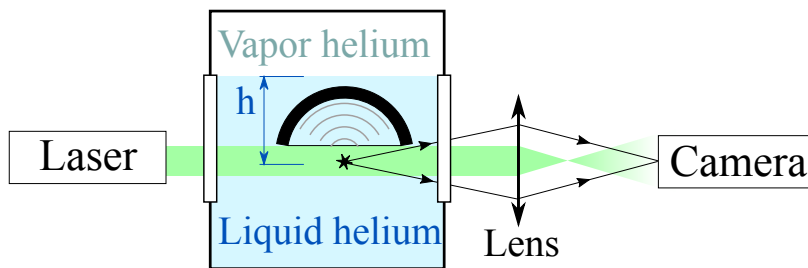
Fig.V.1 – Experimental set-up. PZT is immersed in liquid helium. The height of liquid above the sound focus is marked by h . The CCD camera focuses on the focus plane through a lens.
