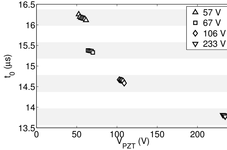
Fig.III.3 – Times of birth t_0 of 20 instabilities at different driving voltages of the PZT. For clarity, the symbols for a given excitation voltage are slightly horizontally dispersed around their nominal values. Error bars are within the data point sizes. Gray areas: Time intervals of negative swings of the pressure wave at sound focus.
