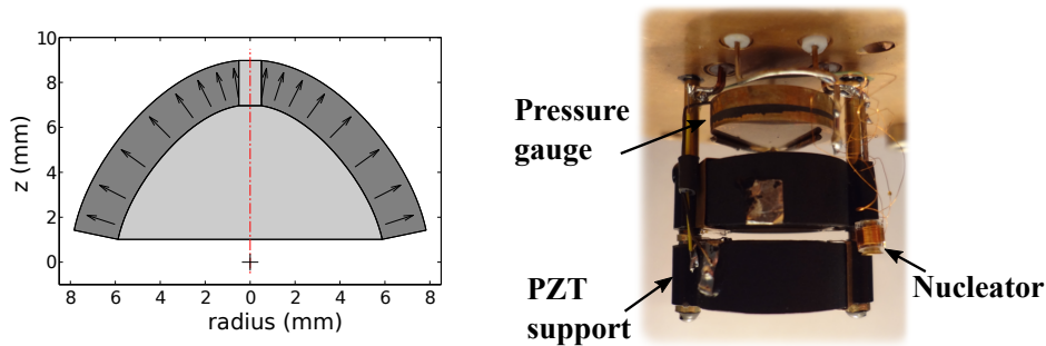
Fig.II.6 – Left: Plan of PZT in solid helium. This sectional profile can compensate the anisotropy of ultrasound velocity. Acoustic focus is marked with black cross. Black arrows represent poling direction. Right: Photo of mounted support and PZT in solid helium. Compared to the one in superfluid, we added a capacitive pressure gauge and a nucleator.
