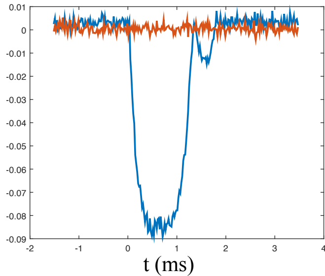
Fig.V.17 – Raw signals of the photodiode. The red line is the signal without a bubble, and the blue one is the signal with a bubble. The bubble scatters light so that it lowers the light intensity received by the photodiode.
