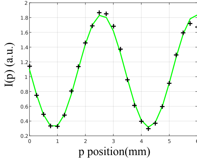
Fig.II.14 – The cross data points are the measured intensity I(p) as a function of p . The green curve is the corresponding sinusoidal regression of the free parameters in Eq.(II.7). These two parameters depend on the inclination angle between the phase plates and the laser beam, which is very difficult to measure.
