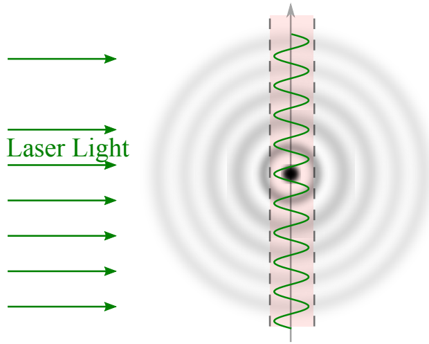
Fig.II.16 – Diagram of the simplified sound field. The amplitude of phase modulation radially increases as 1/r . Roughly speaking, only the central red zone contributes to the light diffraction. Then we can further simplify that in the dashed line zone, the phase modulation is uniform.
