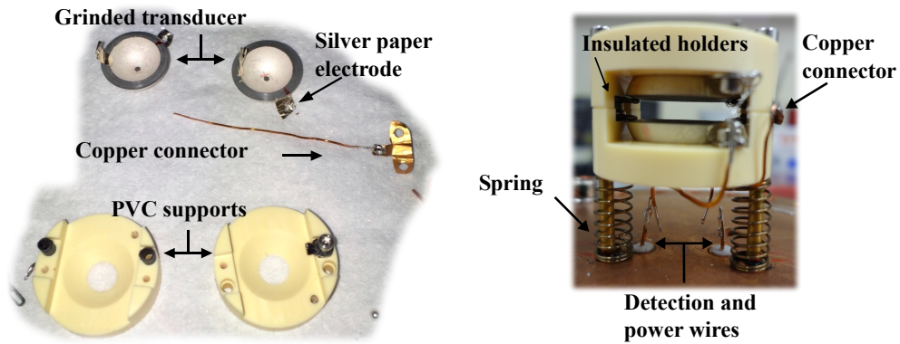
Fig.II.5 – Left: Unmounted PZT and PVC supports. Two silver paper electrodes are already stuck on each transducer. The connector is made of copper paper. All these electric parts have small holes for screws. On PVC support, there are two black plastic tube for insulating bronze sticks. Right: Mounted transducers and support. All connections and fixations are made by springs and screws.
