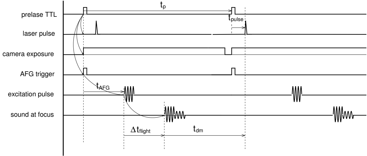
Fig.V.3 – The diagram of the modified time line, which is based on Fig.II.17. We shift all the measurements by the period time T , so as to observe the bubbles who last longer than 170 \mu s .
