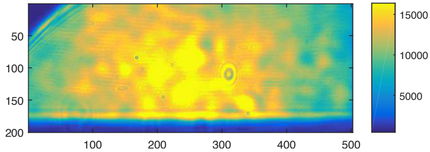
Fig.V.6 – Raw image captured by the CCD camera, the color bar at right side indicates the light intensity. x , y -axis represent the pixel coordinate of the camera. We can roughly find a small bubble around the pixel (300, 100).
