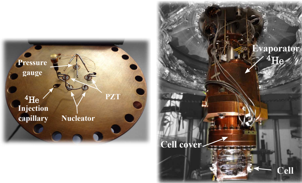
Fig.II.3 – Left: Photo of the cell cover, there are six tunnels on this cover. The one on the left is an injection capillary for helium. The other five are tunnels for wires. This cover is used in solid helium experiments, so we have three additional tunnels for nucleator (see Sect.II.3.2) and pressure gauge (see Sect.II.1.2); Right: Photo of the entire experimental cell part. On the top are the evaporator and wires. Cell cover serves as an important junction between them and the cell. On the photo, the cell (at bottom) is temporarily wrapped with cling film for protection purpose.
