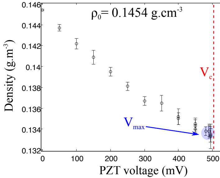
Fig.IV.7 – Experimental measurements of minimum densities \rho_{min} for different driving voltages V at T = 0.96 K and P_{static} = 0.15 bar. The data points in the blue circle are the measurements at V_{max} . The dashed red line represents the cavitation voltage V_c .
