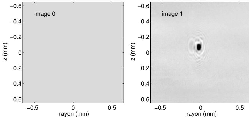
Fig.I.4 – Images of the instability's appearance, extracted from the thesis of F. Souris [2]. Nothing appears in image 0, but in image 1 it shows up. The instability appears in image 1 as an oval defect at the center of the image. The size of this defect is of the order of 0.1 mm.
