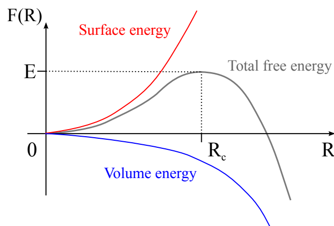
Fig.I.7 – An illustration of the nucleus free energy F(R) . The total free energy is the sum of the surface term and the volume term. It reaches the maximum energy barrier at R_c .
