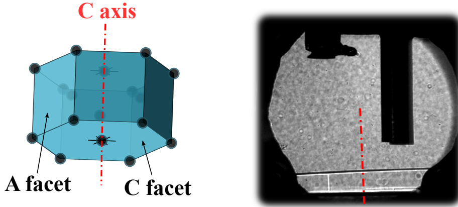
Fig.II.7 – This figure shows hcp solid helium structure. The C-axis in red is perpendicular to C facet, and parallel to A facet. This structure is visible below temperature T = 1.30 K. On the right side is a photo of crystal during its growth at 1 K, the contact line between two A facets is then visible.
