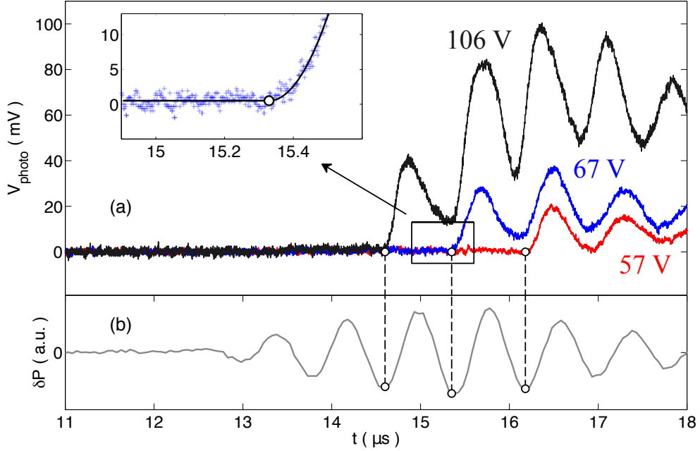
Fig.III.2 – a) Photodiode voltage as function of time for 3 experiments creating solid helium instabilities at different PZT driving voltages. The sharp increase of the signal corresponds to the appearance of damage. The open circles give the time of birth t_0 . Inset: Typical fit of the photodiode voltage as function of time using Eq.(III.1.3). b) Pressure variations at sound focus in arbitrary units for temporal reference.
