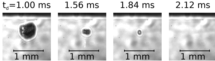
Fig.V.4 – Determining the lifetime of cavitation bubbles: data for T_0 = 0.87 K. Images of typical bubbles at different times t_d (see text). The upper black stripe is the shadow of the PZT.
