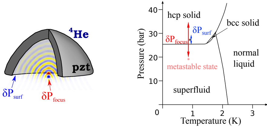
Fig.I.3 – The transducer creates a small variation of pressure on its surface \delta P_{surf} . As acoustic wave propagates and focuses, \delta P_{focus} will become much larger. If we start from an initial state near the phase transition line, helium at focus will become metastable. This technique is available for both solid and superfluid helium.
