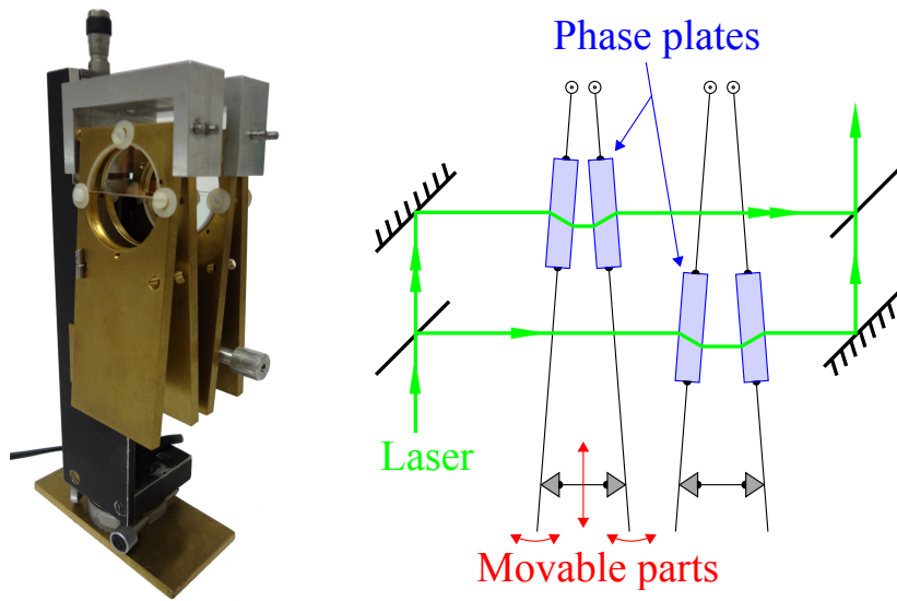
Fig.II.12 – Photo and schematic plan of phase plates and their support. Each phase plate is a half circle of 4 mm thickness and 40 mm diameter. Each pair of phase plates are made by cutting a flat circular glass window so that they have the same thickness and flatness.
