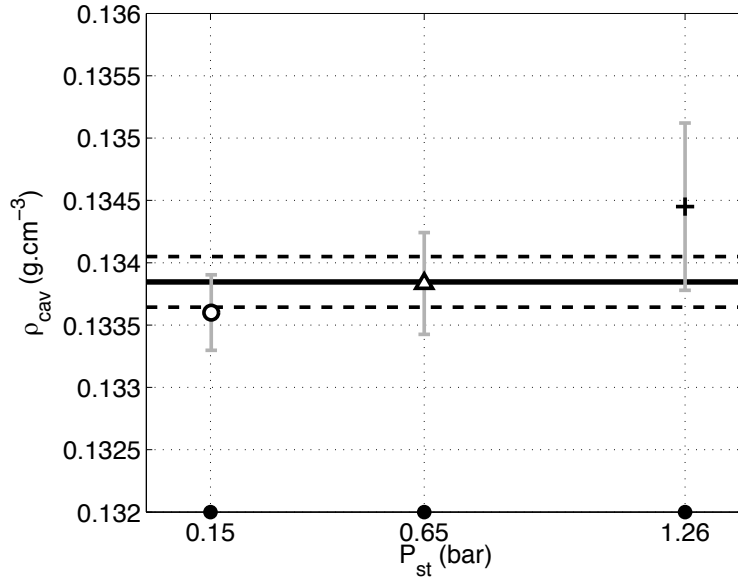
Fig.IV.9 – Same data as Fig.IV.8, but data points are averaged for each pressures.
