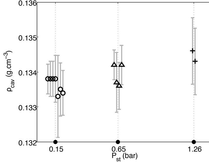
Fig.IV.8 – 13 measurements of the cavitation density at three different P_{static} . For more clarity, the different measurements are shifted from their actual P_{static} values.
