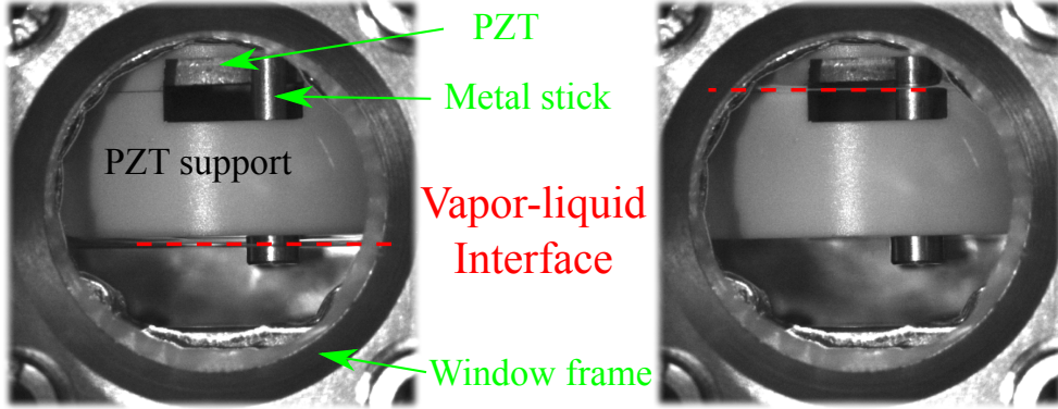
Fig.V.2 – Pictures of the experimental cell being filled with liquid helium. As marked in the left one, the support of the PZT occupies most of the visible zone through the circular window. The ceramic PZT is hung on the upper part of the PZT. Vapor-liquid interface is indicated by the dotted red lines.
