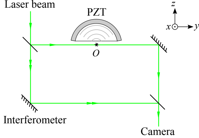
Fig.II.9 – A simplified plan of the interferometer. The incident laser beam is separated into two beams. One passes through the sound field induced by the PZT, and the other passes through an unperturbed zone. We can detect the interference at the end. A detailed description of the optical setup is given in Sect.II.4.3.2.
