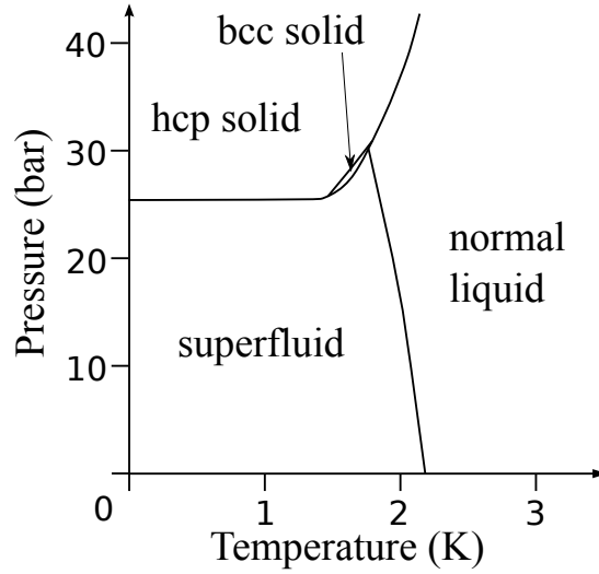
Fig.I.1 – Phase diagram
