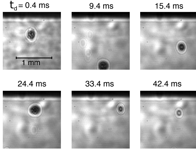
Fig.V.12 – Cavitation bubbles at T_0 = 2.19 K. The maximum diameter is about 200 \mu\text{m} . At first five milliseconds, bubbles are at the PZT focus. Later, bubbles become randomly distributed in the vision.
