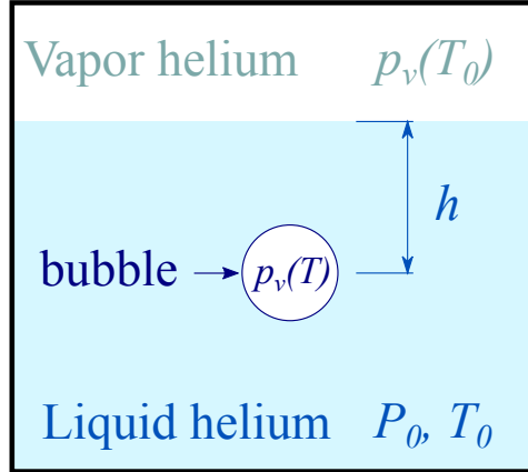
Fig.V.13 – A diagram of the temperatures and pressures in liquid and in bubble.
