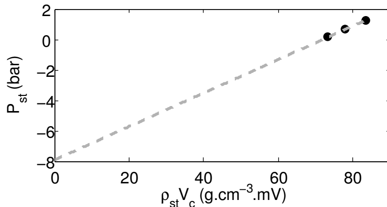
Fig.IV.10 – Reproduction of reference [51] experiment. P_{static} as function of \rho_{static}V_c . The 3 data points (black circles) correspond to static pressures of 0.15 bar, 0.65 bar, 1.26 bar. Cavitation voltage are the ones shown in Fig.IV.5. The dotted line is the linear extrapolation of the data points.
