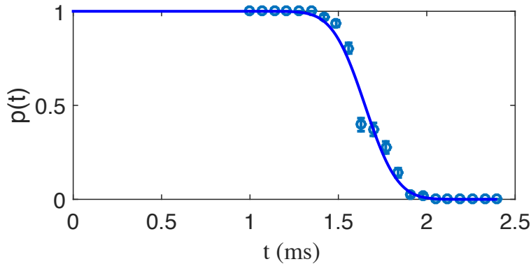
Fig.V.9 – Determining the lifetime of cavitation bubbles: data for T_0 = 0.87 K. Probability of existence of a bubble at time t . The solid line is a fit assuming that the lifetime of the bubble is gaussian distributed. The mean value \langle \tau \rangle = 1.65 ms, the half height length \xi = 0.10 ms.
