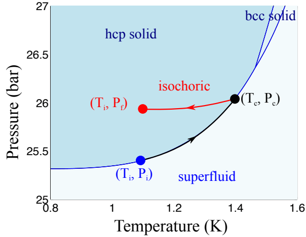
Fig.II.8 – A presentation of the crystal’s growth process on the phase diagram. We bring the crystal seed from its initial state (T_i, P_i) to a higher pressure state (T_c, P_c) , and grow the crystal at this state until the cell is filled with crystal. Then we slowly reduce the temperature so that the crystal follow the red isochoric line and finally reach the final state (T_i, P_f) .
