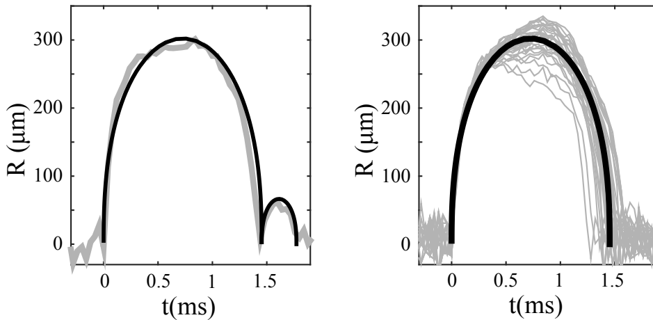
Fig.V.18 – Bubble radius as a function of time at T_0 \sim 1 K. On all figures, black solid line is the Rayleigh solution of the Rayleigh-Plesset equation (eq:V.9). Left: Gray curve is one typical photodiode measurement. After the bubble has collapsed, a second bubble is created. Right: Gray curves is the superposition of 100 measurements of the bubble evolution.
