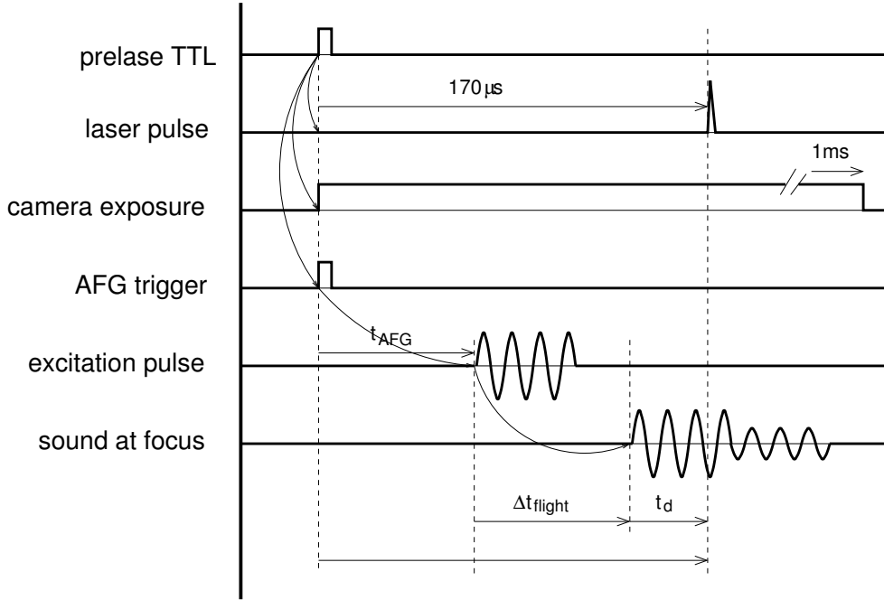
Fig.II.17 – The time line in a single measurement. The time arrow is towards right. 1) Initial trigger at t_0 , it precipitates the camera the AFG and the amplifier. 2) After the delay t_{AFG} , the sound wave sent by the PZT. 3) After the time of flight t_{flight} , the sound wave arrives at the focus. 4) The laser pulses at the pre-lasing time t_{pulse} , and an image is captured at this time.
