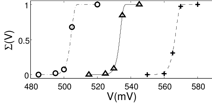
Fig.IV.5 – Cavitation probability at 0.96 K for three different pressures P_{static} : circles 0.15 bar, triangles 0.65 bar, crosses 1.26 bar. The corresponding lines are fits according to Eq.(IV.2).
