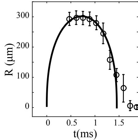
Fig.V.15 – Bubble radius as a function of time at T_0 \sim 1 K. Circles are the data obtained from the bubble images (see Sect.V.2.1). The black curve is the solution of Eq.(V.9).
