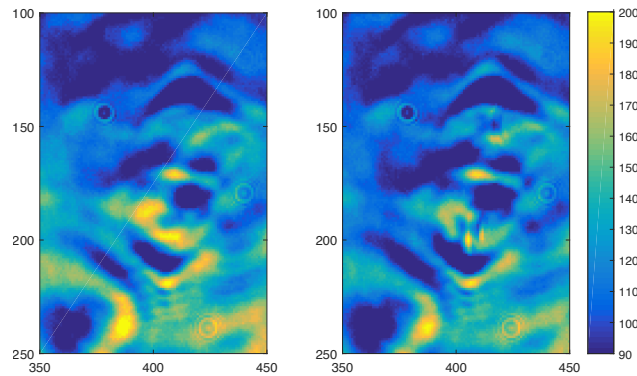
Fig.IV.2 – Partial zoom of the acoustic focus of two raw images. Both images are taken at T = 1.05 K and P_{static} = 25.14 bar, time delay t_d = 3.73 . \mu s . But their AFG voltage are different: left V_1 = 745 mV; right: V_2 = 820 mV. The left one is the same one shown in Fig.IV.1. The color bar is an arbitrary unit indication of the light intensity.
