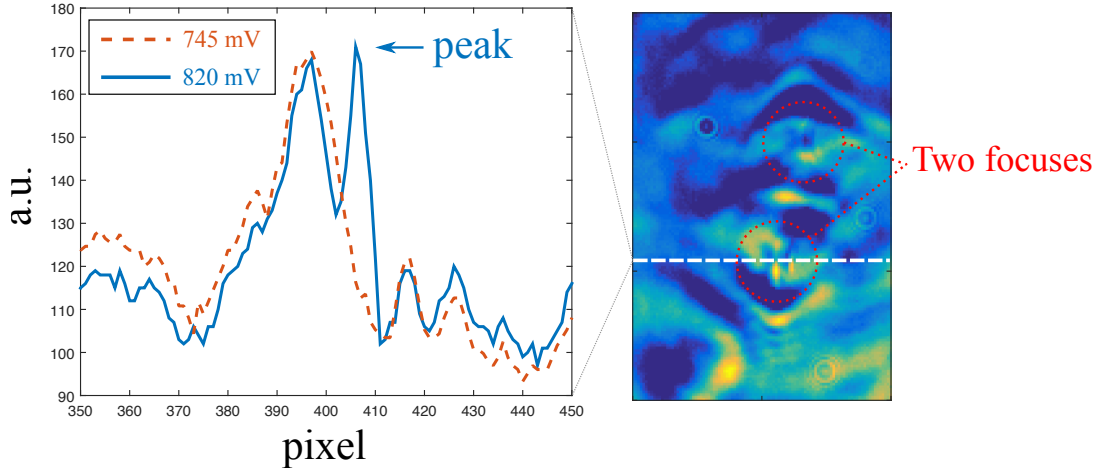
Fig.IV.3 – The profiles of light intensity for the same row of the two images shown in Fig.IV.2. Because the sound wave amplitudes are different in the images, we normalized the light intensity by multiplying one image by a factor so that most pixels of the curves are overlapped. The red dotted line is the profile of V_1 = 745 mV, and the blue line is the profile of V_2 = 820 mV. There is an abnormal peak around the pixel (405,191). On the right side, the horizontal line shows the position of the row. And the two circles are the two separated focuses.
