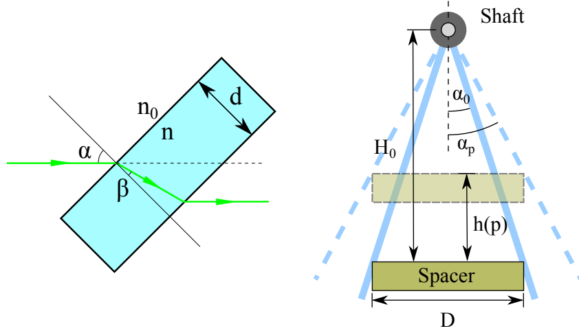
Fig.II.13 – Left: A horizontal laser beam passes through the inclined phase plate of thickness d . The incident angle \alpha is the same as the open angle of phase plate. Right: The schematic plan of the spacer and phase plates' support. Blue lines show two different positions of phase plates, which correspond to two different open angles \alpha_0 and \alpha_p . H_0 is the initial distance between the spacer and the shaft axis, and h is the change of the spacer's height.
