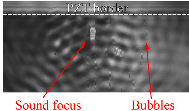
Fig.V.11 – Cavitation bubbles at T_0 = 2.19 K. The big bubble is acoustically created at the PZT focus. Other small bubbles are the survivors from previous sound bursts. This photo was taken at a much higher PZT driving voltage. The variation of refractive index is so high that sound wave deflects much light out of sight, and so makes fringes visible.
