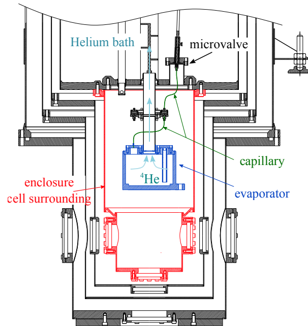
Fig.II.1 – This design plan of the cryostat shows its main parts, such as helium bath, evaporator, optical ports and protection enclosures. The experimental cell (not shown in this figure) will be mounted below the evaporator. The optical port on the bottom was initially planned but is not used in this work.
