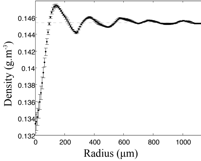
Fig.IV.6 – Typical radial density profile for P_{static} = 0.15 bar at the time when the density is minimum at acoustic focus. The static density corresponding to P_{static} is shown by the horizontal dashed line.
