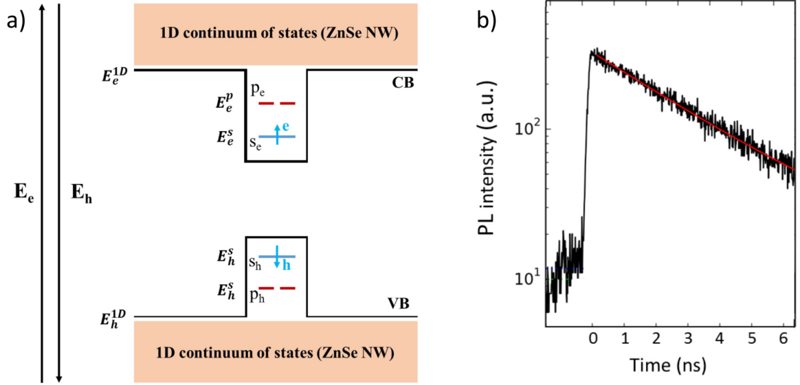
Figure 3.41: a) QD electronic structure described by two discrete levels: the fundamental s (electron and hole energy levels E_e^s and E_h^s ) and excited p (electron and hole energy levels E_e^p and E_h^p ) levels, surrounded by a 1D continuum of states (the ZnSe NW). b) Example of an exciton decay recorded at 75 K on NW1 from S_{1QD}^{Se} (same as in Figures 3.40 and 3.42). This decay shows a clear monoexponential behavior, representative of the measured NW-QDs decays.
