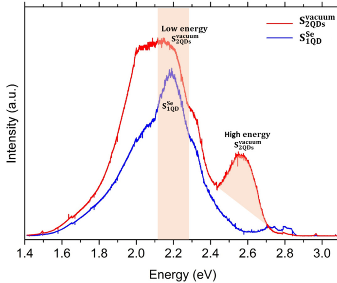
Figure 3.34: MacroPL spectra of the as-grown S_{1QD}^{Se} and S_{2QDs}^{vacuum} recorded at 10 K with a 405 nm laser excitation of \sim 100 \mu W . The emerging part of the QDs emission distributions are highlighted by semi-transparent orange areas. For S_{2QDs}^{vacuum} , the two CdSe QDs emissions are visible at low (2.2 eV) and high (2.55 eV) energies.
