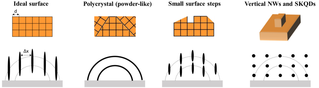
Figure 1.18: (Upper part) Illustration of surface morphologies that can be encountered during MBE growths and (lower part) the corresponding RHEED patterns. d is the in-plane distance at the sample's surface and \Delta x is the vertical streaks horizontal separation on the RHEED pattern.
