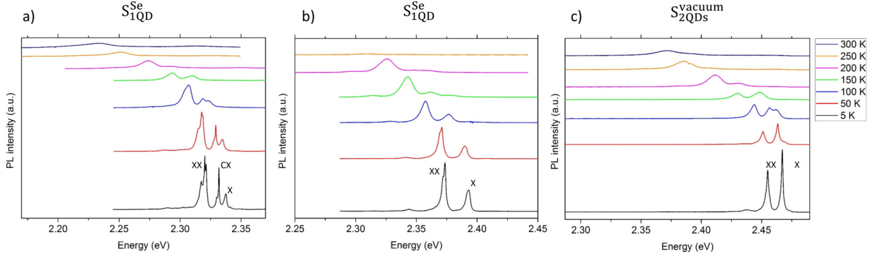
Figure 3.38: \mu PL measurements as a function of the temperature (from 5 to 300 K) of three NW-QDs deposited on a patterned substrate from S_{1QD}^{Se} and S_{2QDs}^{vacuum} . Notice that for the two NW-QDs from S_{1QD}^{Se} , the first one in a) displays a charged-exciton while only the exciton/biexciton are visible for the NW-QD shown on b). The measurements were carried out with a 488 nm laser and a power excitation of 712 \mu W.
