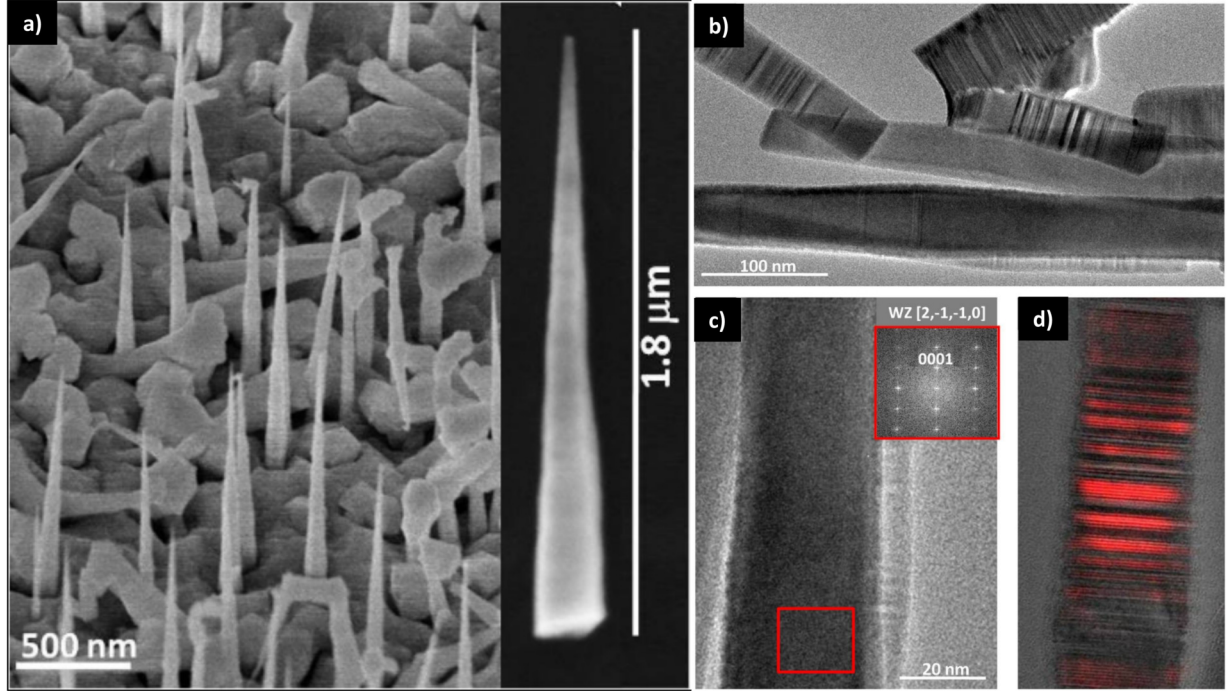
Figure 2.1: a) Tilted-view SEM image ( 45^\circ ) of ZnSe NWs grown at 300^\circ\text{C} on GaAs(111)B. The inset on the right is a magnified image of a representative NW, mechanically transferred onto a patterned substrate. b), c) and d): TEM images of ZnSe NWs transferred on a TEM grid from the same as-grown sample as displayed on the left. b) Ensemble of NWs. c) Representative image of a defect-free WZ NW. Inset: Fourier transform of the red rectangle on c) highlighting the WZ structure of the NW (zone axis WZ [2,-1,-1,0] ). d) False-color high resolution TEM image of a NW with alternating WZ (red) and ZB crystal phases of various thickness.
