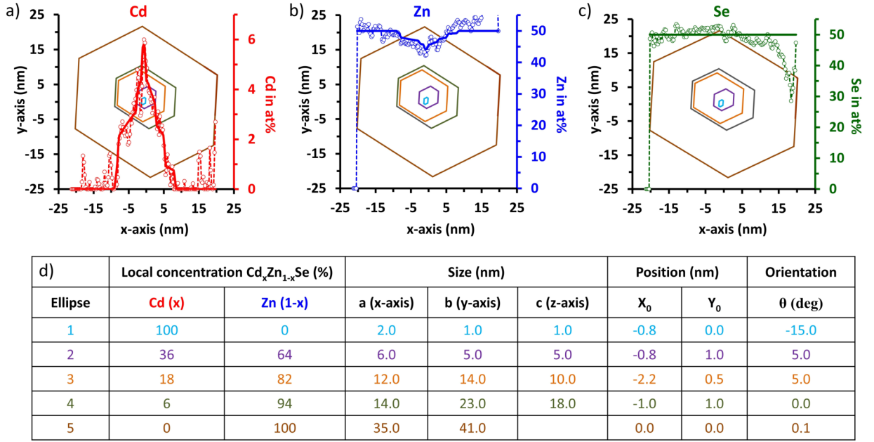
Figure 3.24: a) Cd, b) Zn and c) Se relative composition (atomic % of content averaged over the local thickness) along the line scan across the QD insertion at a 0° tilt-angle (see rectangle in Figure 3.22). Experimental data: open dots; calculated values using the 5 imbricated hexagons.: solid black curve). d) Table summarizing the set of parameters used to fit our data. For each hexagon, the parameters are the Cd, Zn and Se concentrations, the size of the hexagon (along the x, y and z axis), its center position ( X_0, Y_0 ) and orientation ( \theta ). The colors used for each imbricated hexagons are reported in the Table for visualization purpose.
