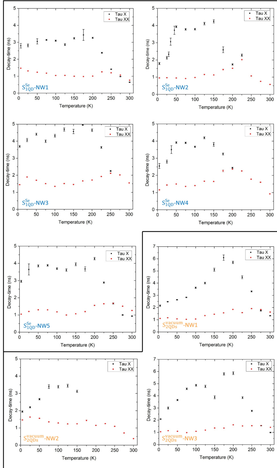
Figure 3.40: Decay-time of single ZnSe-CdSe NW-QDs as a function of the temperature from S_{1QD}^{Se} (top part in blue) and S_{2QDs}^{vacuum} (bottom part in orange). The exciton and biexciton decay-times are displayed respectively in black and red.
