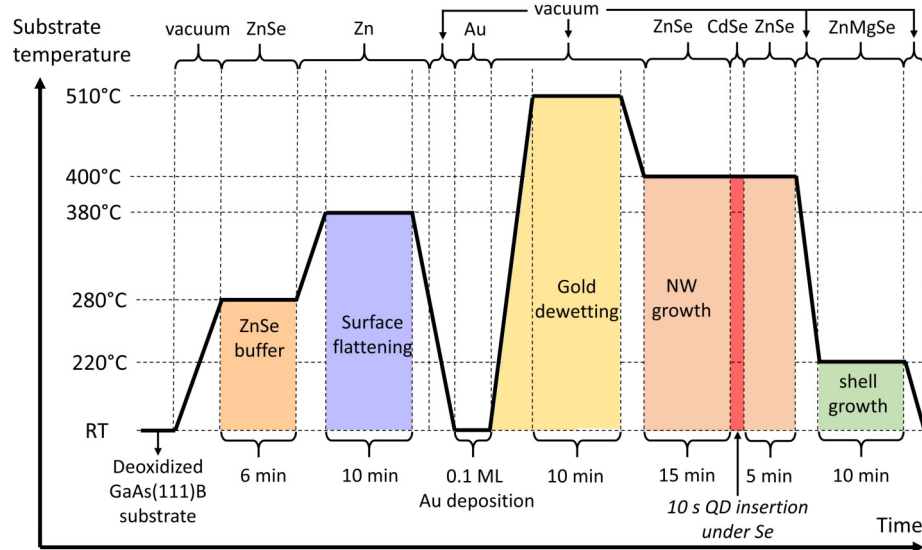
Figure 3.6: Illustration of the growth process of S_{1QD}^{Se} : ZnSe NWs with one CdSe QD insertion (10 s) grown at 400°C under Se-rich conditions and a nominal Zn_{0.90}Mg_{0.10}Se shell deposited during 10 min at 220°C.
