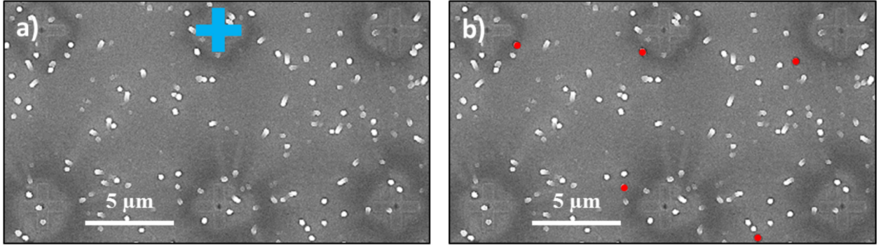
Figure 4.15: Top-view SEM images of the sample composed of 110 nm \text{Al}_2\text{O}_3 shell radius photonic wires. This sample has been etched by FIB to create regular squared patterns of 2.5\text{ }\mu\text{m} \times 2.5\text{ }\mu\text{m} crosses (a single cross is colored in blue for visualization purpose) separated by 10\text{ }\mu\text{m} . The SEM images are displayed a) before and b) after the localization of photonic wires emitting a clear excitonic signature, labeled by red circles on the image.
