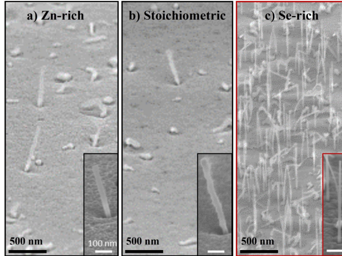
Figure 2.22: Tilted view SEM images (65°) of ZnSe NWs grown on a (111)B substrate at 400°C under a) Zn-rich (Zn:Se nominal growth speed ratio of 3:2), b) stoichiometric (Zn:Se of 1:1) and c) Se-rich conditions (Zn:Se of 1:2). All the white scale bars of the insets represent 100 nm.
