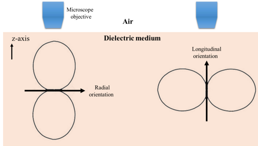
Figure 4.5: Illustration of dipole emissions in an homogeneous dielectric medium. The radial and longitudinal (according to the z-axis) dipole orientations and there radiation pattern in vacuum are sketched to highlight their difference for the photon collection in a microscope objective. Indeed, more light is expected to be collected from the radial dipole.
