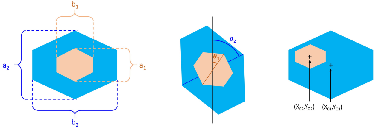
Figure 3.19: The hexagons have five parameters that can be tailored: their axes length a and b , their tilt-angle and the position of the center (X_0, Y_0) .
