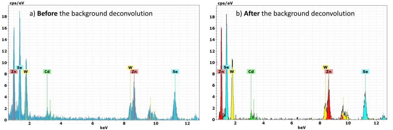
Figure 3.20: EDX spectrum from the analyzed ZnSe-CdSe NW-QD from S_{1QD}^{Se} a) before and b) after the background deconvolution. Only the colored peaks are used to quantify the concentration of each element.
