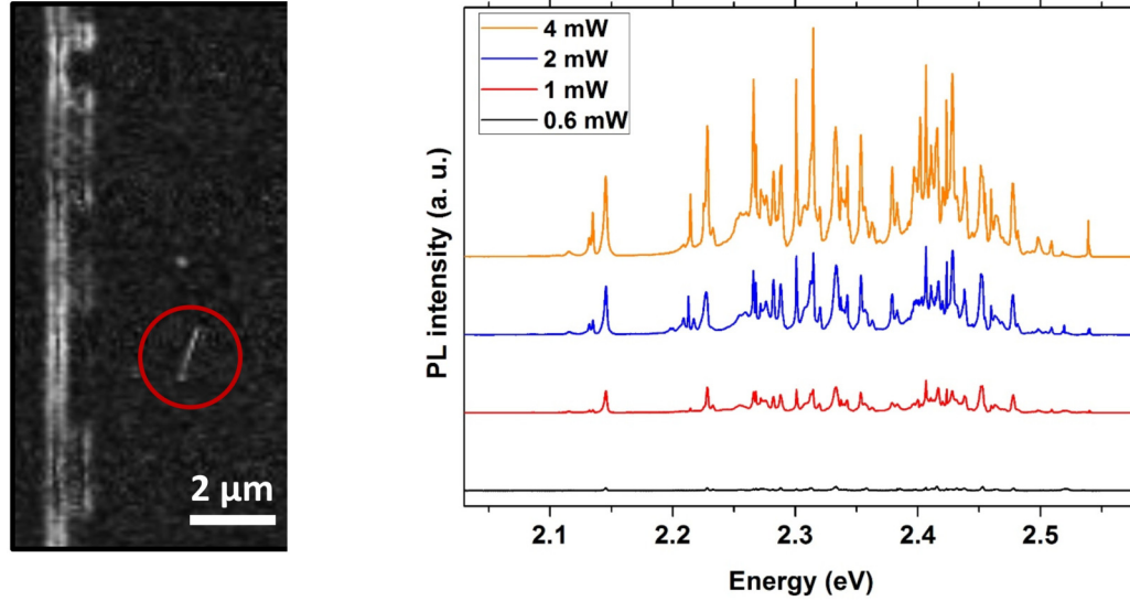
Figure 2.7: Left: Top-view SEM image of a single NW-QD measured by \mu PL (30 s CdSe insertion) and deposited on a patterned substrate. Right: PL spectra of this single NW-QD recorded at 5 K as a function of the 488 nm laser power.
