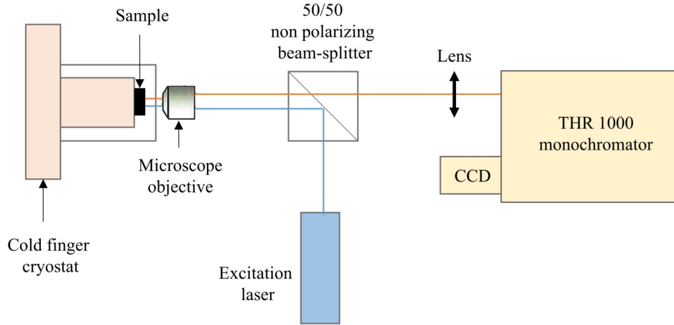
Figure 1.26: Scheme of the \mu PL setup used in this study.
