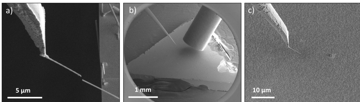
Figure 3.30: Tilted view SEM images (45°) of the micromanipulator tip etched with the FIB down to a 500 nm apex. a) Welding and cut-out of a 50 nm-diameter Ge NW at the apex of the micromanipulator tip. This whole system is then used as a fishing rod to grab the NW-QDs. b) Small pipe used to send tungsten precursor onto the sample to weld thanks to the electron beam and the precursor reaction, forming tungsten. c) Approach of the fishing rod toward the NW-QDs.
