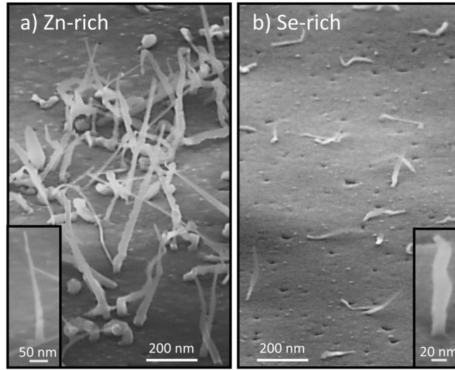
Figure 2.21: Tilted view SEM images (65°) of ZnSe NWs grown on a (111)A substrate at 400°C under a) Zn-rich conditions (Zn:Se of 3:1) and b) Se-rich conditions (Zn:Se of 1:2).
