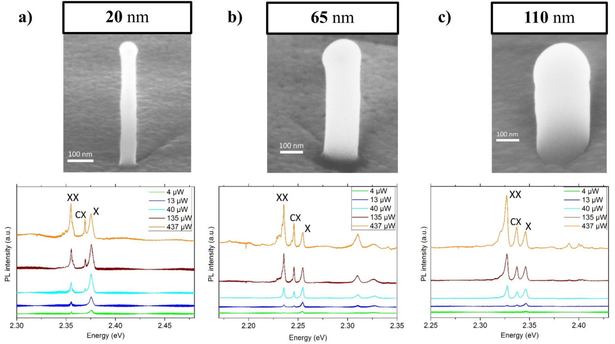
Figure 4.13: (Upper part) Tilted-view SEM images ( 65^\circ ) of photonic wires coated with an \text{Al}_2\text{O}_3 radius of a) 20 nm, b) 65 nm and c) 110 nm. (Bottom part) Corresponding power dependence pPL spectra with a clear excitonic (X, CX and XX) signature of the NW-QD emission. The excitation was carried out at 10 K with a pulsed Fianium WhiteLase Supercontinuum fiber laser tuned at 485 nm (2.556 eV).
