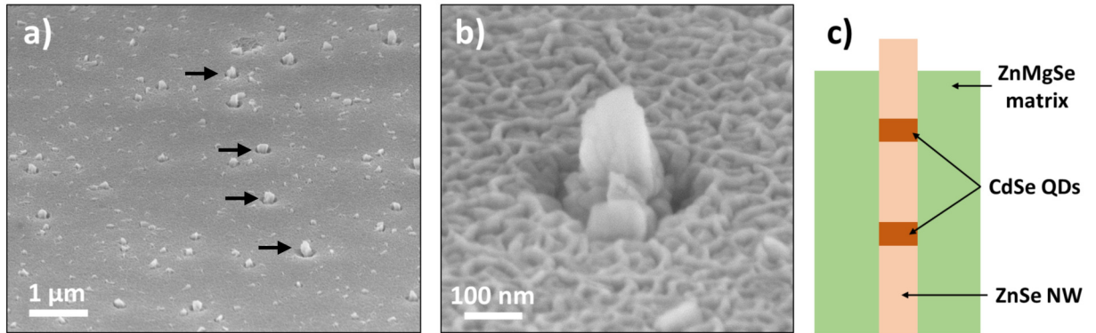
Figure 4.1: Tilted-view SEM images (65°) of the buried NW-QDs sample: ZnSe NWs with two CdSe QD insertions (10 and 20 s) grown at 400°C under Se-rich conditions and a nominal Zn_{0.90}Mg_{0.10}Se shell deposited during 30 min at 220°C. The NW-QDs are almost completely buried and can be recognized thanks to their stone-like ZnMgSe shell head. a) Ensemble (black arrows show some well visible buried NW-QDs), b) zoom on the stone-like head of a single NW-QD and c) side view illustration of the aimed structure.
