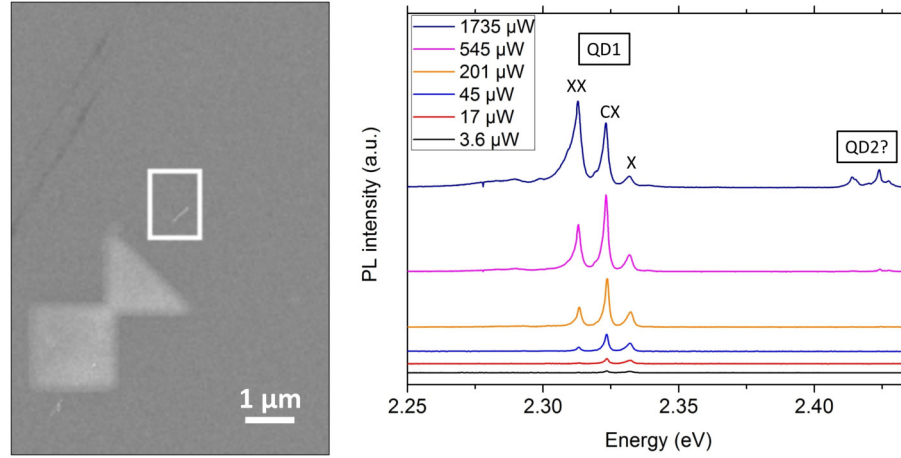
Figure 3.35: Top-view SEM image of a well-isolated single NW-QD from S_{2QDs}^{vacuum} deposited on a patterned substrate and its PL spectra as a function of the 488 nm laser power.
