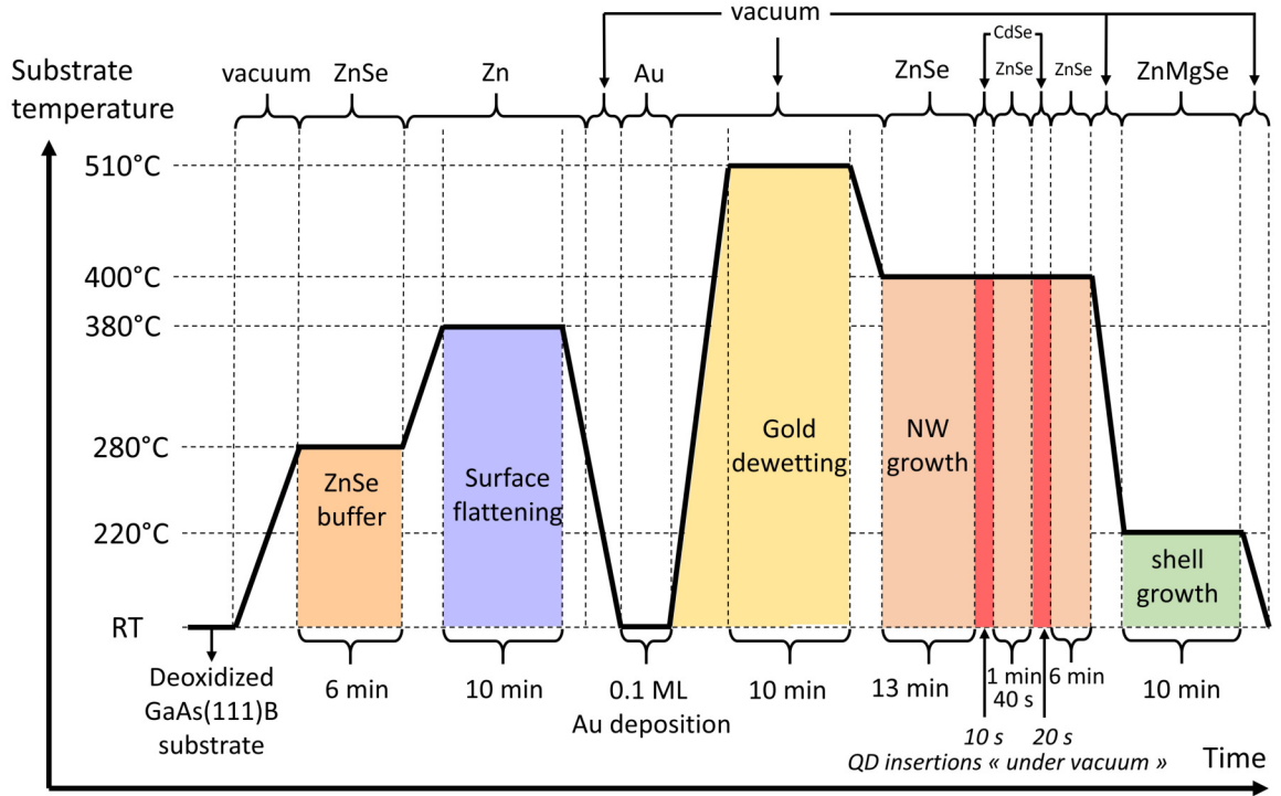
Figure 3.4: Illustration of the growth process of S_{2QDs}^{vacuum} : ZnSe NWs with two CdSe QD insertions of 10 and 20 s grown at 400°C under Se-rich conditions and a nominal Zn_{0.90}Mg_{0.10}Se shell deposited during 10 min at 220°C.
