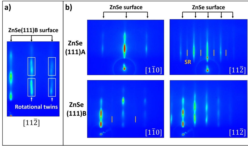
Figure 2.16: Typical RHEED diffraction patterns. a) Highlight of rotational twins along the [11\bar{2}] azimuth characterized by slightly inclined brighter segments along the ZnSe surface vertical streaks. b) Overview of ZnSe(111)A and B layers. Both [1\bar{1}0] and [11\bar{2}] azimuths are displayed. The vertical lines corresponds to the ZnSe(111) surface diffraction (black arrows) and the ZnSe SRs (yellow segments).
