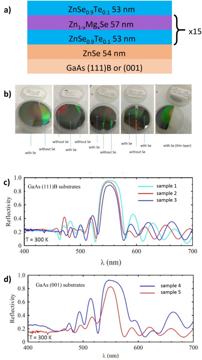
Figure 4.21: a) Sketch of the grown DBR (with x in \text{Zn}_{1-x}\text{Mg}_x\text{Se} ranging from 30 to 60 according to the samples). b) Picture of some of the grown DBR. The zones protected by a Se layer are mentioned. c) and d) Calculated reflectivity of some of these DBR structures grown on the (111)B and (001) surface orientations.
