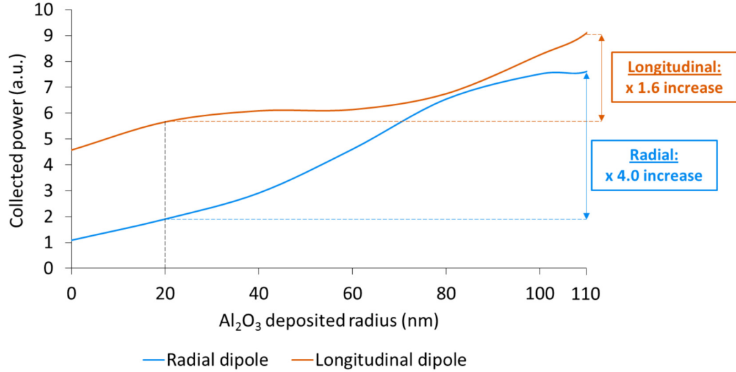
Figure 4.17: Collected power in a 0.6 NA microscope objective from a vertically oriented photonic wire (illustrated in Figure 4.16) for radial and longitudinal dipole orientations. On the right of the Figure, the collected power enhancement between 20 and 110 nm \text{Al}_2\text{O}_3 deposited radii are displayed, with values of 4.0 and 1.6 for the radial and longitudinal dipoles respectively.
