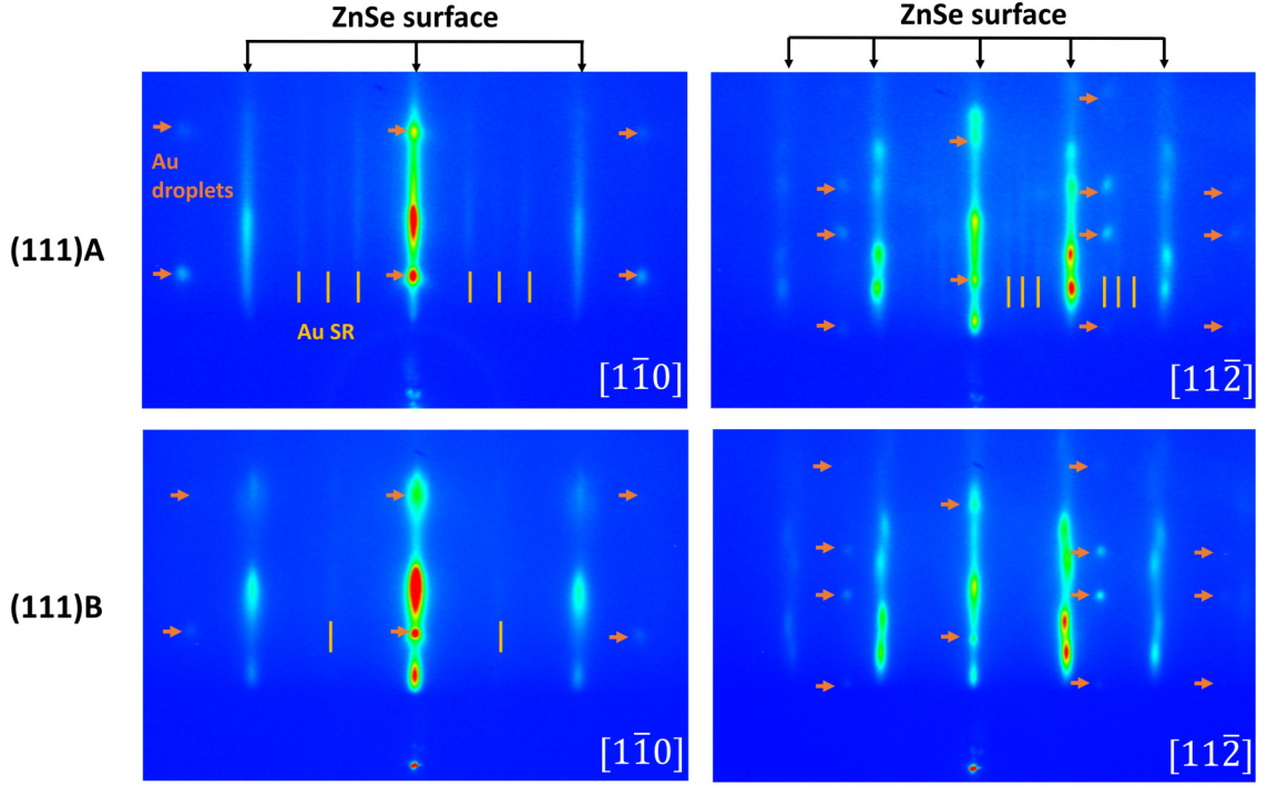
Figure 2.20: Typical RHEED diffraction pattern of ZnSe(111)A and B layers covered with Au particles dewetted at 510°C during 10 min. Both [1\bar{1}0] and [11\bar{2}] azimuths are displayed. The spots indicated with orange arrows highlight the presence of solid Au particles on the surface. The vertical lines corresponds to the ZnSe(111) surface diffraction (black arrows) and Au SRs (yellow lines).
