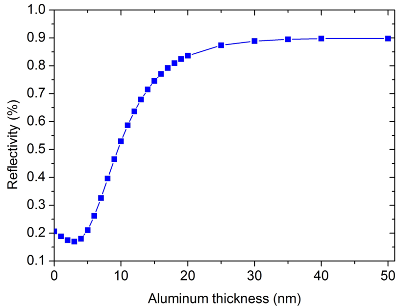
Figure 4.25: Reflectivity of an Al thin film as a function of its thickness. The Al film is deposited on a ZnSe substrate. The Al and ZnSe refractive indexes used are 0.965 + j\ 6.3996 and 2.6628 respectively. This calculation is in good agreement with similar calculations carried out by only considering a layer of Al in Refs. [241, 242].
