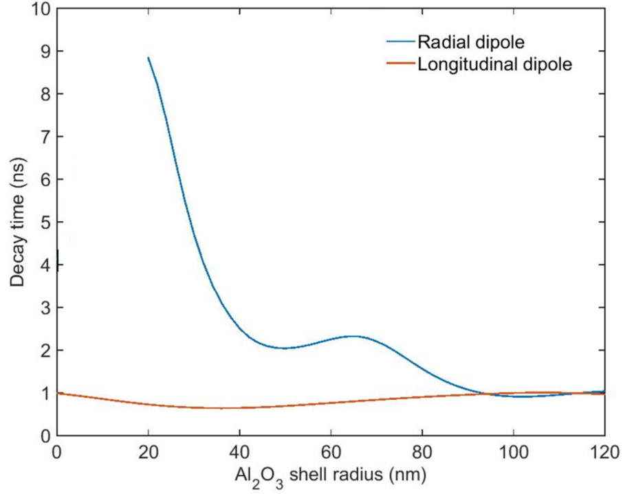
Figure 4.19: Calculated exciton decay-times of radial (blue) and longitudinal (red) dipoles as a function of the \text{Al}_2\text{O}_3 shell radius. These results have been calculated using the analytical Modal method technique.
