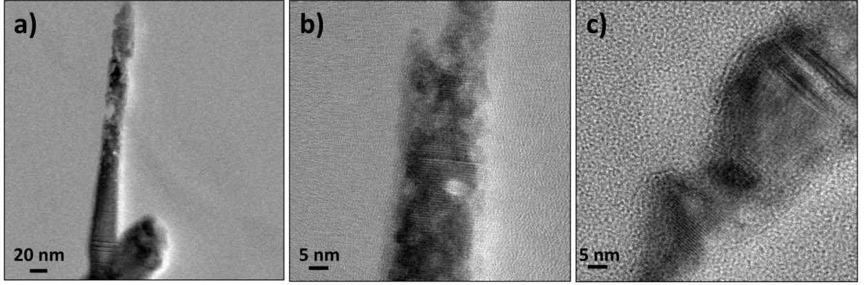
Figure 3.16: TEM images of single NW-QDs from S_{2QDs}^{vacuum} after less than one minute of TEM observation. On the three Figures a, b and c, clear deteriorations can be observed, indicating that the NW-QDs are very prone to TEM electron beam damages.
