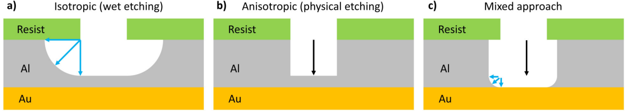
Figure 4.28: Difference between a) an isotropic wet etching and b) an anisotropic physical etching. c) Mixed approach used in this work, which consists in a first physical etching of 20 nm followed by a 10 nm wet etching.
