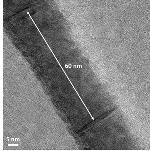
Figure 3.8: TEM image of a single ZnSe NW from S_{2QDs}^{vacuum} with two darker zones attributed to two CdSe insertions. These insertions are very thin (2 to 3 nm along the NW axis while the NW-QD is 29 nm large) and separated by 60 nm.
