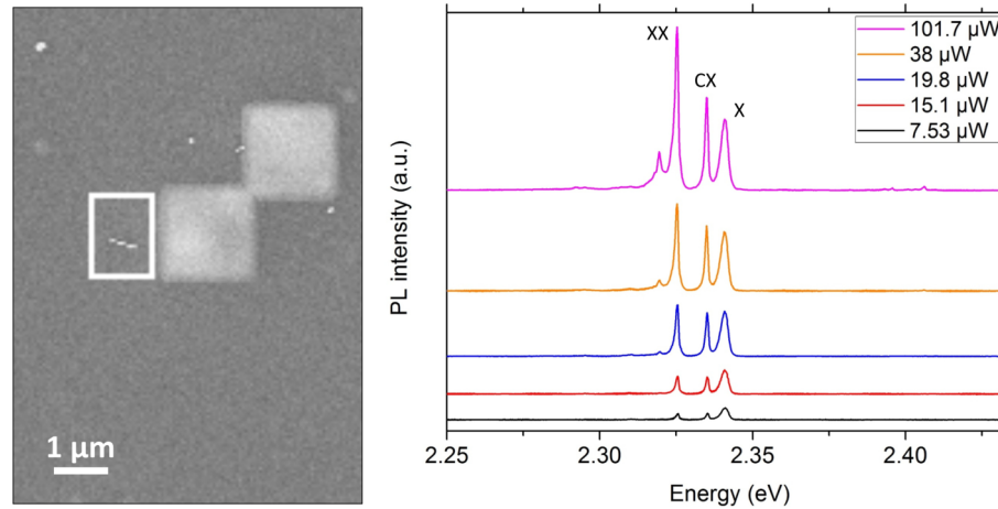
Figure 3.36: Top-view SEM image of a well-isolated single NW-QD from S_{IQD}^{Se} deposited on a patterned substrate and its PL spectra as a function of the 488 nm laser power.
