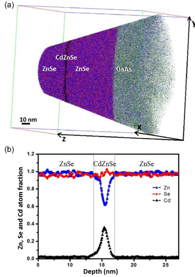
Figure 3.26: a) Reconstructed volume 90 x 90 x 100 nm 3 , showing the ZnSe/ CdSe/ZnSe layers on top of the GaAs substrate. The 3D atom map shows the abrupt interface between layers. b) Concentration profile along the growth direction z measured inside a cylinder of 15 nm-diameter in the reconstructed volume; the average concentration of Cd is about 37 % in the \text{Cd}_x\text{Zn}_{1-x}\text{Se} layer.
