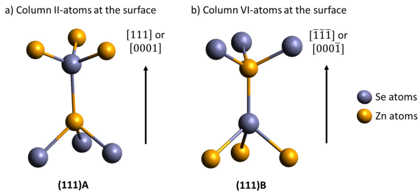
Figure 1.7: Illustrations of a (111)\mathbf{A} (last atomic layer composed of Zn atoms) and a (111)\mathbf{B} (idem with Se atoms) atomic stacking.
