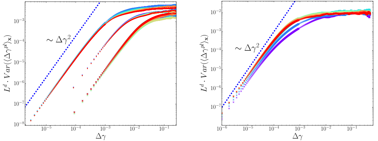
Figure 5.20: Rescaled variance of global plastic strain L^d \cdot Var(\langle \Delta\gamma^{pl} \rangle_{\mathbf{x}}) as function of global strain \Delta\gamma . Left: Shear rate decreases from 10^{-2} to 10^{-4} from bottom to top. \times : \dot{\gamma} = 10^{-2} ; \bullet : \dot{\gamma} = 10^{-3} ; + : \dot{\gamma} = 10^{-4} . Different colors correspond to system sizes L = 32, 64, 128, 256, 512, 1024, 2048 . The collapse is rather good when rescaling with the system size. Large fluctuations at high strain \Delta\gamma are due to lack of statistics. Right: Shear rate \dot{\gamma} = 10^{-5} . The correspondence between the color and the system size is the same as it is in the left panel. Only curves for large system sizes L > 128 collapse well after rescaling with L to the power d . Blue dashed lines show a quadratic growth as a guide to the eye.
