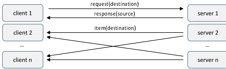
Figure 3.3: CS semantics.
