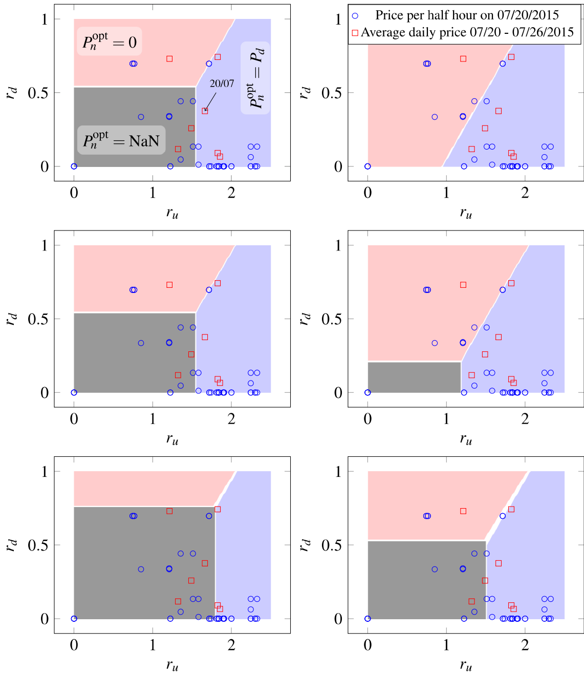
Fig. 3.16 Comparison of feasible regions on r_d \times r_u plane and the optimal x, t = 0.03, C_B = 50, \rho_d = \rho_u = 0.48, \bar{\theta} = 0.3, \gamma = 0.05 for the first row, \bar{\theta} = 0.1, \gamma = 0.05 for the second, and \bar{\theta} = 0.1, \gamma = 0.5 for the third.
