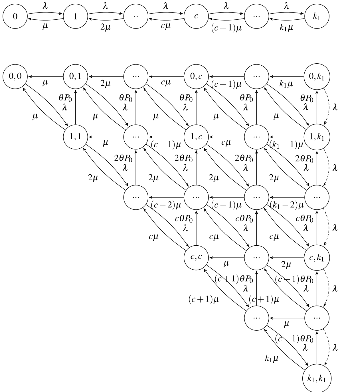
Fig. 4.2 Continuous-Time Markov Chains describing the evolution of the number of plugged EVs m_t (top) and of (n_t, m_t)=(nb\_discharging\_EVs, nb\_plugged\_EVs) (bottom). Both are for Scheme 1
