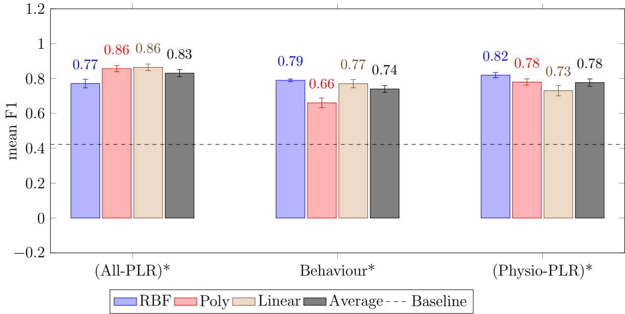
Figure 6.3: Performances of each kernel for each modality for the prediction of PEA without using features related to HRV. The baseline average F1 score obtained by a random classifier is 0.422 (\pm 0.080) .
