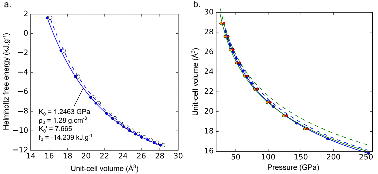
Figure 4.9: Equation of state of NaCl B2 phase at 1600 K. a. Specific Helmholtz free energy as function of the B2 unit-cell volume. The open circles correspond to the free energy computed from our simulations and the dashed blue line is the fit of a Vinet equation of state to these data. The blue dots and the blue continuous line respectively represent our data corrected from the GGA volume overestimation and the associated Vinet EOS fit. b. Volume – pressure relations in B2 NaCl. The orange and red dots correspond to experimental data obtained at 1000 K and 2000 K (Nishiyama et al., 2003). The dashed blue line represents the pressures given by the derivation of the non-GGA-corrected fit of the Helmholtz free energy. The volume difference between this curve and the experimental data is due to the overestimation of the volumes by the GGA. To obtain the continuous blue line we reduce all the volumes by \Delta V_{\text{GGA}} = 0.3 \text{ \AA}^3/\text{unit-cell} . The blue dots refer to the non-quantum-corrected pressures p_{\text{MD}} obtained from our simulations whose corresponding volumes have been corrected by \Delta V_{\text{GGA}} . GGA-corrected and non-corrected theoretical equations of state from Ono et al. (2008) are respectively represented by green continuous and dashed lines.
