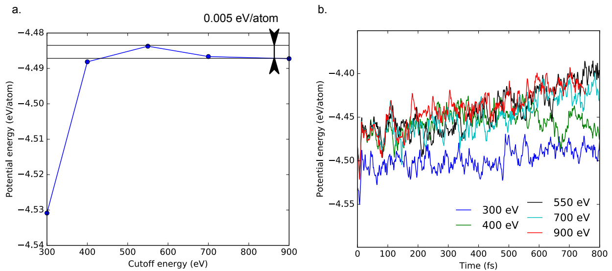
Figure A.1: a. Evolution of the potential energy as function of the cutoff energy for the plane-wave basis set in \text{H}_2\text{O} at \rho = 2.453 \text{ g.cm}^{-3} . b. Evolution of the potential energy as a function of time for different cutoff energies. These short molecular dynamics simulations are performed in the isokinetic ensemble at 1600 K with a time step of 1 fs and at \rho = 2.453 \text{ g.cm}^{-3} in \text{H}_2\text{O} ; the system is still in the thermalization phase. For the molecular dynamics simulations we choose a cutoff energy equal to 550 eV that leads to an error of 5 meV/atom. We obtain the same accuracy in NaCl-bearing systems. This error is three time smaller than the energy variations that occurs during the molecular dynamics simulations in the production run. We perform the ionic relaxation of the dislocation quadrupoles at 0 K using a cutoff energy of 875 eV. In this case the energy is converged within 1.10^{-5} \text{ eV/atom} .
