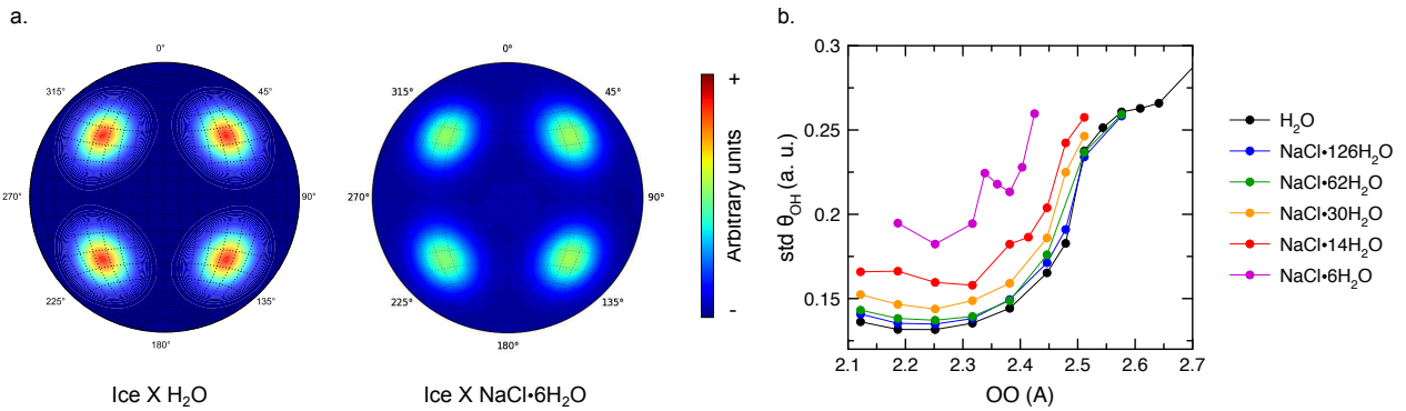
Figure 4.5: Orientational disorder induced from the inclusion of NaCl. a. Stereographic representation for the spatial distribution of O – H bonds orientations in pure and NaCl-bearing ice X at 1600 K and OO \sim 2.19 Å. The color scale is the same for the two projections. b. Standard deviation of the O – H orientation, i.e. quantitative estimation of the dispersion of the O – H orientation around the \langle 111 \rangle directions.
