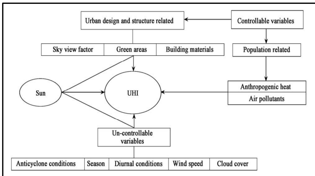
Figure (2-5): Generation of Urban Heat Island (Rizwan et al., 2008).
