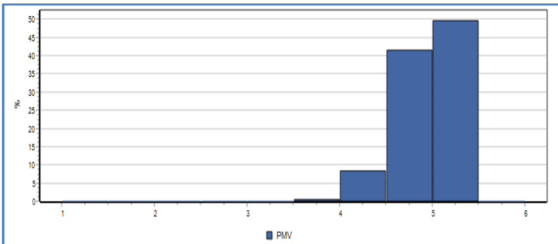
Figure (5-31): Percentage value of PMV for Haifa Street at noon, at 1.5 m above the ground.
