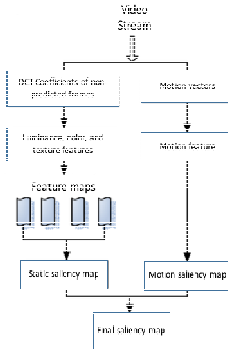
Figure II-17: Flowchart of the saliency computation model [FAN14]: the visual saliency is extracted from the transformed domain of the MPEG-4 ASP.
