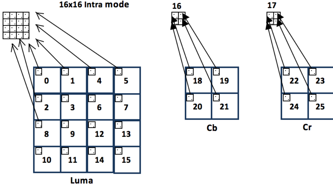
Figure B-5: Block construction for DCT and Hadamard transformations.
