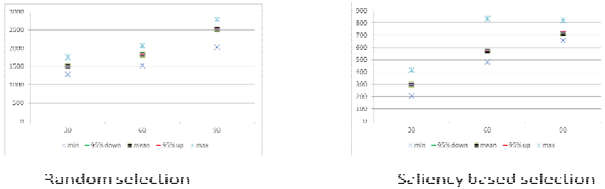
Figure E-3: DVQ results of the objective quality evaluation when alternatively considering random selection and saliency map based selection corresponding to DVQ results in Table III-9.
