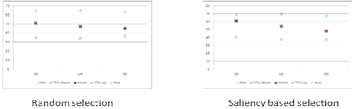
Figure E-1: PSNR results of the objective quality evaluation when alternatively considering random selection and saliency map based selection corresponding to PSNR results in Table III-9.
