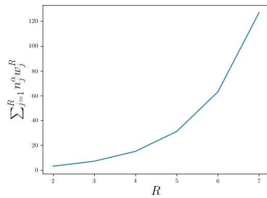
(b) \alpha = 1 .
