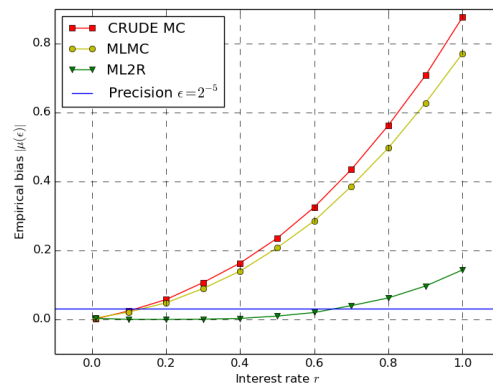
(b) Milstein scheme ( \alpha = 1, \beta = 2 ).
