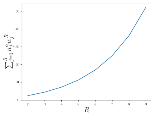
(a) \alpha = 0.5 .
