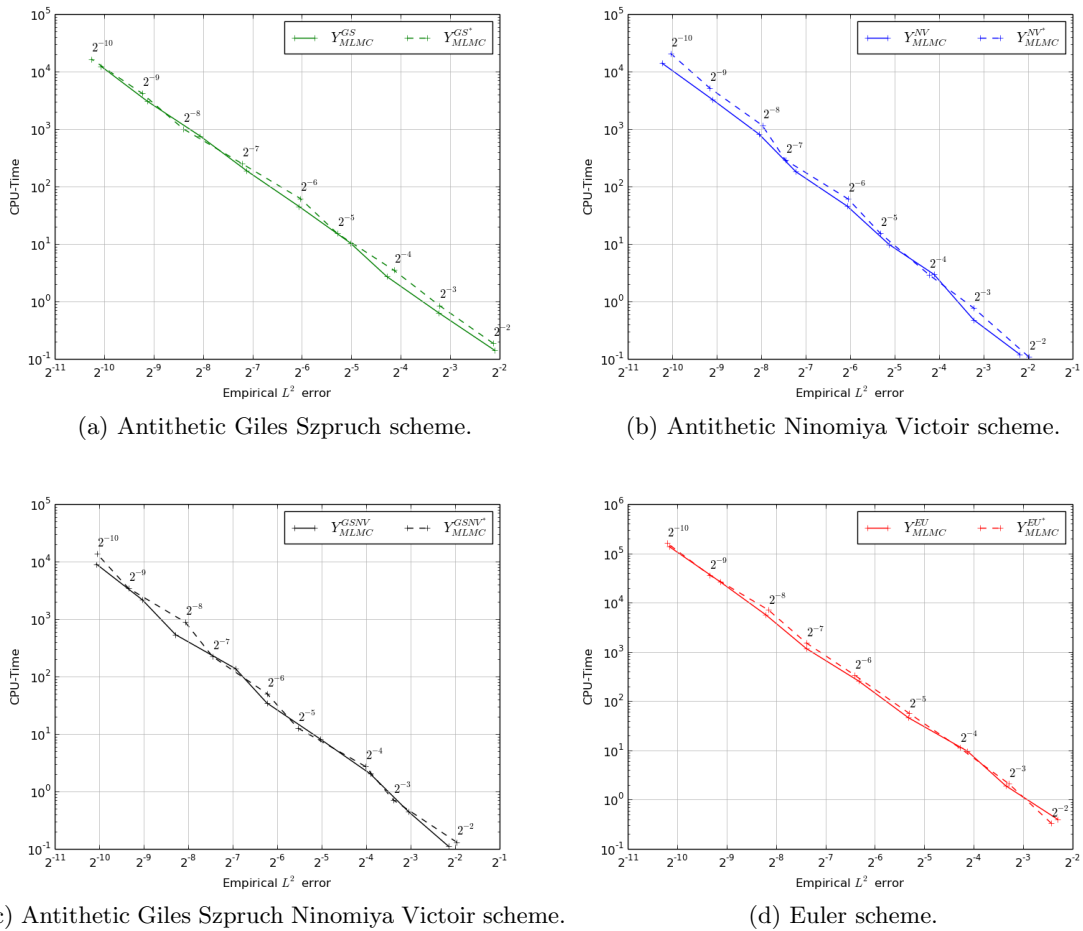
FIGURE 3.1 – CPU time vs empirical error for MLMC estimator calibrated with Table 3.2 or with formulas (3.23) and (3.24). Clark-Cameron model with U_0 = S_0 = 0 , T = 1 and \mu = 1 . Payoff function f(u, s) = 10 \cos(u) .
