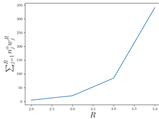
(c) \alpha = 2 .
