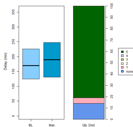
Figure 5.6: Adaptive Packetization
