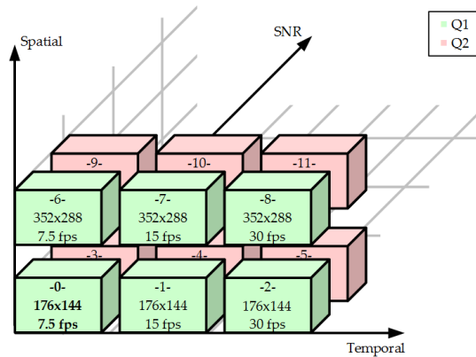
Figure 4.9: SVC Layers
