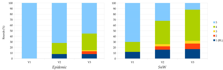
Figure 4.15: Quality Distribution
