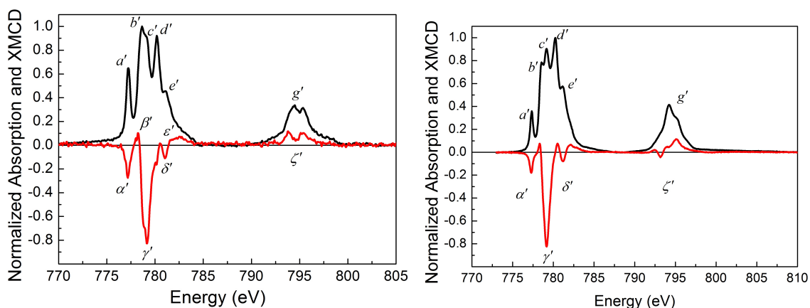
Figure 4.15 – Experimental XAS (black line) and XMCD (red line) spectra at the Co L_{2,3} edges in sample 1 (dinuclear complex, left) and sample 3 (Co precursor of 1 , right) at T = 4 K and \mathbf{B} = 6.5 T.
