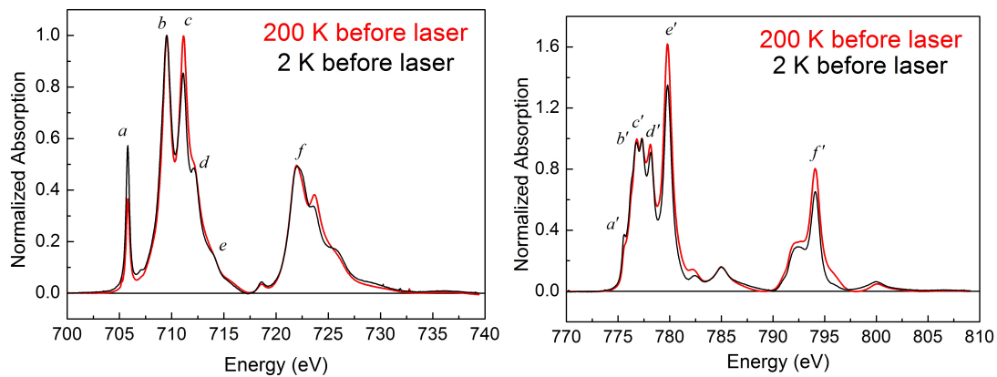
Figure 5.9 – Experimental XAS spectra at Fe (left) and Co (right) L_{2,3} edges at 200 K (red line) and at 2 K before laser irradiation (black line).
