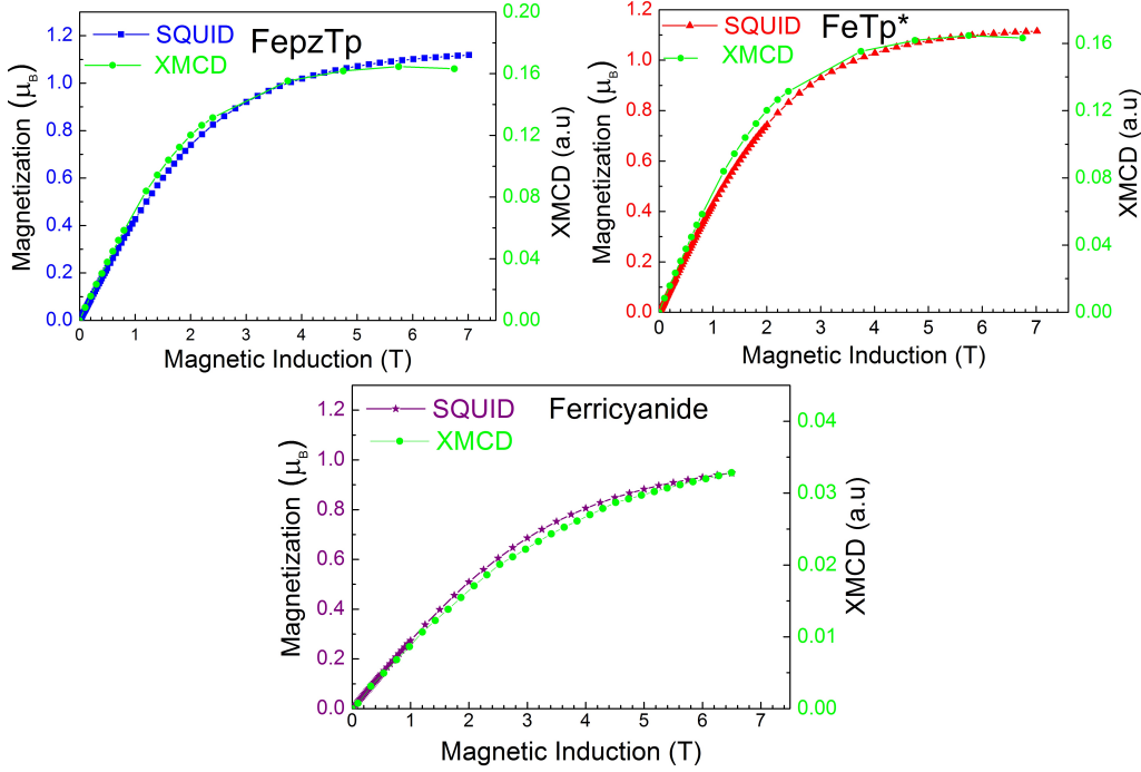
Figure 3.14 – Comparison of XMCD detected magnetization curves (light green line) at T = 2 K with 6.5 T and SQUID measurements (top left) for FepzTp ( \text{NEt}_4 )[(pzTp) \text{Fe}^{\text{III}}(\text{CN})_3 ] (blue), (top right) for FeTp* ( \text{NEt}_4 )[(Tp*) \text{Fe}^{\text{III}}(\text{CN})_3 ] (red line), and (bottom) for Potassium hexacyanidoferrate(III) \text{K}_3[\text{Fe}^{\text{III}}(\text{CN})_6] (purple line).
