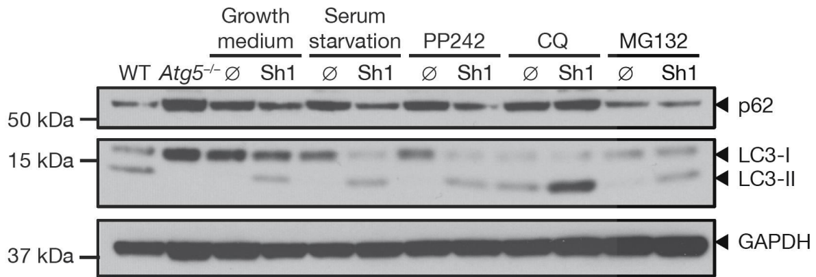
Figure 11: Basal autophagy is restored and autophagy can be stimulated in Shield1-treated ATG5 DD cells.
