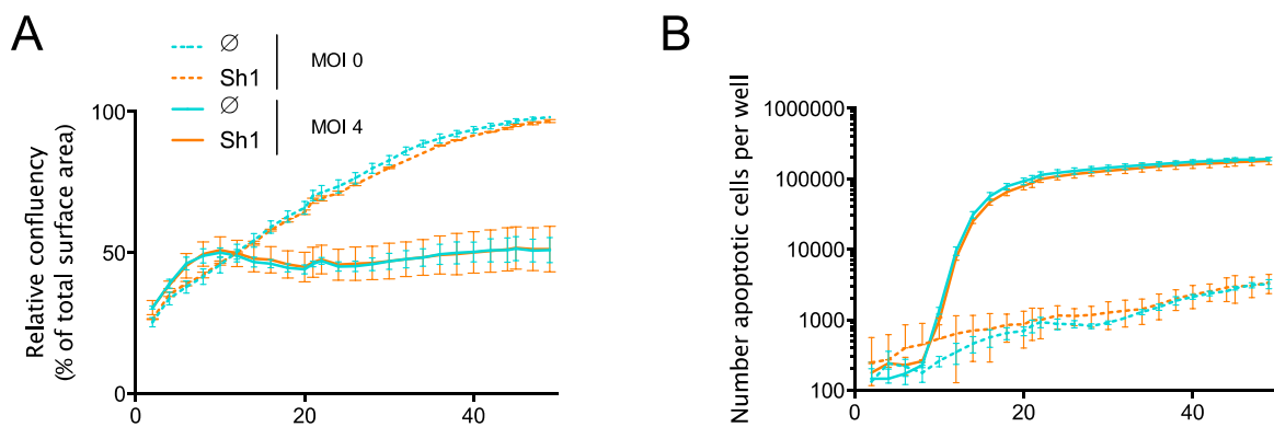
Figure 20: Autophagy capacity does not impact apoptosis levels after infection. ATG5 DD -expressing Atg5 -/- cells, pre-treated or not with Shied1 (Sh1), were infected with IAV at MOI 4 and images were obtained every hour for 50 h to assess cell growth ( A ) and apoptotic cell number ( B ). Points depict mean relative confluency at interval time and error bars depict standard deviation.
