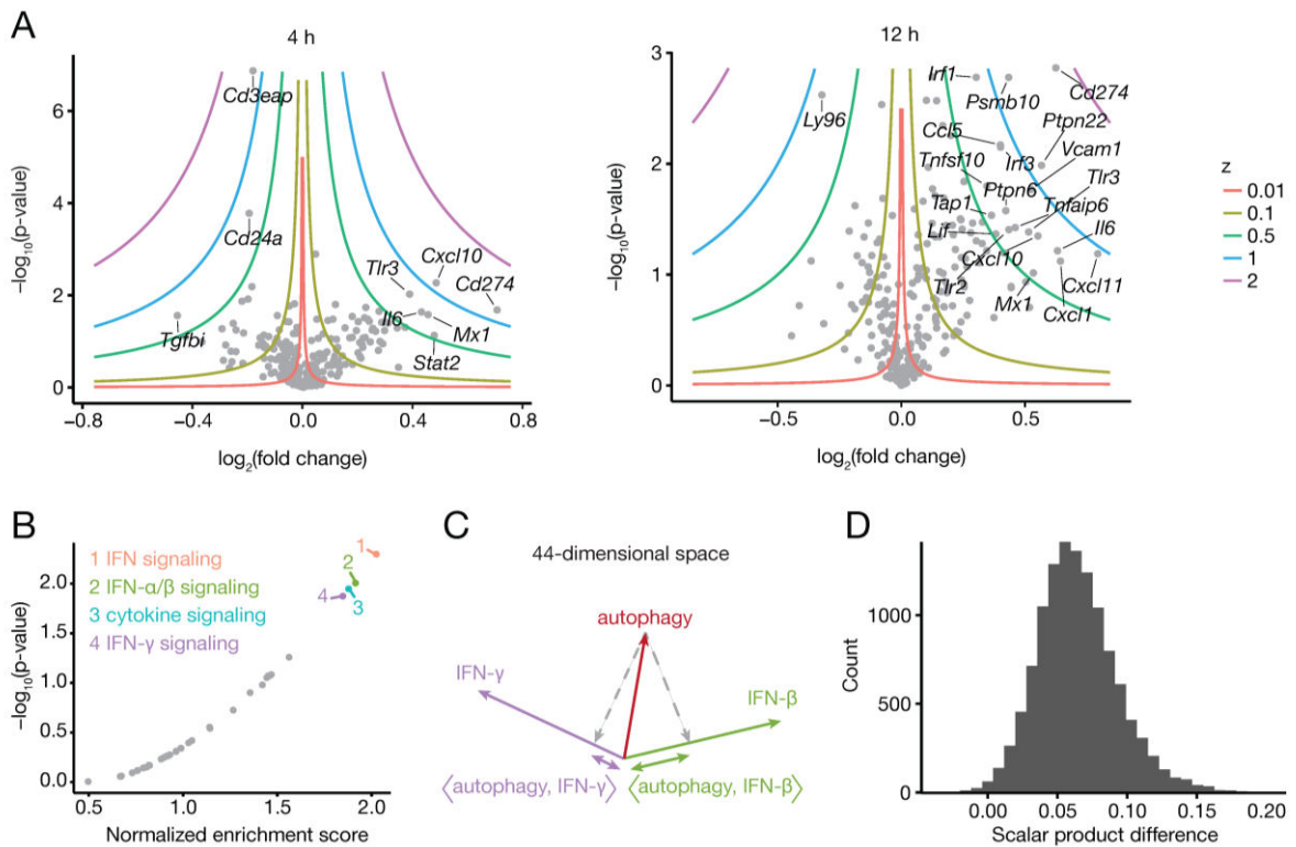
Figure 22: IAV-induced expression of type I IFN-stimulated genes is reduced when ATG5 DD is stabilized.
