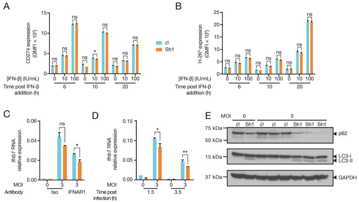
Figure 25: Autophagy inhibits ISG expression via cell-intrinsic modulation of IFN- \beta expression and not through desensitization to IFNAR signaling.
