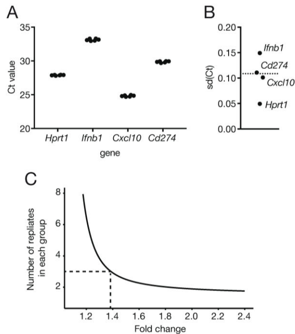
Figure 26: Detection power of RT-qPCR for Hprt1 , Ifnb1 , Cxcl10 and Cd274 .
