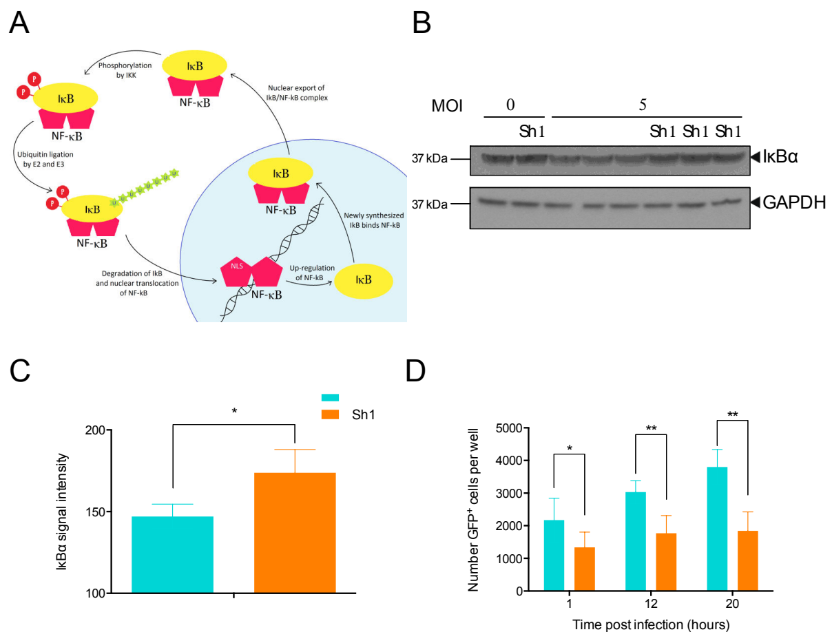
Figure 27: Activation of the NF- \kappa B pathway is negatively impacted by autophagy. (A) NF- \kappa B activation, involves I \kappa B phosphorylation, ubiquitination and proteasomal degradation, which frees NF- \kappa B and allows it to translocate to the nucleus for stimulation of transcription. (from sites.tufts.edu). (B,C) ATG5 ^{DD} cells pre-treated or not with Shield1 (Sh1) were infected by PR8 for 1 h before monitoring I \kappa B \alpha degradation by immunoblot (B) and quantification with ImageJ (C). ATG5 ^{DD} cells transfected by with NF- \kappa B transcription activity GFP reporter for 20 hours were pre-treated or not with Shield1 (Sh1) and infected by PR8. Incucyte intra-incubator microscope allowed the monitoring of GFP positive cell number.
