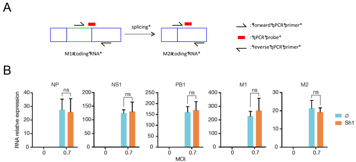
Figure 17: IAV RNA expression is not impacted by autophagy capacity.
