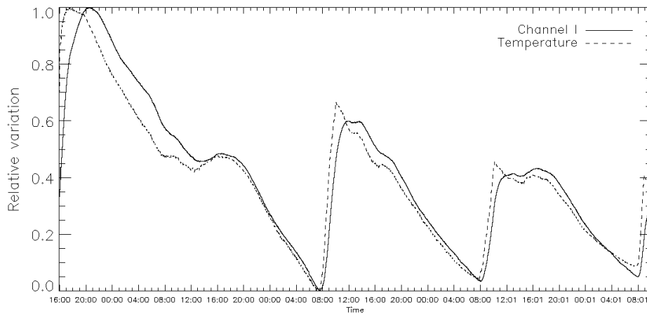
Figure 4. Relative channel I position and temperature variation as a function of time.
