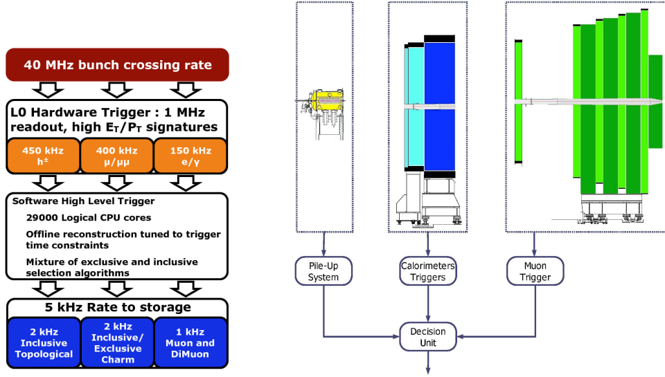
Figure 2.21 – (Left) Overview of the LHCb trigger system in 2012, along with the allowed rates for each line. (Right) Detector subsystems involved in the L0 trigger decision.
