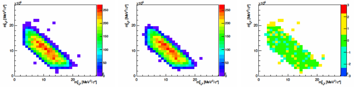
Figure C.2 – Distributions of m_{K_S^0 h}^2 versus m_{K_S^0 h'}^2 for the B^0 \rightarrow K_S^0 \eta mode, with DD reconstruction of the K_S^0 . Left: Reconstructed events. Middle: Fast MC events. Right: Pulls between the two distributions.
