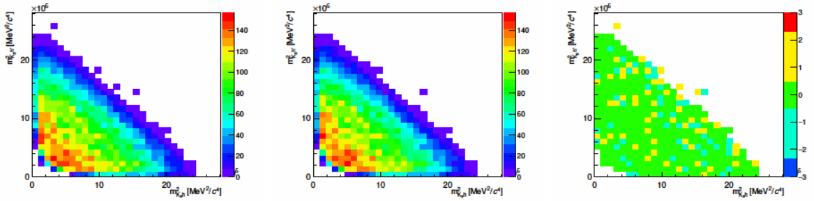
Figure C.6 – Distributions of m_{K_S^0 h}^2 versus m_{K_S^0 h'}^2 for the B^+ \rightarrow K^{*+} \pi^+ \pi^- mode, with DD reconstruction of the K_S^0 . Left: Reconstructed events. Middle: Fast MC events. Right: Pulls between the two distributions.
