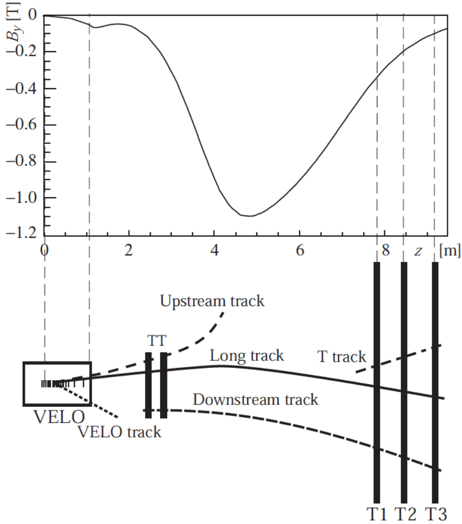
Figure 2.15 – Types of track in LHCb, along with the magnetic field as a function of z [58]. Muon tracks that only leave hits in the muon stations are not shown.
