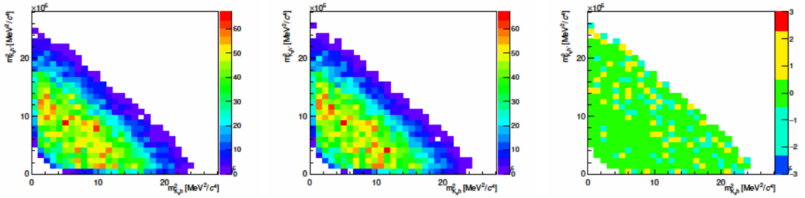
Figure C.4 – Distributions of m_{K_S^0 h}^2 versus m_{K_S^0 h'}^2 for the B^0 \rightarrow K_S^0 \pi^+ \pi^- \gamma mode, with DD reconstruction of the K_S^0 . Left: Reconstructed events. Middle: Fast MC events. Right: Pulls between the two distributions.
