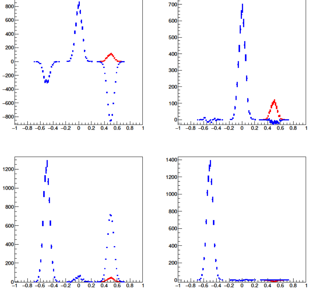
Figure A.5 – Distribution of Y in data samples sWeighted according to signal (combinatorial) weights. Results of the approach A(B) are shown on the left (right). The red points correspond to the distribution of the sum of sWeights, whereas the blue points represent the final distribution (after correction using Eq. A.6).
