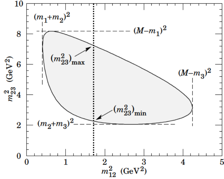
Figure 1.5 – Typical Dalitz plot, along with kinematical boundaries [4].
