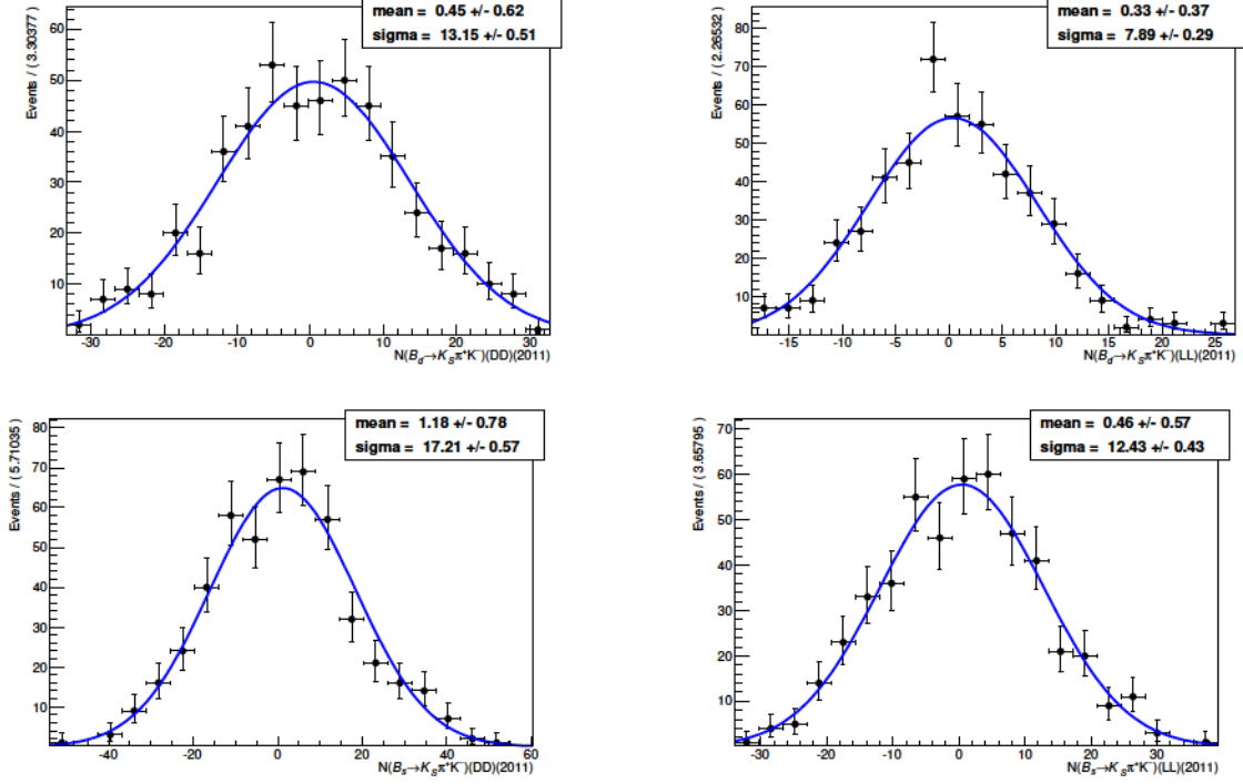
Figure 4.12 – Residuals distributions for yields of K_s^0 \pi^+ K^- 2011 signals. Top: B^0 \rightarrow K_s^0 K^- \pi^+ signal, bottom: B_s^0 \rightarrow K_s^0 K^- \pi^+ signal. Left: Down-Down, right: Long-Long.
