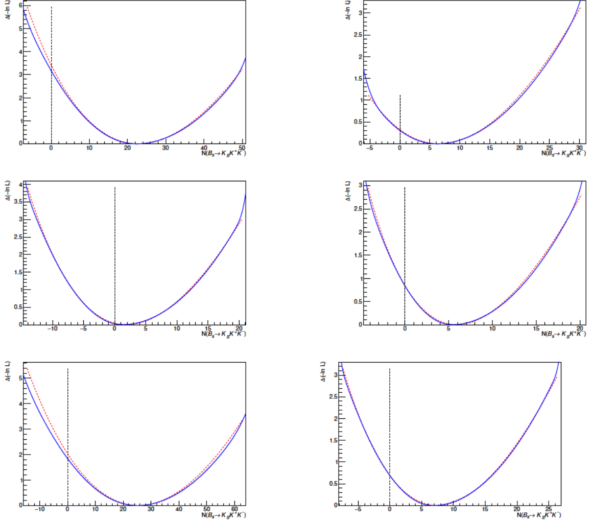
Figure 4.18 – Likelihood scans of B_s^0 \rightarrow K_s^0 K^+ K^- yields. The blue line indicates the total likelihood (including systematics), whereas the red, dotted line is statistical only. The dashed, vertical line indicates the N(B_s^0 \rightarrow K_s^0 K^+ K^-) = 0 hypothesis. Left: Down-Down K_s^0 reconstruction mode. Right: Long-Long K_s^0 reconstruction mode. Different data-taking periods are shown on top (2011), middle (2012 pre-June), and bottom (2012 post-June).
