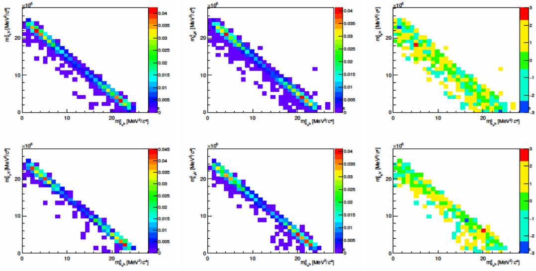
Figure 3.12 – Left: Distributions of fully simulated B^0 \rightarrow K^{*0} \rho^0 events with Down-Down (top) and Long-Long (bottom) K_S^0 reconstruction mode over the Dalitz plane. Middle: Distributions of fast Monte-Carlo B^0 \rightarrow K^{*0} \rho^0 events with Down-Down (top) and Long-Long (bottom) K_S^0 reconstruction mode over the Dalitz plane. Right: Pulls between the two distributions with Down-Down (top) and Long-Long (bottom) K_S^0 reconstruction mode.
