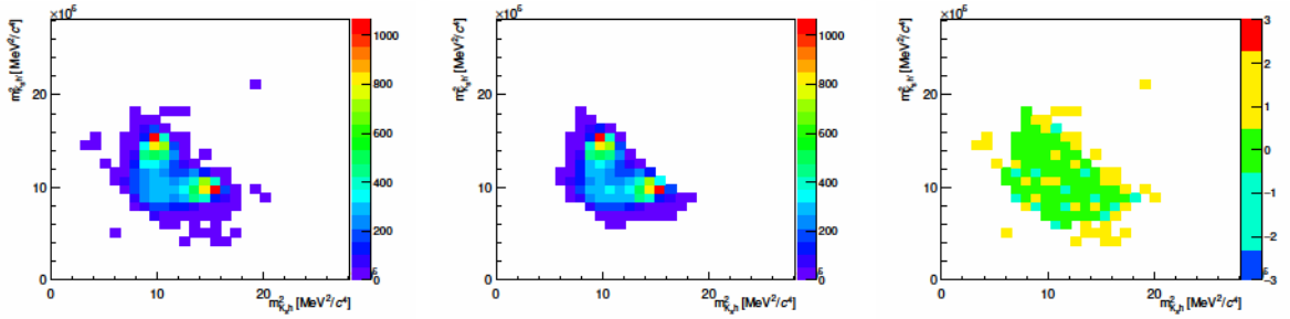
Figure C.10 – Distributions of m_{K_S^0}^2 versus m_{K_S^0 h'}^2 for the B^+ \rightarrow K^{*+} \phi mode, with DD reconstruction of the K_S^0 . Left: Reconstructed events. Middle: Fast MC events. Right: Pulls between the two distributions.
