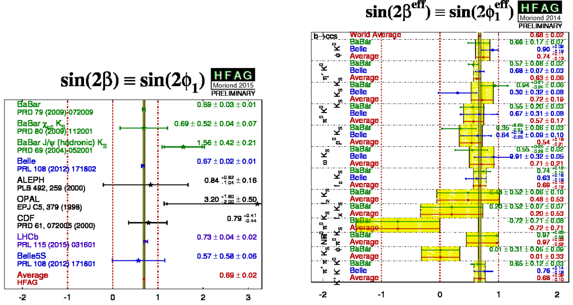
Figure 1.4 – World average of \beta from [19], extracted from b \rightarrow c\bar{c}s decays (left) and b \rightarrow q\bar{q}s decays (right). The world average from b \rightarrow c\bar{c}d is also indicated in the right hand-side figure.
