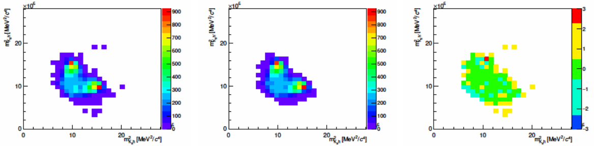
Figure C.8 – Distributions of m_{K_S^0}^2 versus m_{K_S^0 h'}^2 for the B^0 \rightarrow K^{*0} \phi mode, with DD reconstruction of the K_S^0 . Left: Reconstructed events. Middle: Fast MC events. Right: Pulls between the two distributions.
