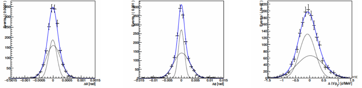
Figure 3.3 – Fit results for p_z ( \pi^+ ) between 8.5 GeV/ c^2 and 11.5 GeV/ c^2 . Left: \Delta\theta(\pi^+) . Middle: \Delta\phi(\pi^+) . Right: \Delta_{1/p_z}(\pi^+) .
