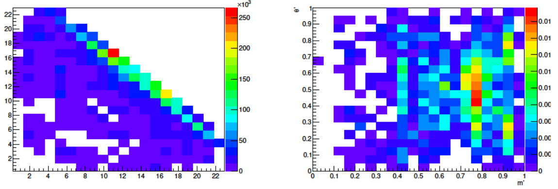
Figure 5.13 – Distribution of data events from all data-taking periods and K_S^0 reconstruction modes over the Dalitz plot (left) and the square Dalitz plot (right).
