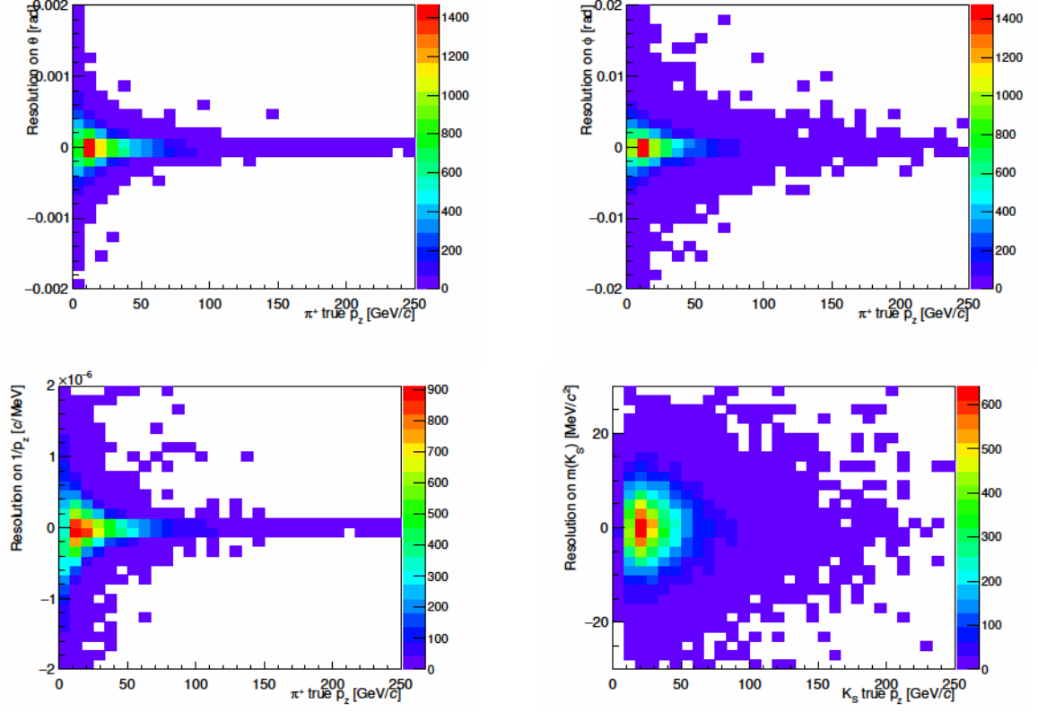
Figure 3.2 – Distributions versus p_z of \Delta\theta (top, left), \Delta\phi (top, right), and \Delta_{1/p_z} (bottom, left) for \pi^+ , and distribution of \Delta m_{K_S^0} versus p_z (bottom, right).
