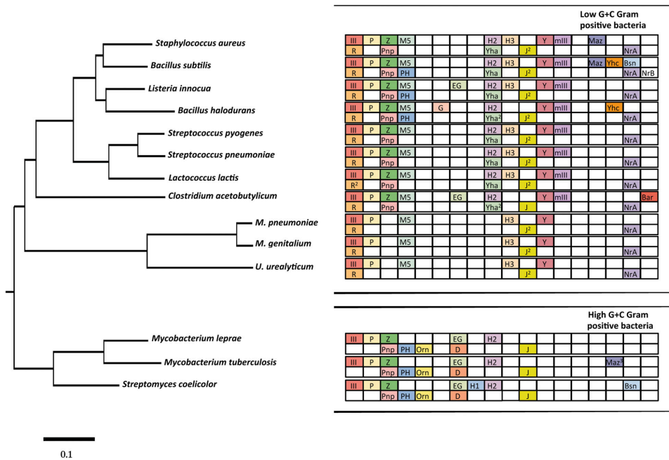
Figure 2. The phylogenetic distribution of Gram-positive ribonucleases. The endonucleases are shown in the top row and the exonucleases in the bottom row of blocks for each species. The phylogenetic relationship between the different organisms was calculated by comparing 16S rRNA sequences using Clustal X. The phylogenetic tree was drawn using Phylodendron ( http://iubio.bio.indiana.edu/soft/molbio/java/apps/trees/ ). The abbreviations for the different RNases are as follows: III = RNase III; P = RNase P; Z = RNase Z; M5 = RNase M5; G = RNase G; EG = RNase E/G; H1 = RNase H1; H2 = RNase H2; H3 = RNase H3; Y = RNase Y; mIII = MiniRNase III; Maz = MazF/EndoA; Yhc = YhcR; Bsn = RNase Bsn; Bar = Barnase; R = RNase R; II = RNase II; Pnp = polynucleotide phosphorylase; PH = RNase PH; Om = oligoribonuclease; T = RNase T; D = RNase D; Yha = RNase Yha; J = RNase J; NrA = NanoRNase A; NrB = NanoRNase B. *Number potential orthologues present. This figure is an updated version of a figure shown in Condon and Putzer (2002).
