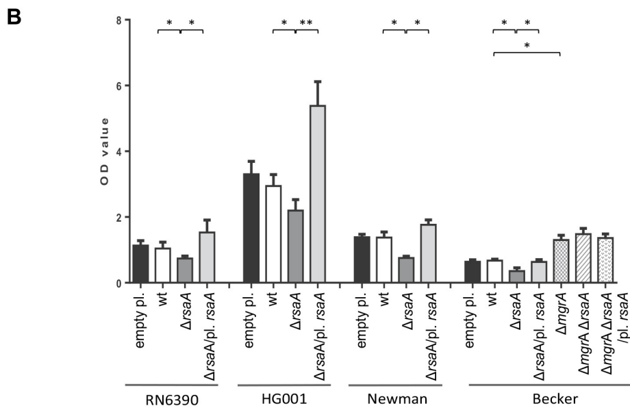
Figure 5. Effect of RsaA on biofilm formation. (A) Kinetics of the early phase of biofilm formation in different S. aureus backgrounds with the Biofilm Ring Test at different incubation times. Standardized bacterial cultures were incubated in 96 well micro-titer plate in the presence of magnetic beads at 37°C. A plate reader measures the number of beads in each well before and after magnetization. The beads are gathered in the center of the well if no biofilm is formed whereas the beads are dispersed if they are immobilized into the biofilm. The Biofilm Forming Index (BFI) corresponds to the mobility of beads under magnet action. Results are expressed as the DBFI corresponding to the difference between a control well (without bacteria) and the studied sample. A value of DBFI \geq 7 means that the biofilm is formed. Data obtained for each strain were shown with a color code as given in the figure: blue for the parental wild-type (RN6390, Newman, Becker) strains, red for the DrsaA mutant strain, and green for the complemented strain expressing RsaA from a plasmid. (B) Analysis of the mature biofilm formation with crystal violet staining. Overnight bacterial cultures were standardized and incubated 24 h at 37°C in rich medium supplemented with glucose 0.25%. The mature biofilm was stained by crystal violet 0.1%, released with acetic acid 33%, and quantified by OD 570 nm . The mean and the standard deviations are presented on the histogram. Statistical differences * (p < 0.05) and ** (p < 0.005) between each strains were obtained by using Anova test. doi:10.1371/journal.ppat.1003979.g005
