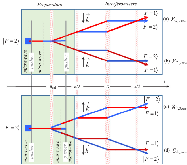
FIG. 2. Different preparation sequences, with two or three microwave pulses, corresponding to input states in |F = 1\rangle or |F = 2\rangle . The corresponding interferometer configurations with the trajectories along the two interferometer paths are also displayed.
