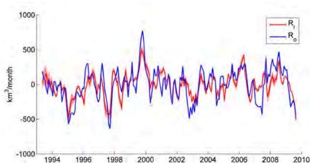
Fig. 8. Comparison of runoff computed from land–atmosphere ( R_1 ) and ocean–atmosphere ( R_o ) water budgets. The red shading represents discrepancies relative to the different considered LSMs.
