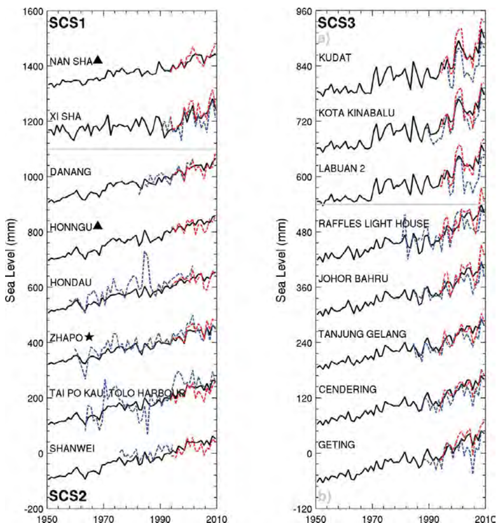
Figure 11. Sea level curves at tide gauge sites since 1950. Time series of MRESL (black), tide gauge (blue), and altimetry-based sea level (red). The time series were arranged in 3 groups: SCS1, SCS2, and SCS3. (Color figure available online.)
