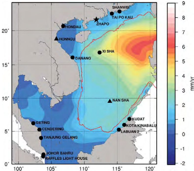
Figure 5. Map of steric sea level trends over the SCS during 1993–2009. (Color figure available online.)
