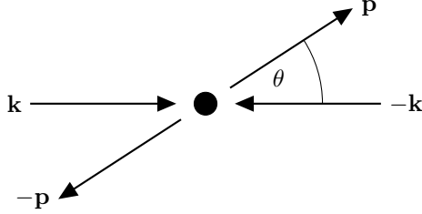
Figure 2.3: Elastic center-of-mass scattering of two scalar particles. When a spin- j resonance dominates the scattering process, the amplitude is proportional to P_j(\cos \theta) .
