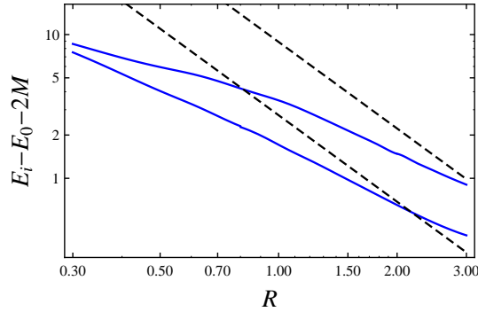
Figure 7.10: Blue curves: E_i - E_0 - 2M for the lowest two orbital excitations in the two-particle sector of the \lambda = 0.3 spectrum corresponding (log-log scale). We excised by hand a state which asymptotes to 4M and thus looks like a four-particle state at rest. Dashed black lines: 2(\Delta M_{\text{curv}} + \Delta M_l) for l = 1, 2 .
