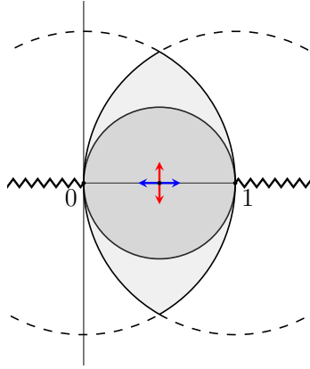
Figure 1.3: Light shaded area: domain of convergence of the conformal blocks in the z -plane. Dark shaded area: domain of convergence of the series expansion around z = 1/2 . Zigzag lines: branch cuts of the conformal blocks. The arrows indicate how the Taylor expansion around z = 1/2 must be understood.
