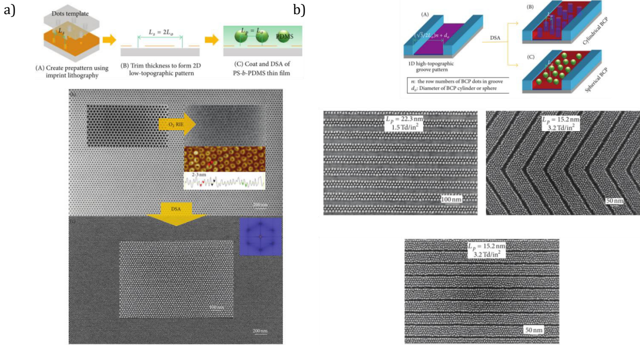
Figure 1-20: (a) Schematic representation of directed self-assembly of sphere-forming PS- b -PDMS thin films by a 2D low-topographic holes array resist prepattern with L_p=2L_0 and corresponding SEM top view images. (b) Schematic representation of directed self-assembly of sphere-forming PS- b -PDMS thin films by a 1D high-topographic groove pattern and corresponding SEM images (top L_0=22.3 nm, bottom L_0=15.2 nm) 87
