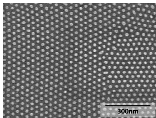
Figure 3-7: SD42 self-assembly by the DOS plasticizer effect. DOS was evaporated in a vacuum chamber ( \sim 13 mPa) for 5 minutes, immediately followed by the two-step plasma etching for PS removal and PDMS oxidizing
