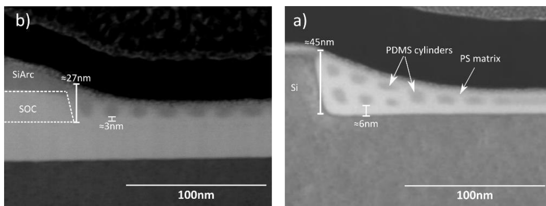
Figure 4-2 cross section STEM images of SD16 after annealing in a) SiArc/SOC and b) PS-brushed silicon trenches
