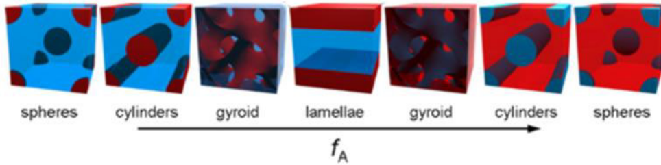
Figure 1-10: Schematic representation of different morphologies of a diblock copolymers depending on the volume fraction of block A 25
