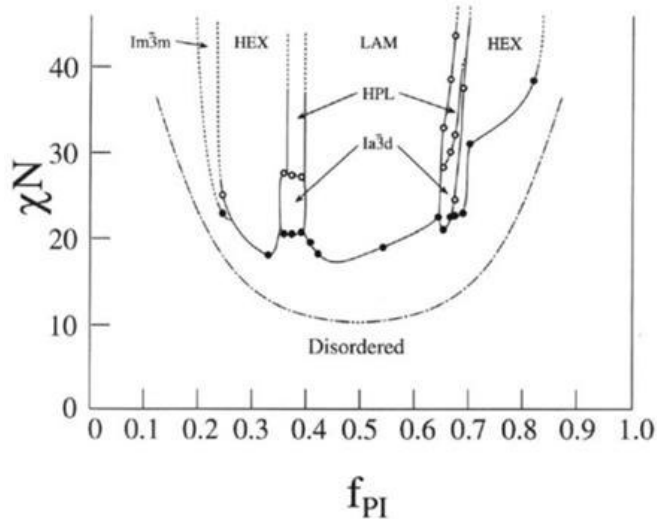
Figure 1-11: Experimental phase diagram of PS-PI 26 . Lm3m and la3d are crystallographic space groups
