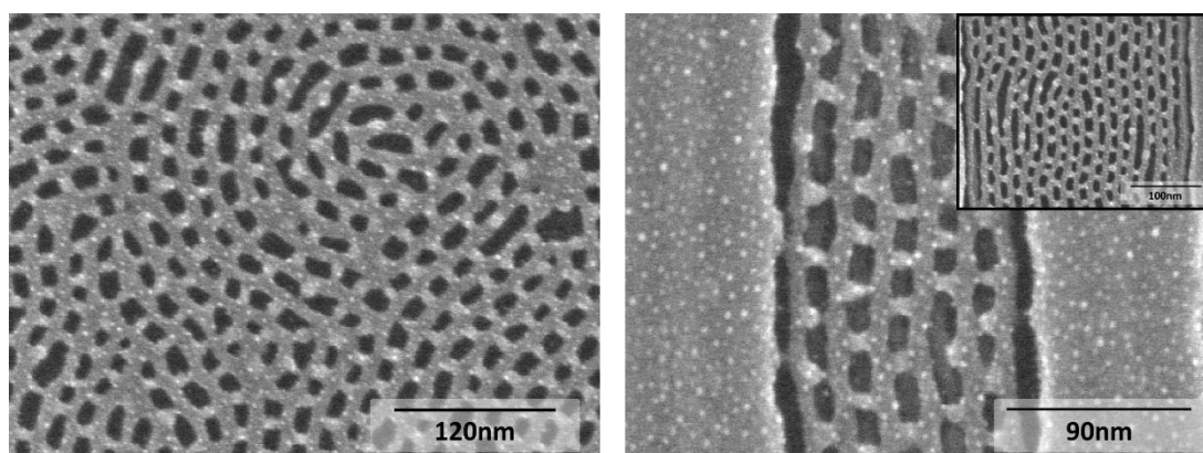
Figure 6-5: SEM top view images of SD16 after double patterning on (a) plane and (b) graphoepitaxy SiArc/SOC substrates
