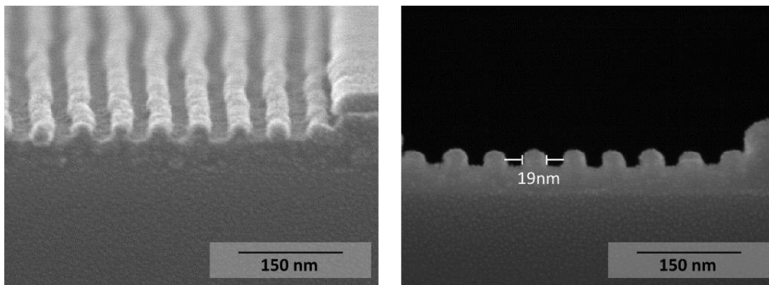
Figure 5-5: Cross section SEM images of SD45 lines after CF_4 and brief O_2 revealing etch step
