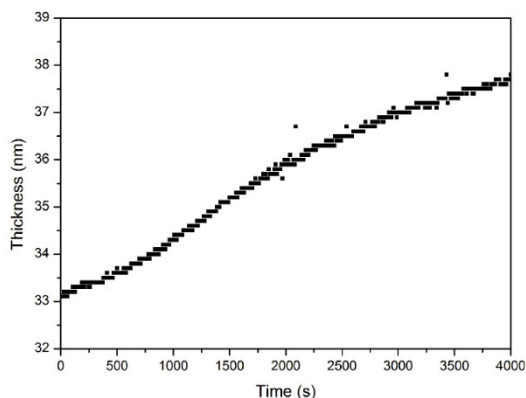
Figure 4-7 : Swelling rate of SOC substrate in solvent vapor
