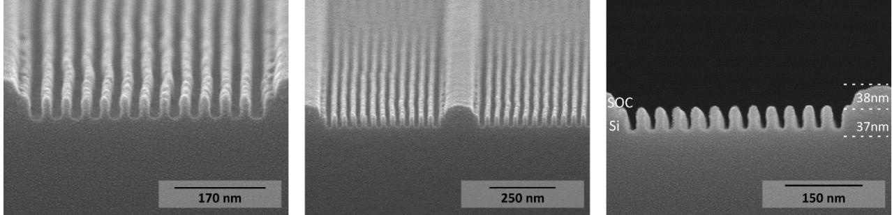
Figure 5-11: SEM cross section images of SD45 after 10s CW mode SF 6 /CHF 3 /Ar transfer etching
