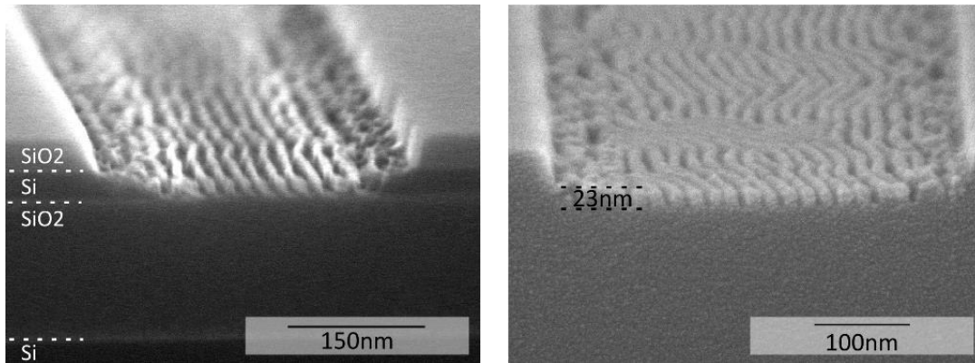
Figure 5-16: cross section SEM images of SD16 transferred into SOI substrate by HBr/He-O2 CW plasma
