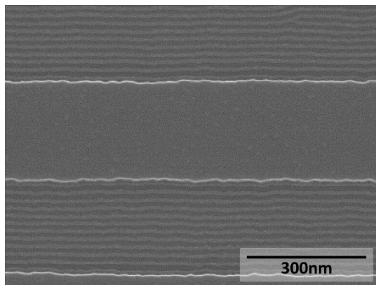
Figure 4-5 : SEM top view image of SD16 after 1min SVA in PGMEA followed by a TA of 15min at 150°C
