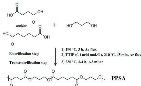
Scheme 2.2.1 : Reaction procedure for PPSA organometallic synthesis.
